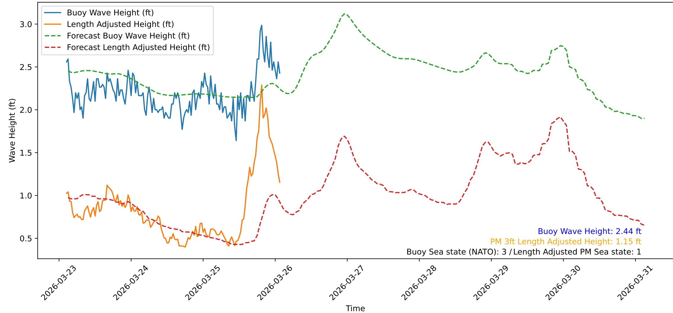
Wave Heights over Time for Green Beach at 2026-03-26 02:31:10
