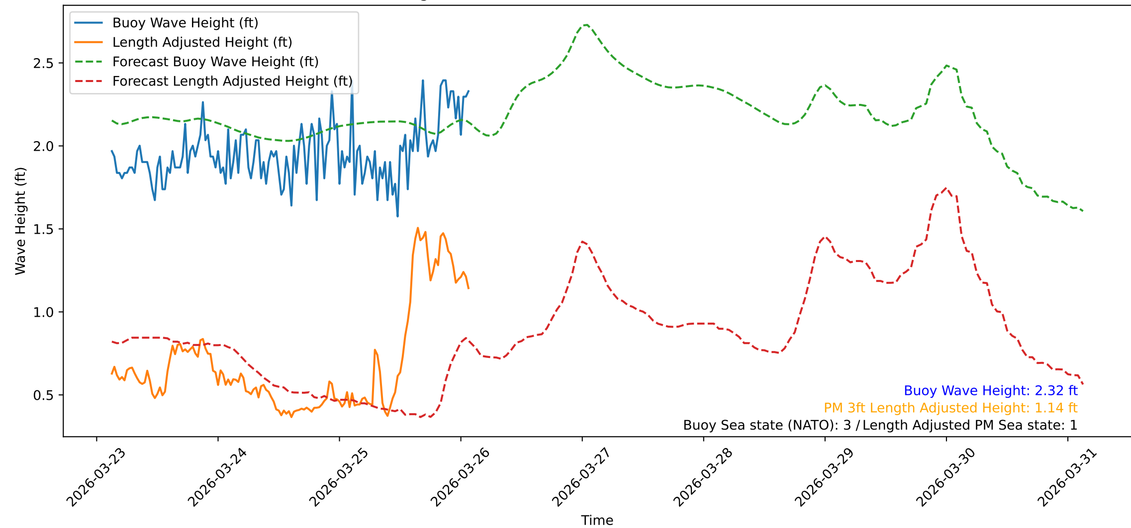
Wave Heights over Time for Red Beach at 2026-03-26 02:30:48
