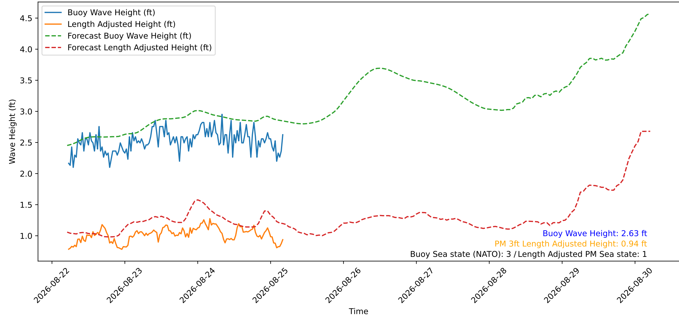
Wave Heights over Time for Red Beach at 2026-08-25 05:00:50
