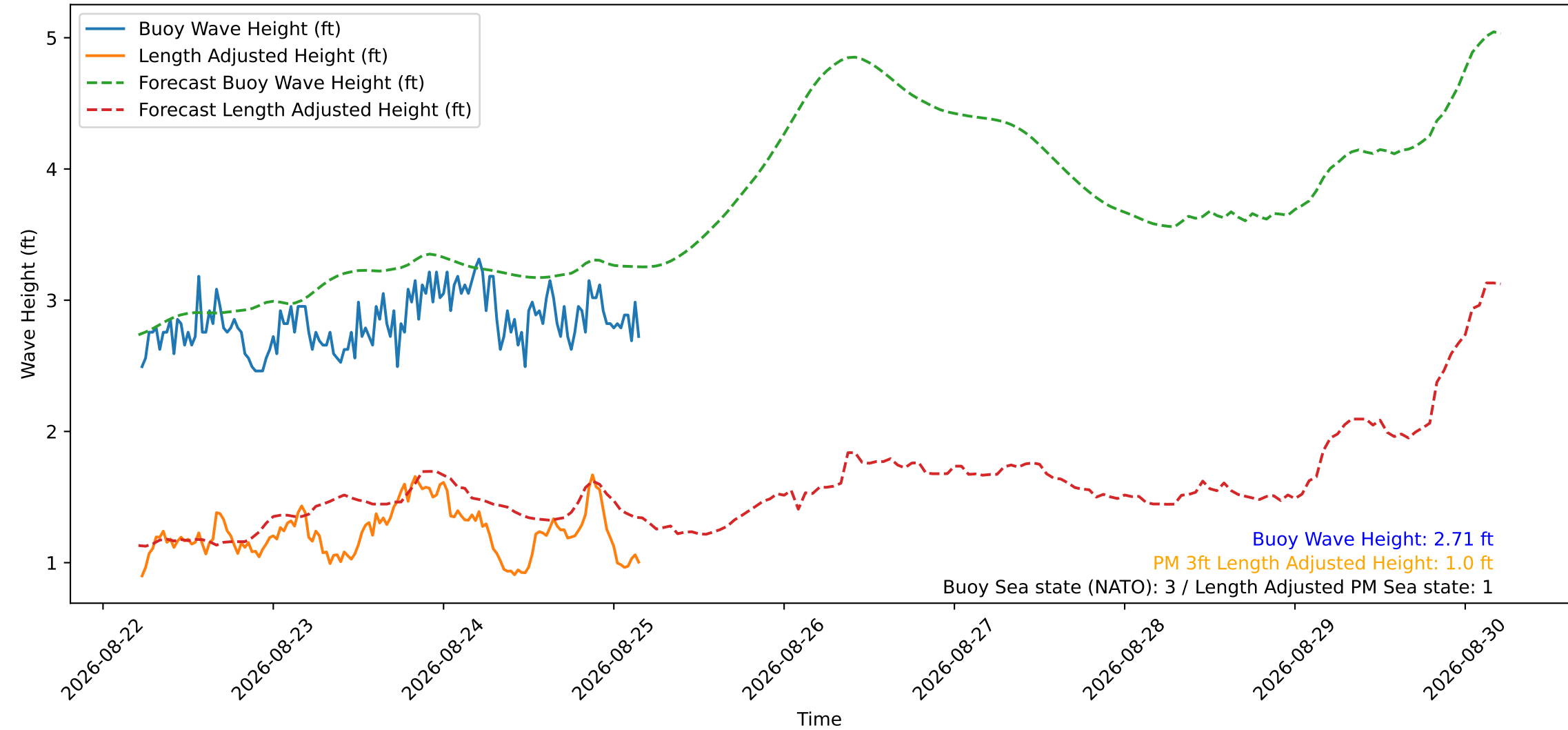
Wave Heights over Time for Green Beach at 2026-08-25 05:01:13
