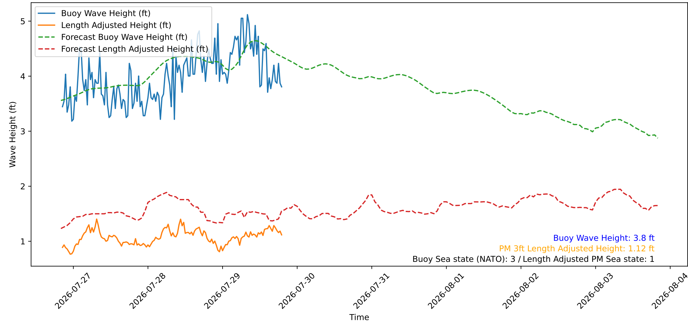
Wave Heights over Time for Red Beach at 2026-07-29 20:00:46
