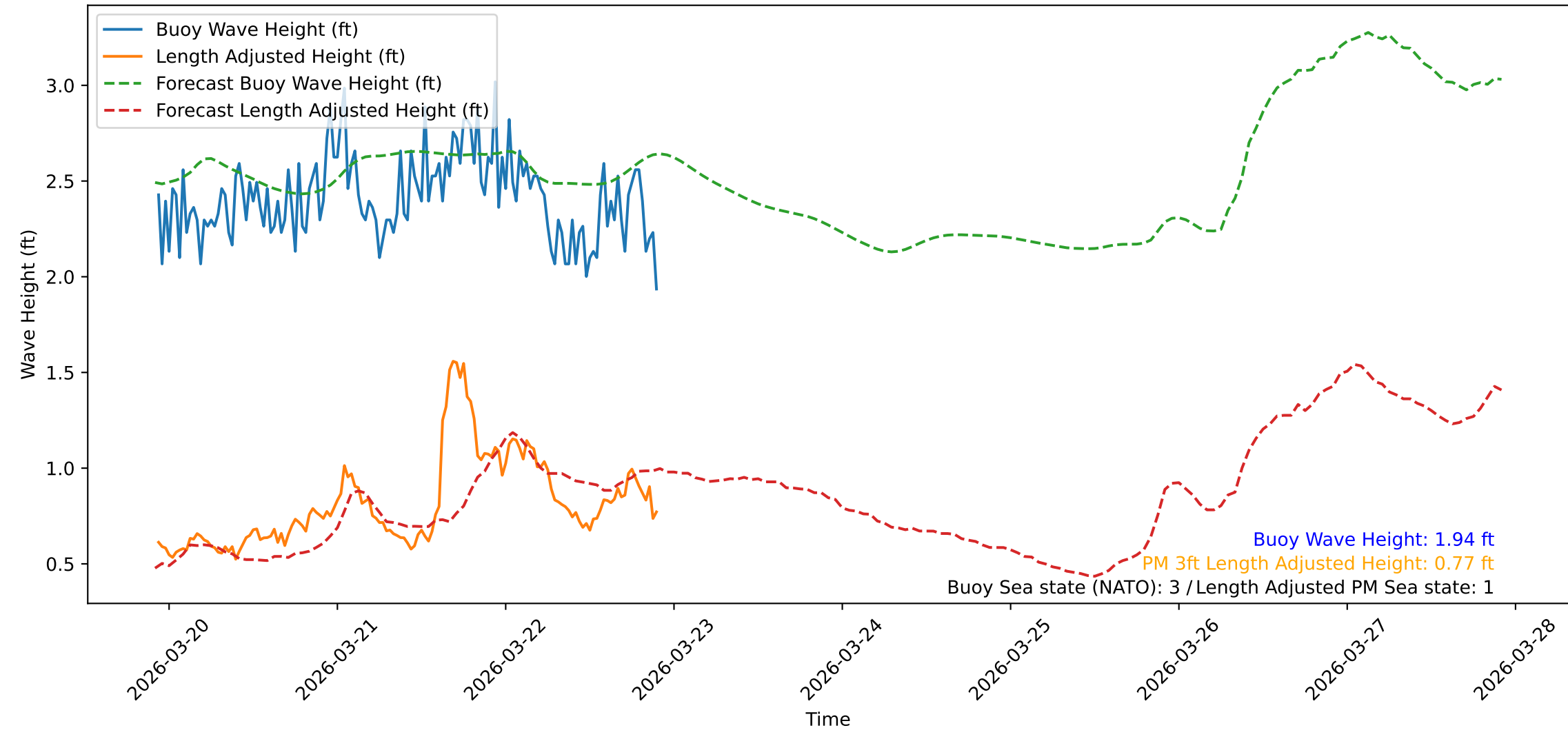
Wave Heights over Time for Oceanside Harbor at 2026-03-22 22:20:31
