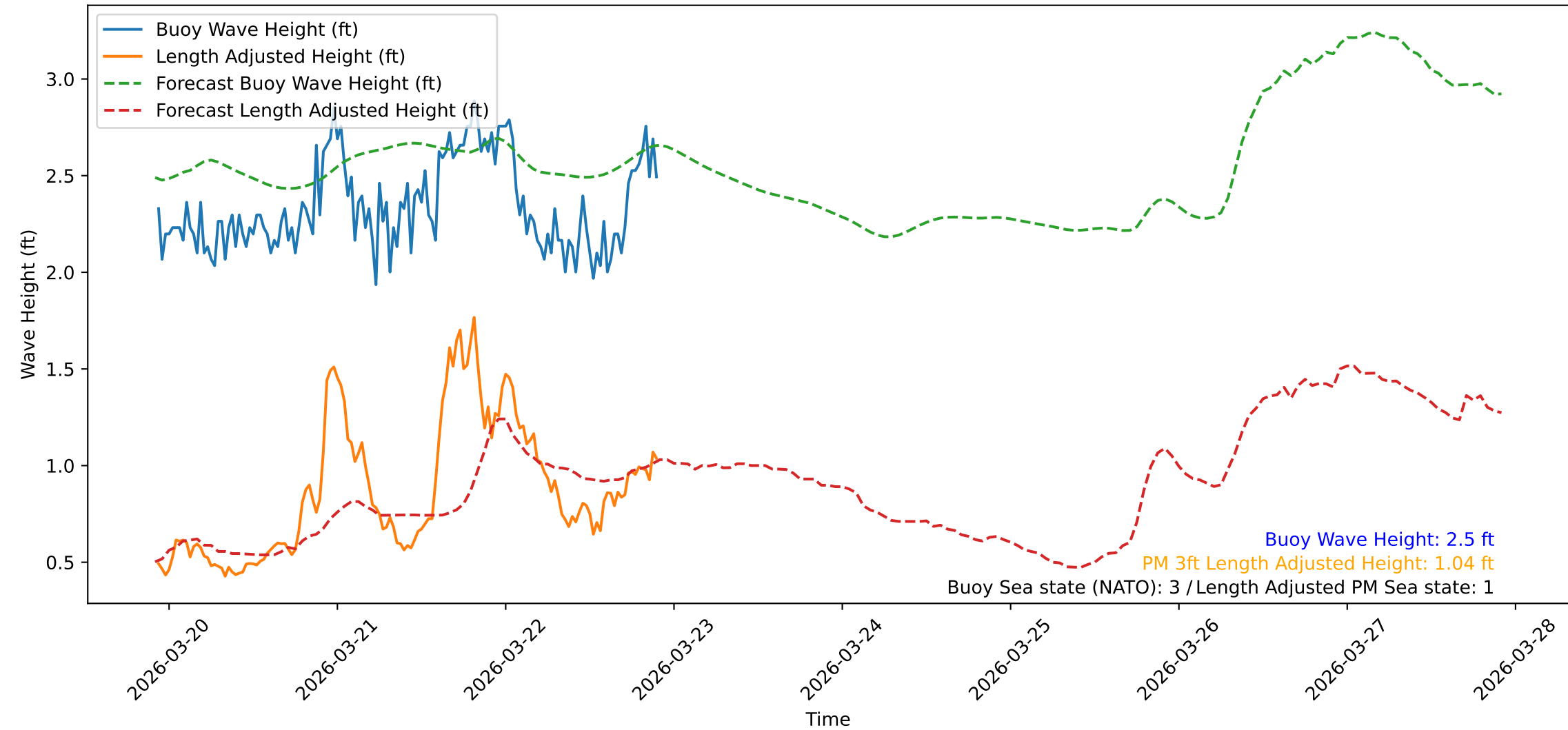
Wave Heights over Time for Green Beach at 2026-03-22 22:21:09
