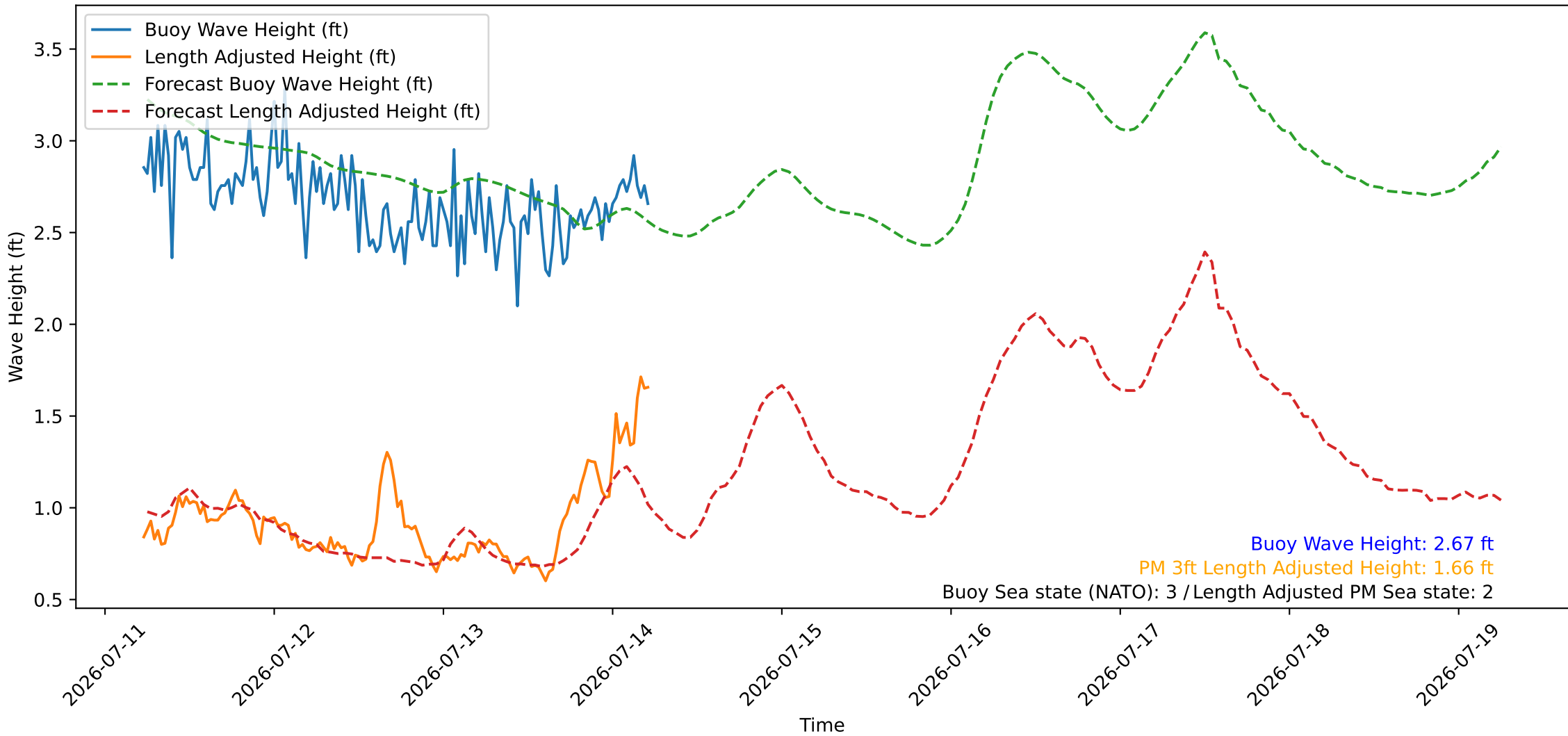
Wave Heights over Time for Oceanside Harbor at 2026-07-14 05:40:27
