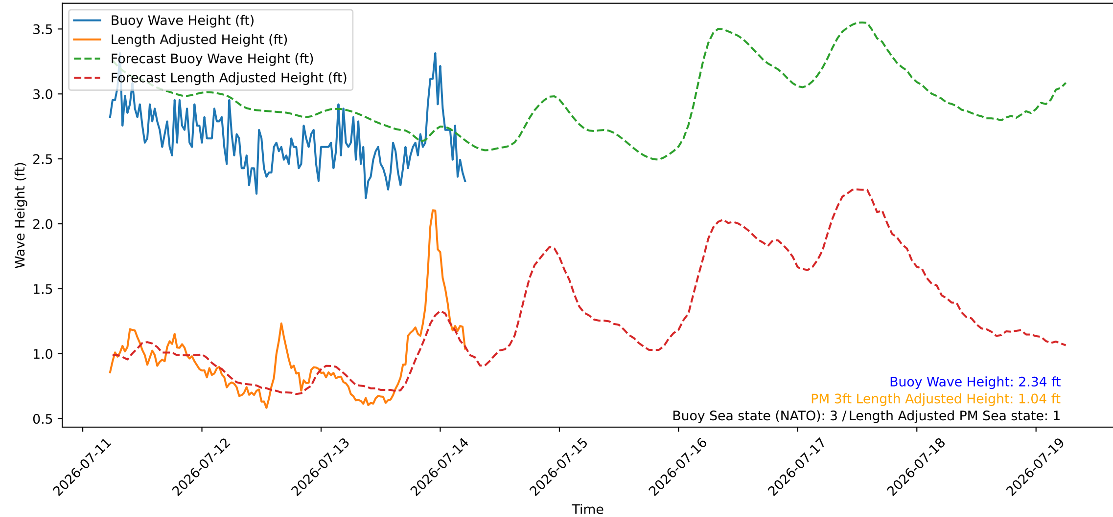
Wave Heights over Time for Green Beach at 2026-07-14 05:41:09
