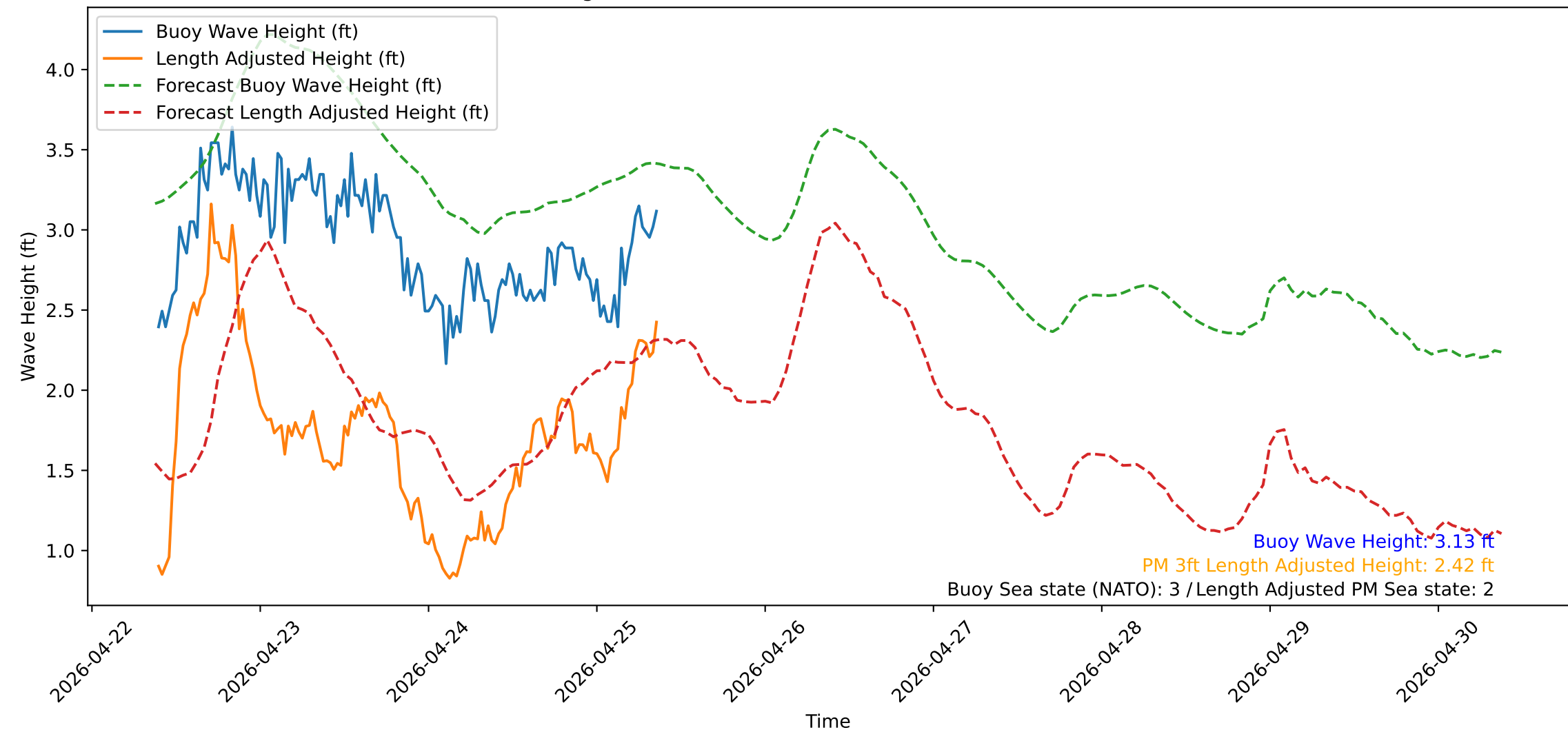
Wave Heights over Time for Red Beach at 2026-04-25 09:20:52
