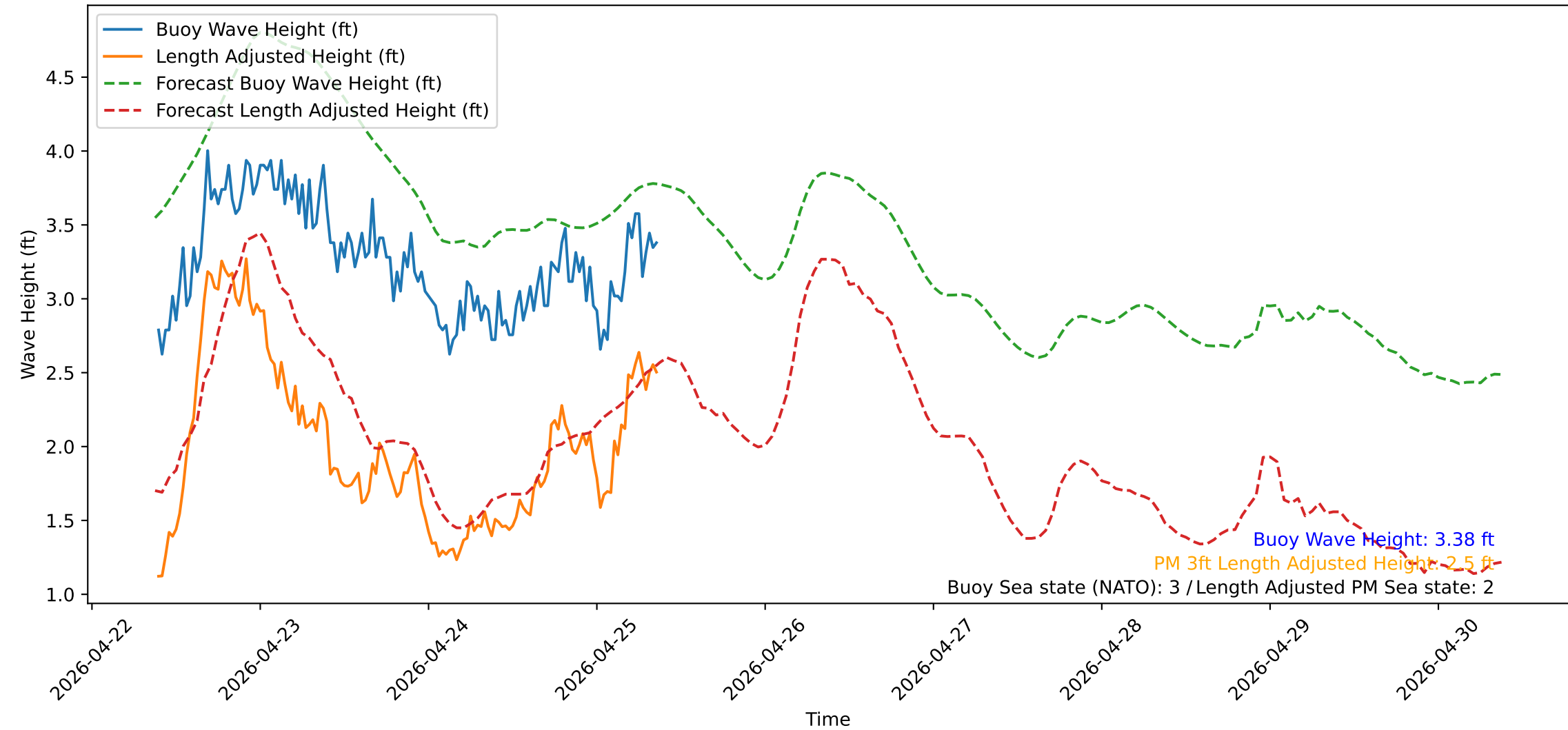
Wave Heights over Time for Green Beach at 2026-04-25 09:21:14
