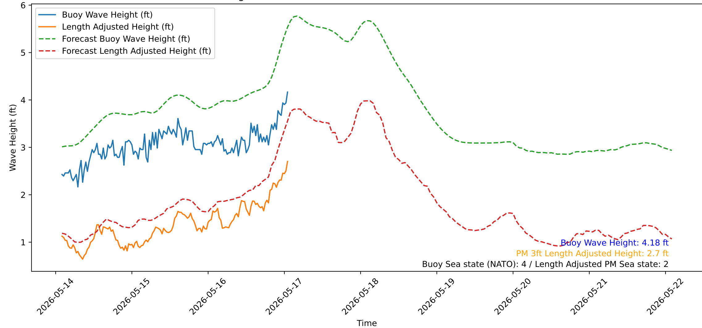
Wave Heights over Time for Oceanside Harbor at 2026-05-17 01:50:31
