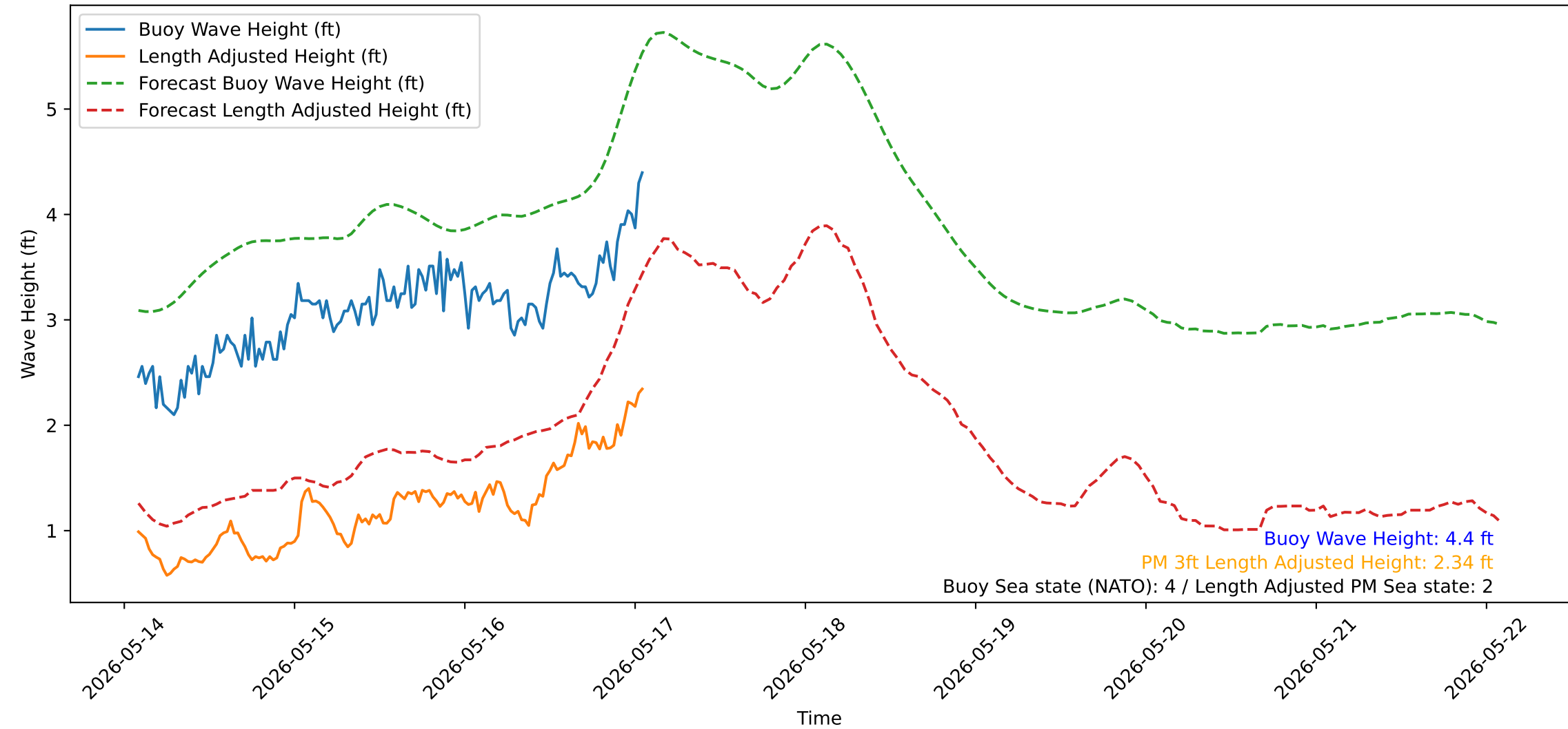
Wave Heights over Time for Green Beach at 2026-05-17 01:51:14
