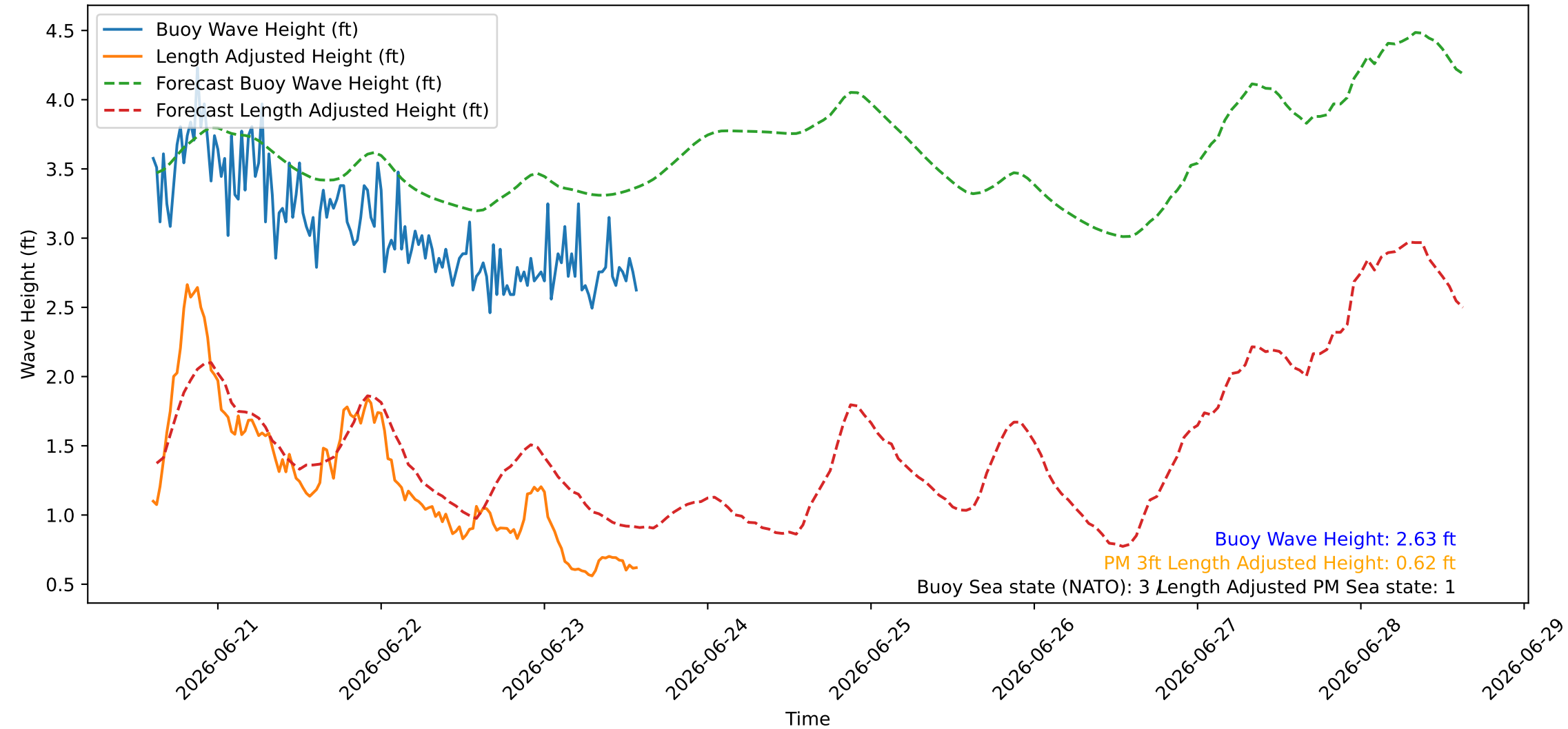
Wave Heights over Time for Green Beach at 2026-06-23 14:31:08
