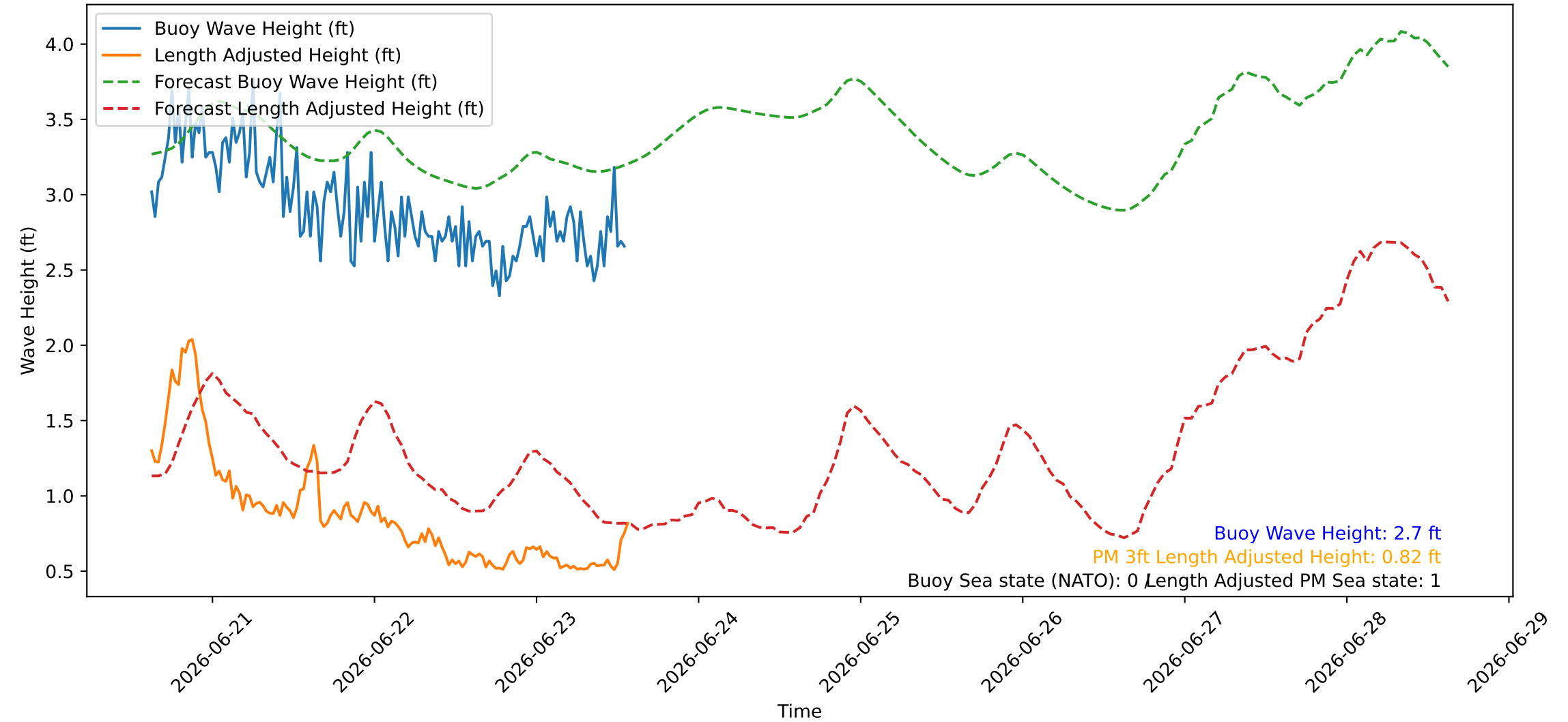
Wave Heights over Time for Red Beach at 2026-06-23 14:30:45
