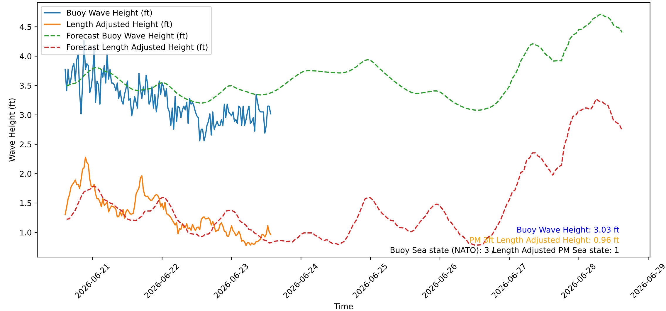
Wave Heights over Time for Oceanside Harbor at 2026-06-23 14:30:26
