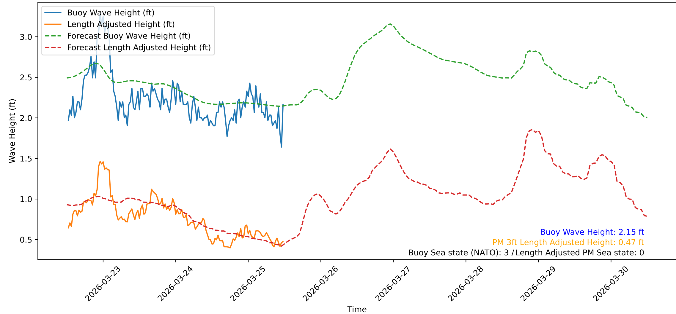
Wave Heights over Time for Green Beach at 2026-03-25 12:21:09
