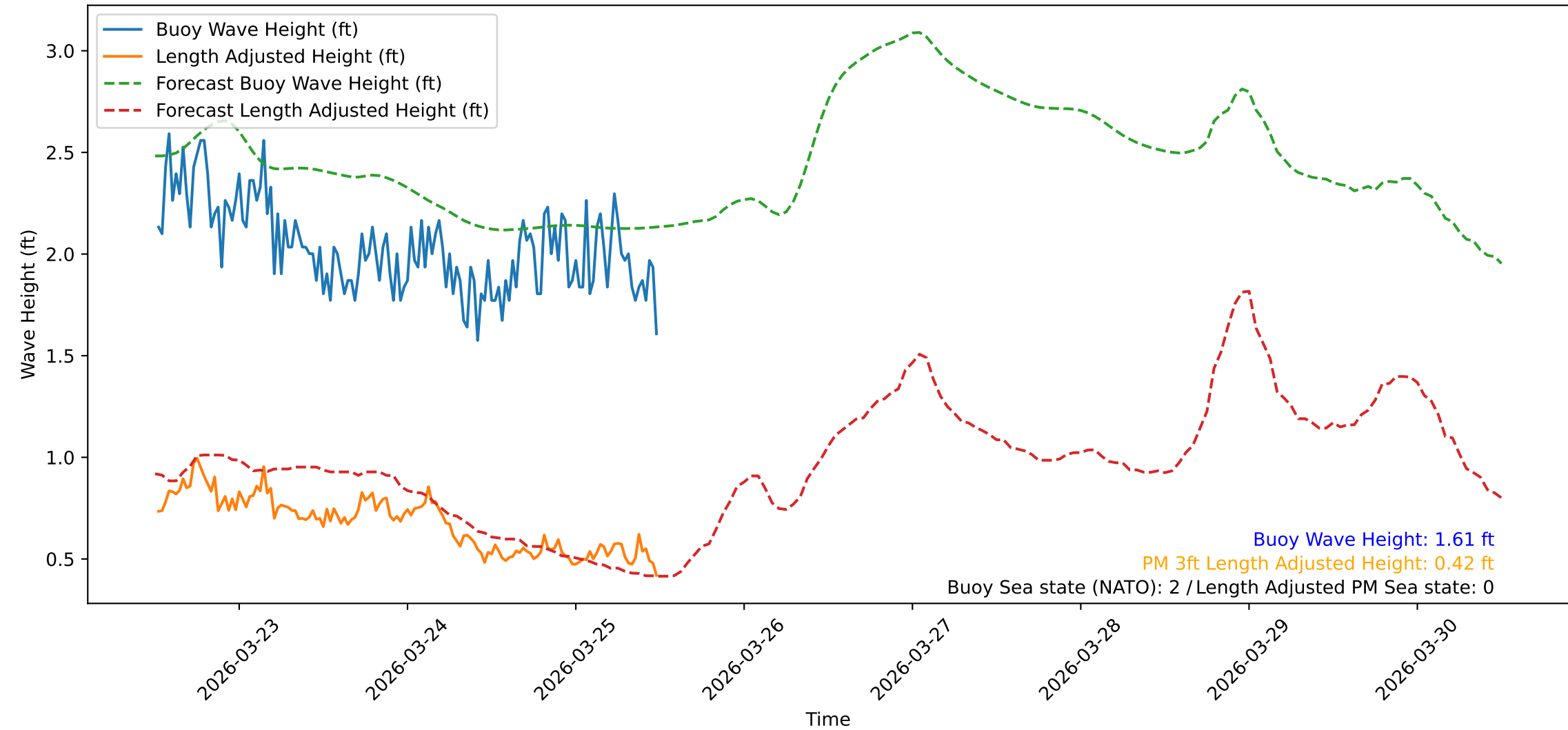
Wave Heights over Time for Oceanside Harbor at 2026-03-25 12:20:31
