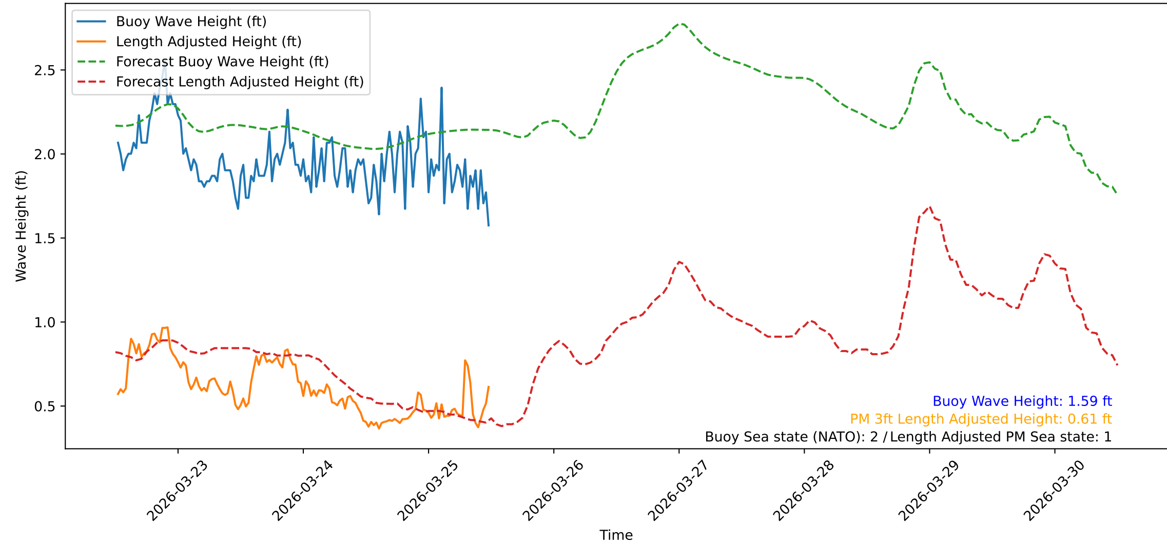
Wave Heights over Time for Red Beach at 2026-03-25 12:20:47
