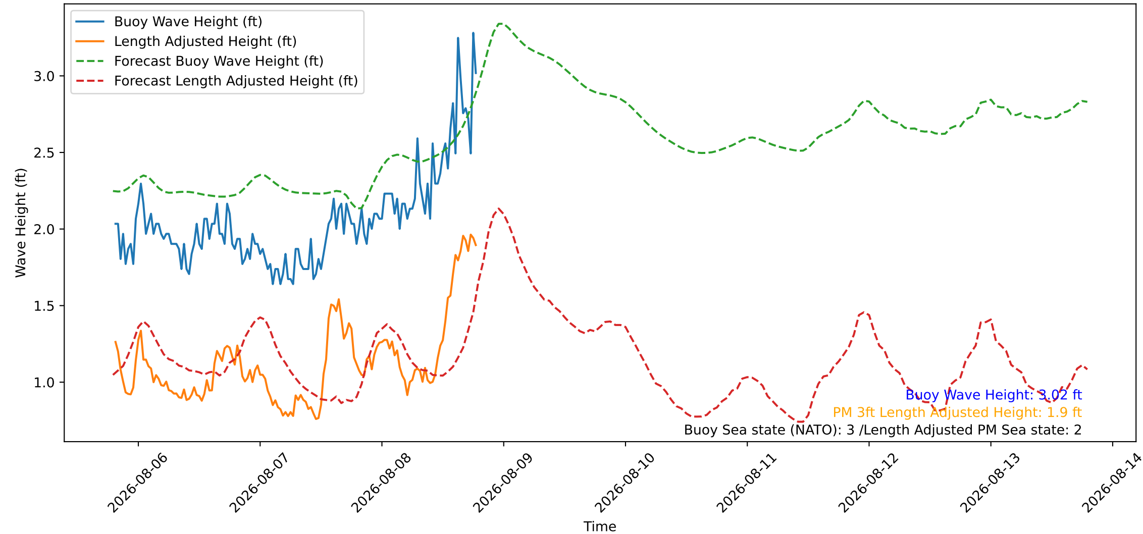
Wave Heights over Time for Oceanside Harbor at 2026-08-08 19:20:26
