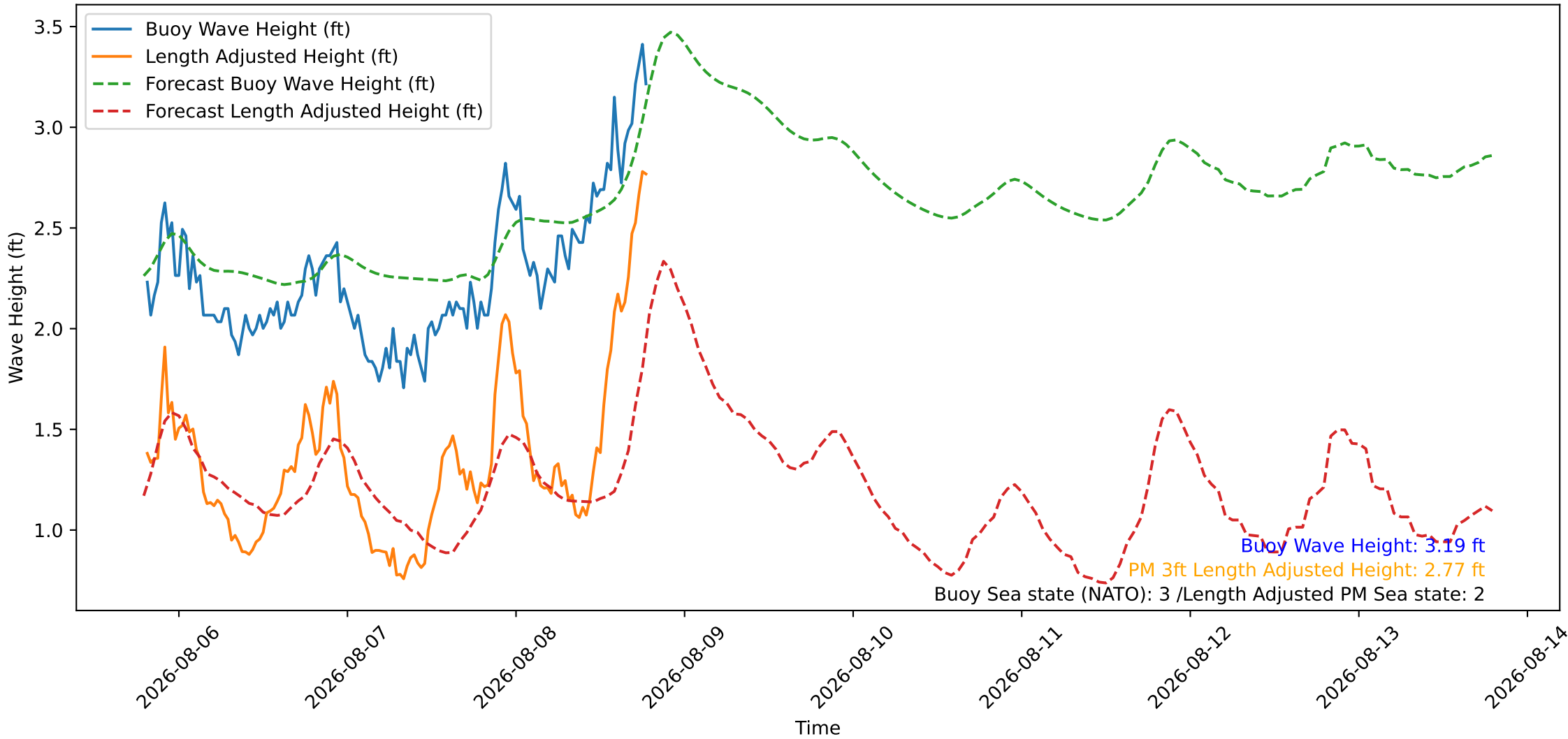
Wave Heights over Time for Green Beach at 2026-08-08 19:21:11
