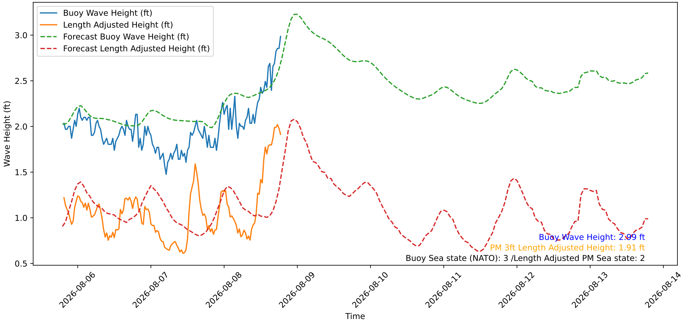
Wave Heights over Time for Red Beach at 2026-08-08 19:20:48
