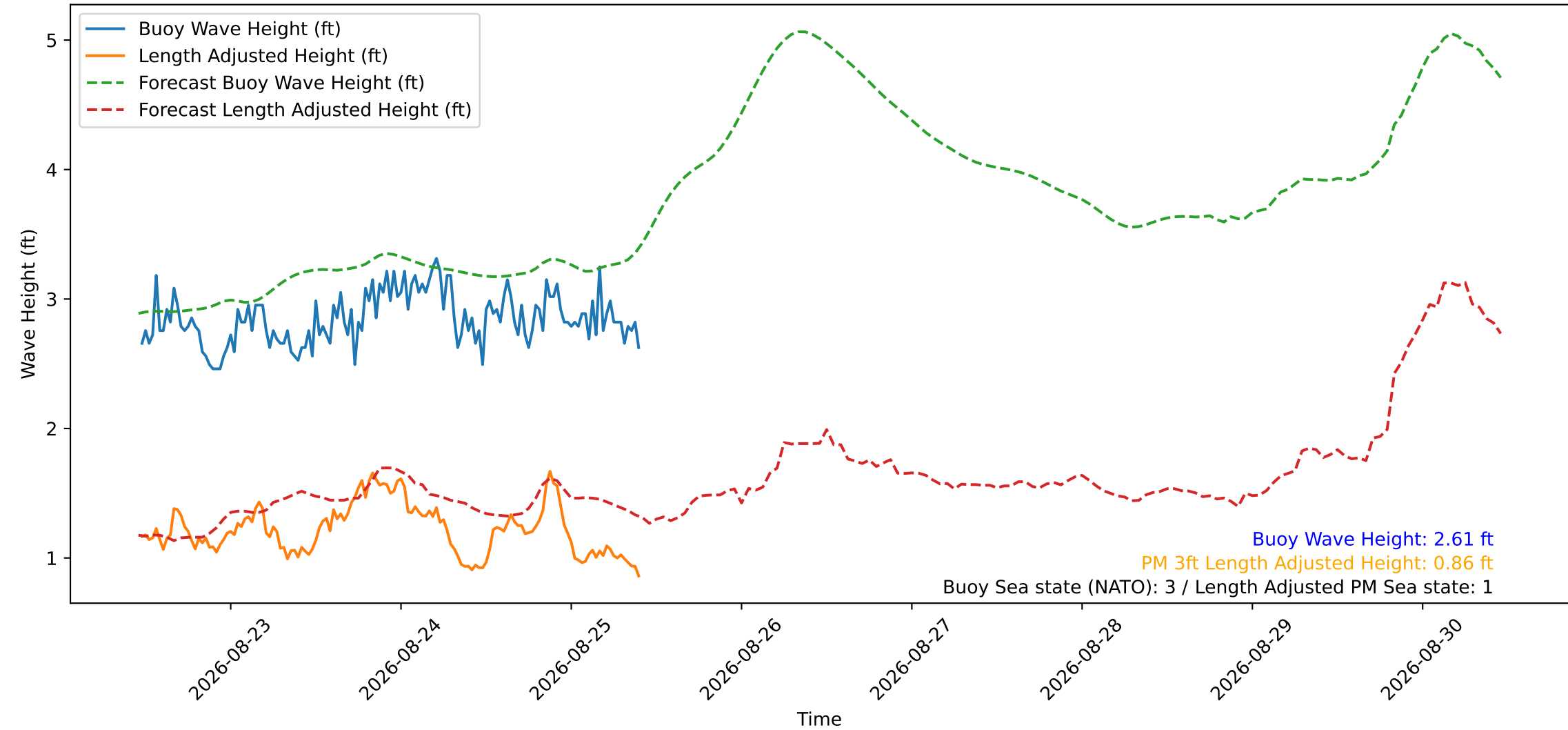
Wave Heights over Time for Green Beach at 2026-08-25 11:01:12
