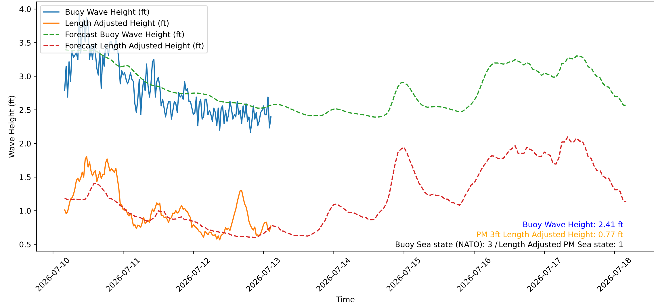
Wave Heights over Time for Red Beach at 2026-07-13 03:30:45
