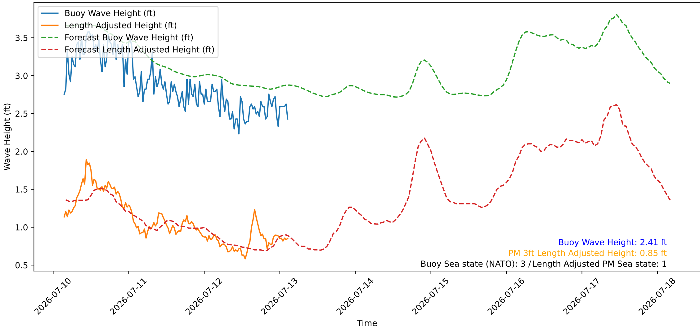
Wave Heights over Time for Green Beach at 2026-07-13 03:31:08
