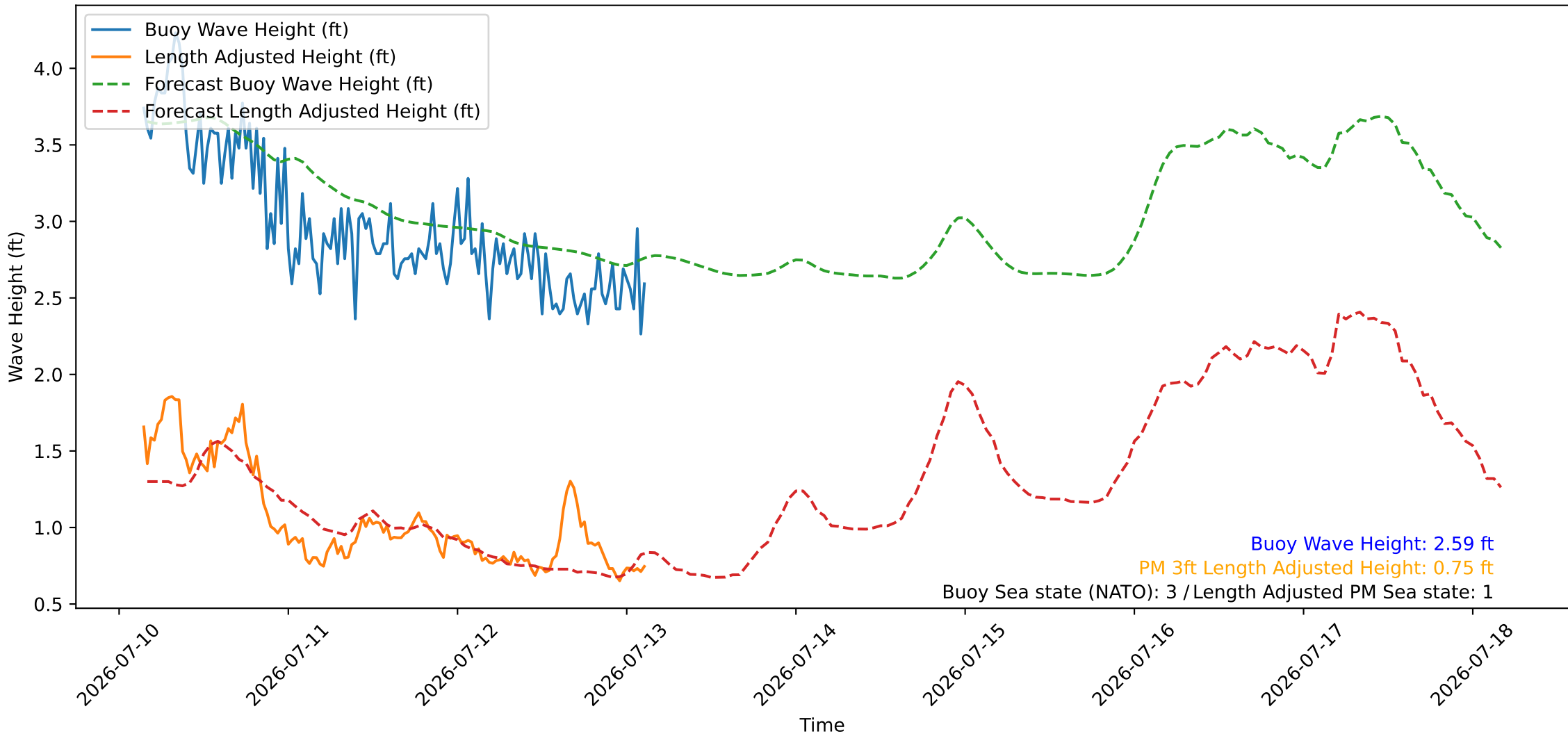
Wave Heights over Time for Oceanside Harbor at 2026-07-13 03:30:26
