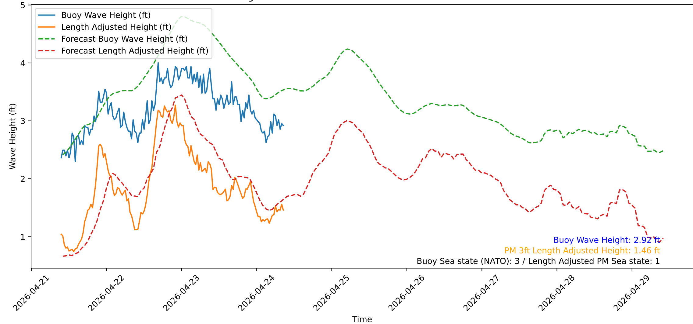
Wave Heights over Time for Green Beach at 2026-04-24 09:31:13
