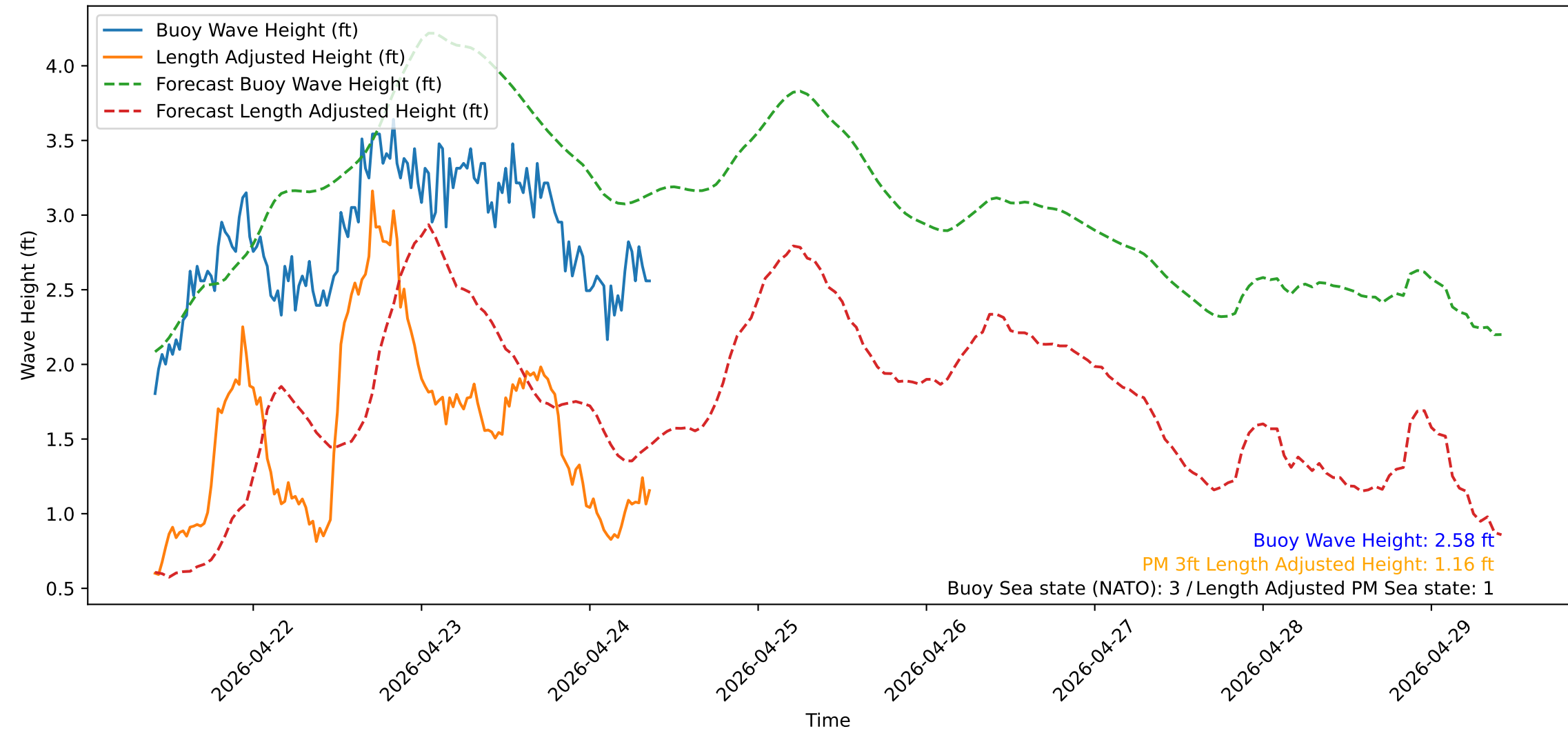
Wave Heights over Time for Red Beach at 2026-04-24 09:30:51
