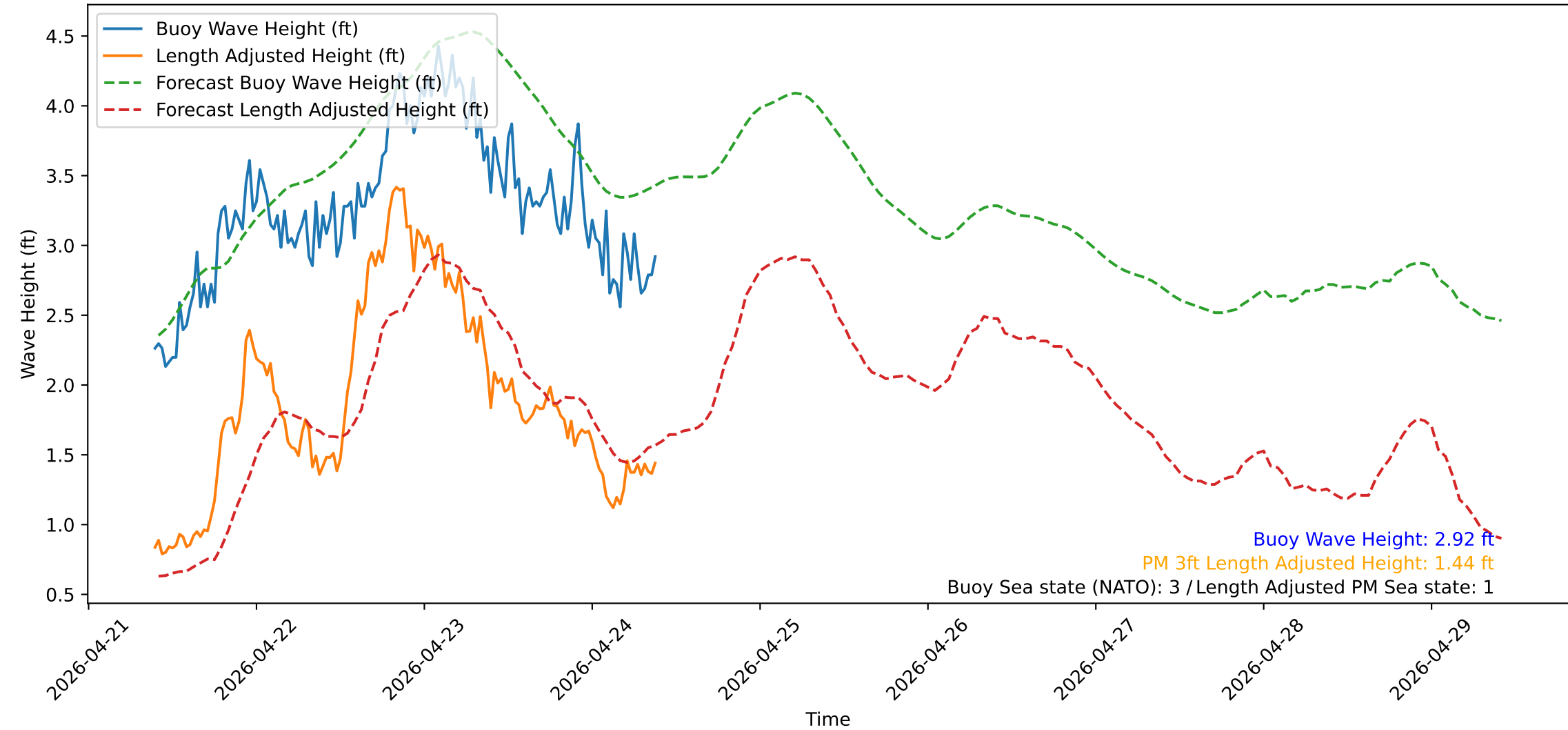
Wave Heights over Time for Oceanside Harbor at 2026-04-24 09:30:32
