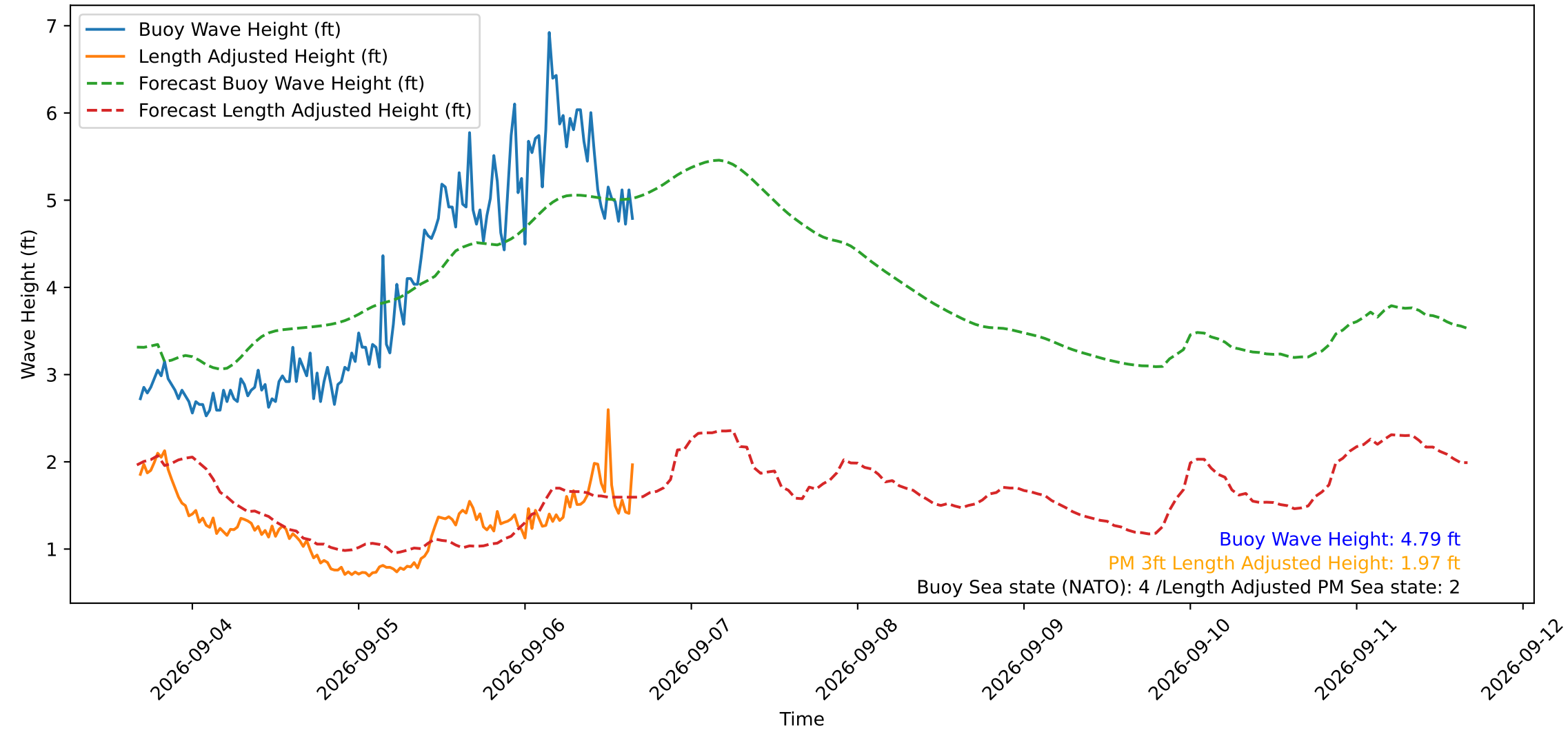
Wave Heights over Time for Red Beach at 2026-09-06 16:20:51
