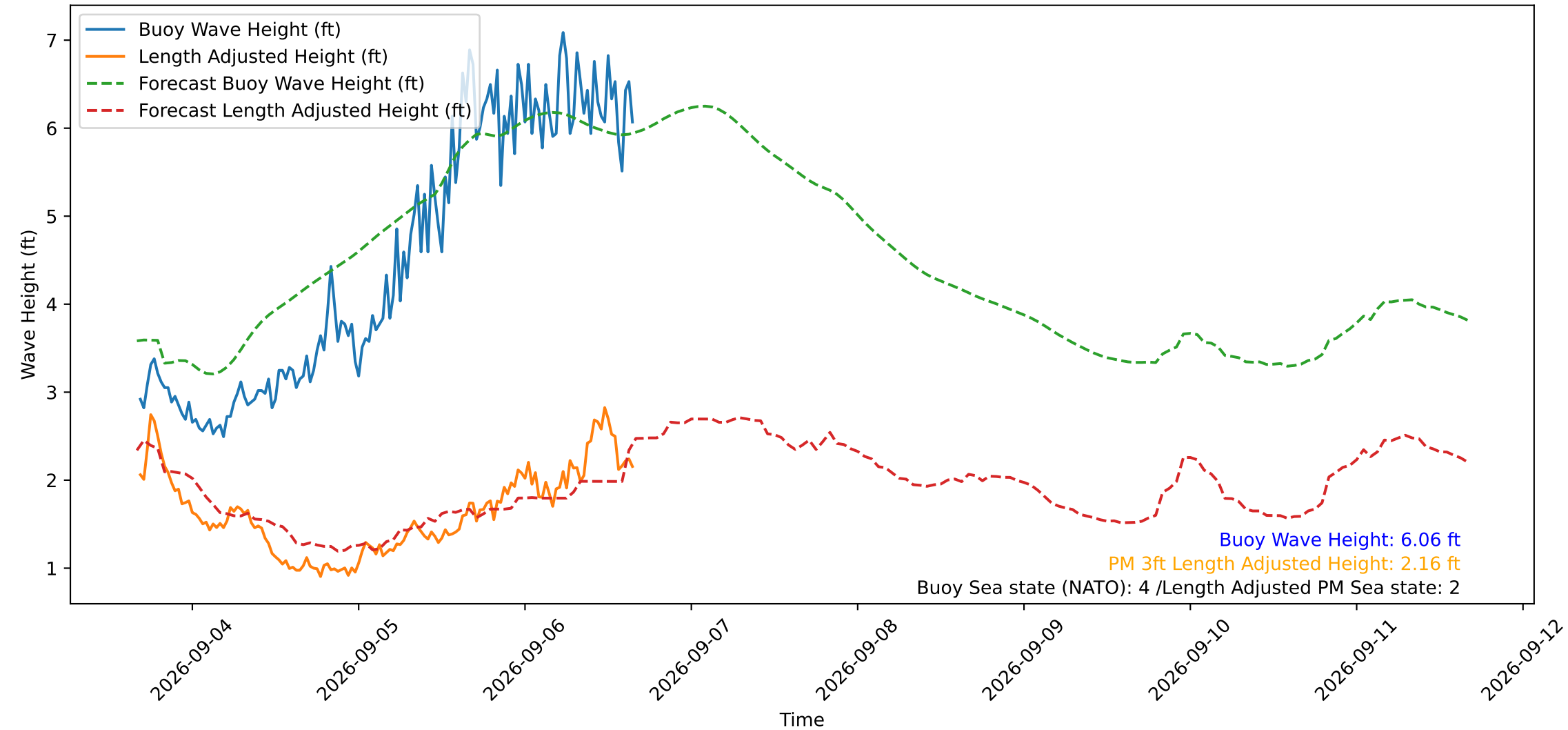
Wave Heights over Time for Green Beach at 2026-09-06 16:21:14
