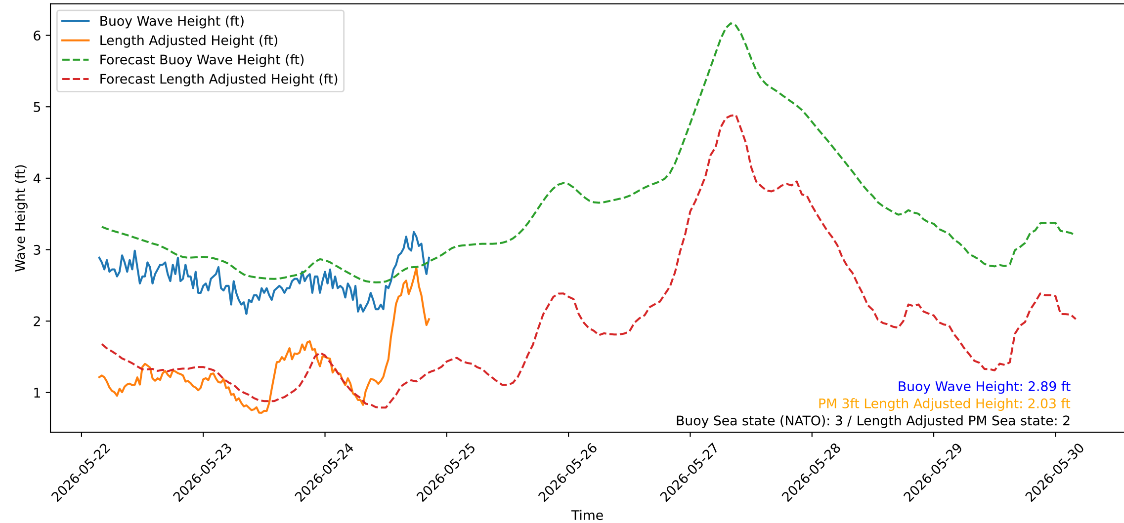
Wave Heights over Time for Oceanside Harbor at 2026-05-25 03:30:31
