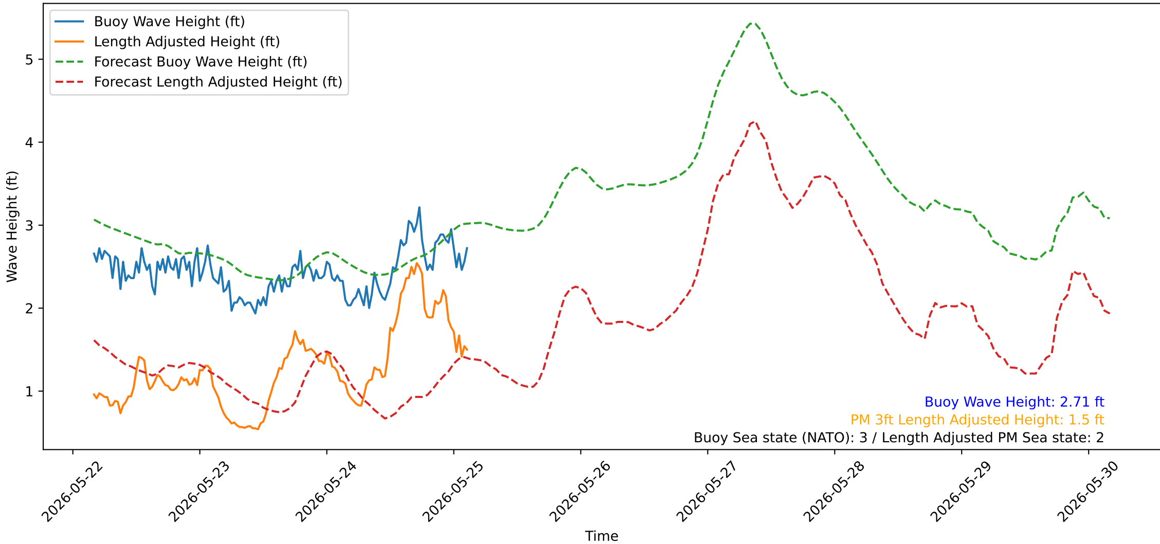
Wave Heights over Time for Red Beach at 2026-05-25 03:30:50
