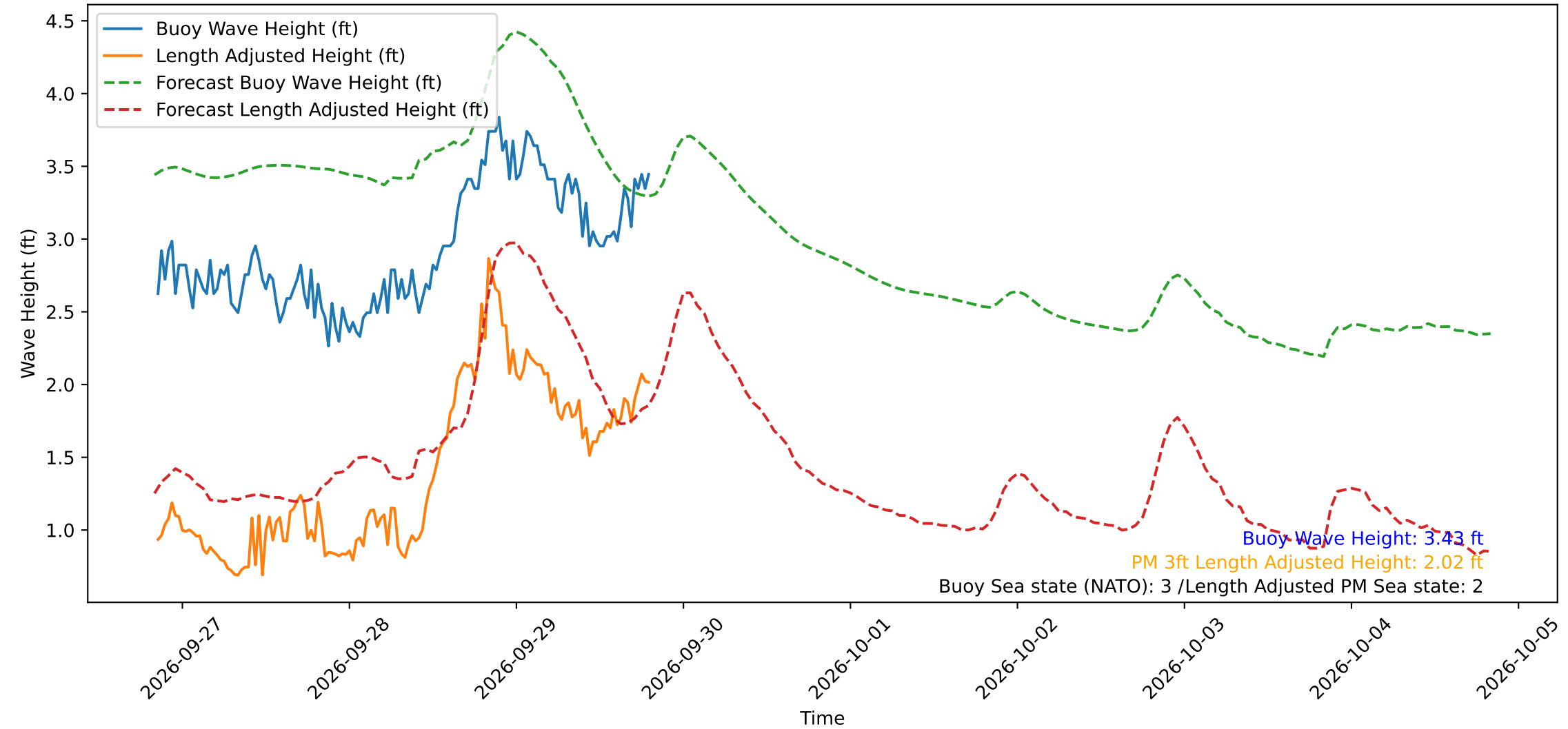
Wave Heights over Time for Red Beach at 2026-09-29 20:00:49
