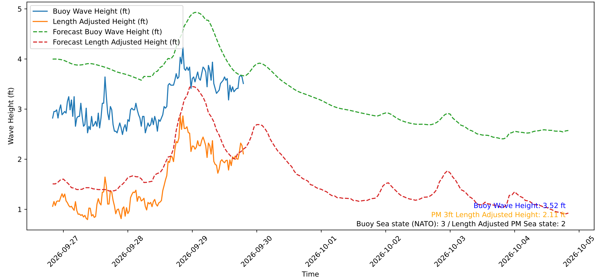
Wave Heights over Time for Oceanside Harbor at 2026-09-29 20:00:30
