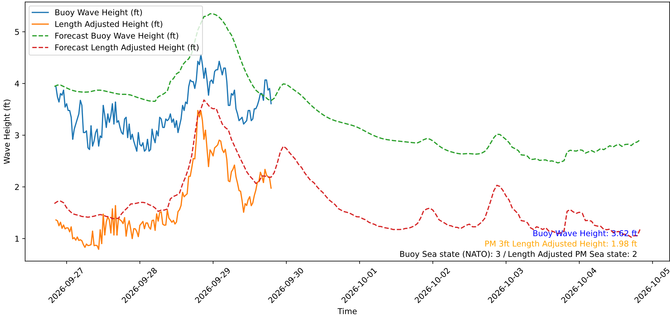
Wave Heights over Time for Green Beach at 2026-09-29 20:01:12
