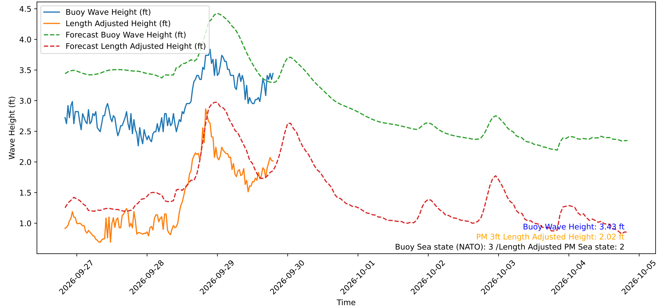
Wave Heights over Time for Red Beach at 2026-09-29 19:50:51
