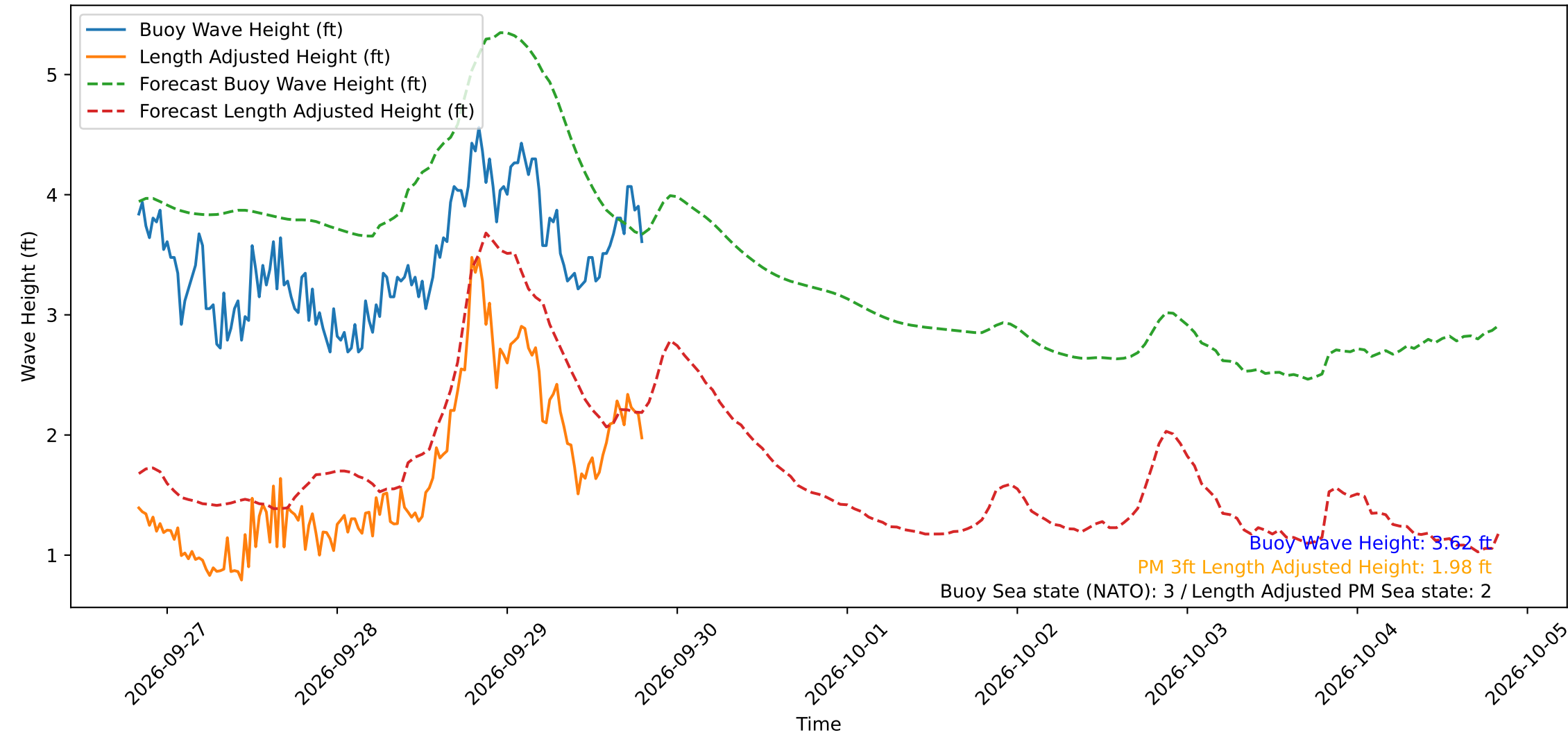
Wave Heights over Time for Green Beach at 2026-09-29 19:51:15
