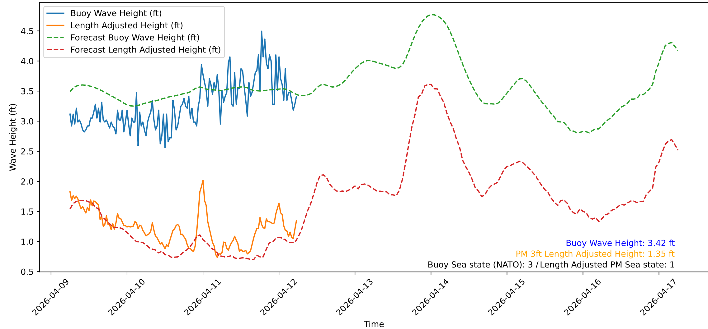
Wave Heights over Time for Green Beach at 2026-04-12 06:11:13
