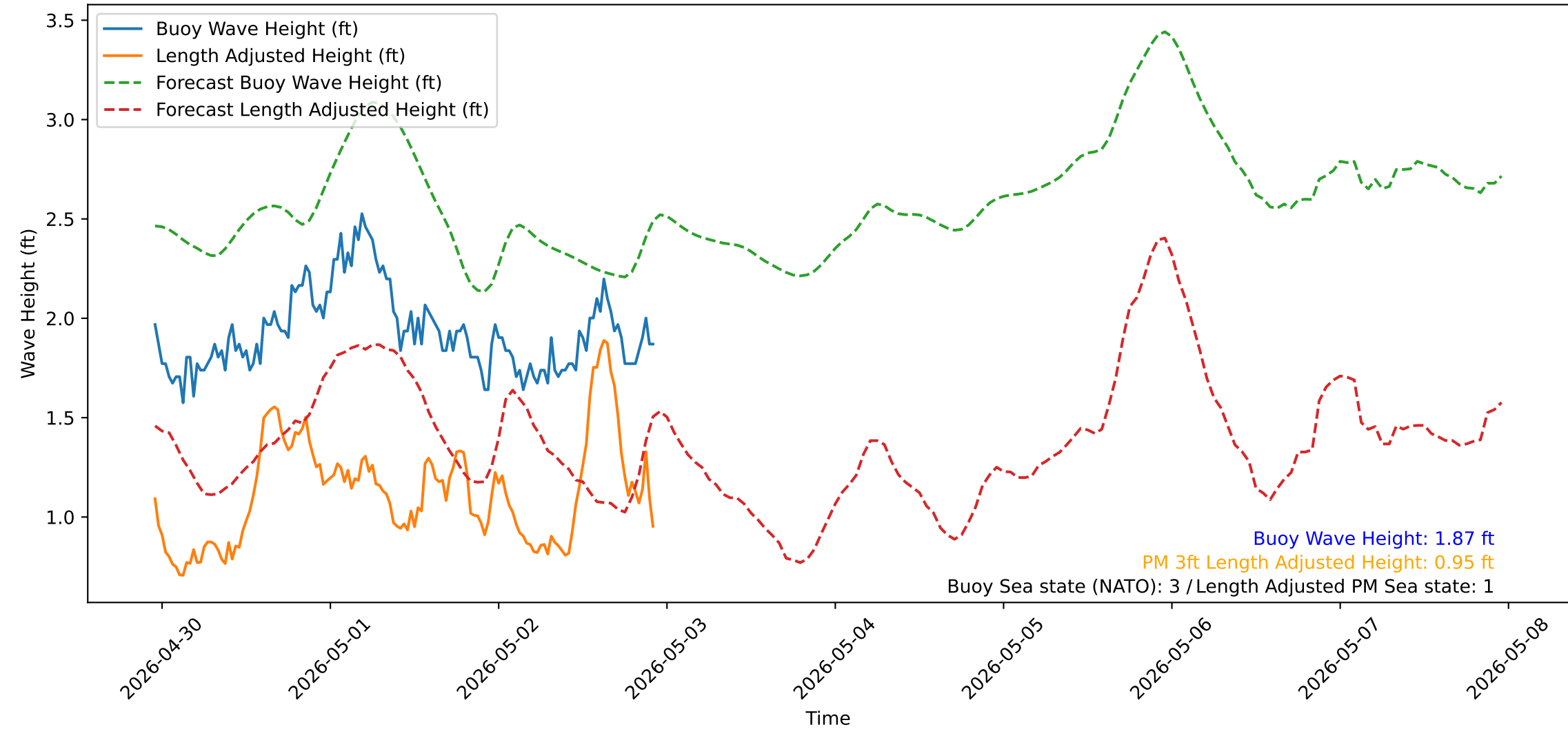
Wave Heights over Time for Red Beach at 2026-05-02 22:50:52
