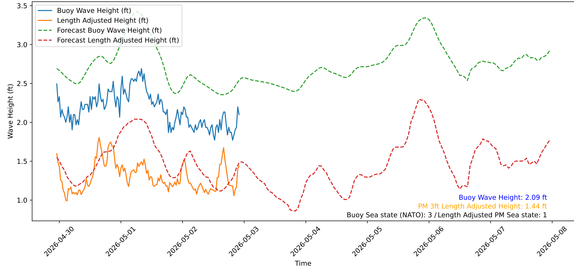
Wave Heights over Time for Oceanside Harbor at 2026-05-02 22:50:32
