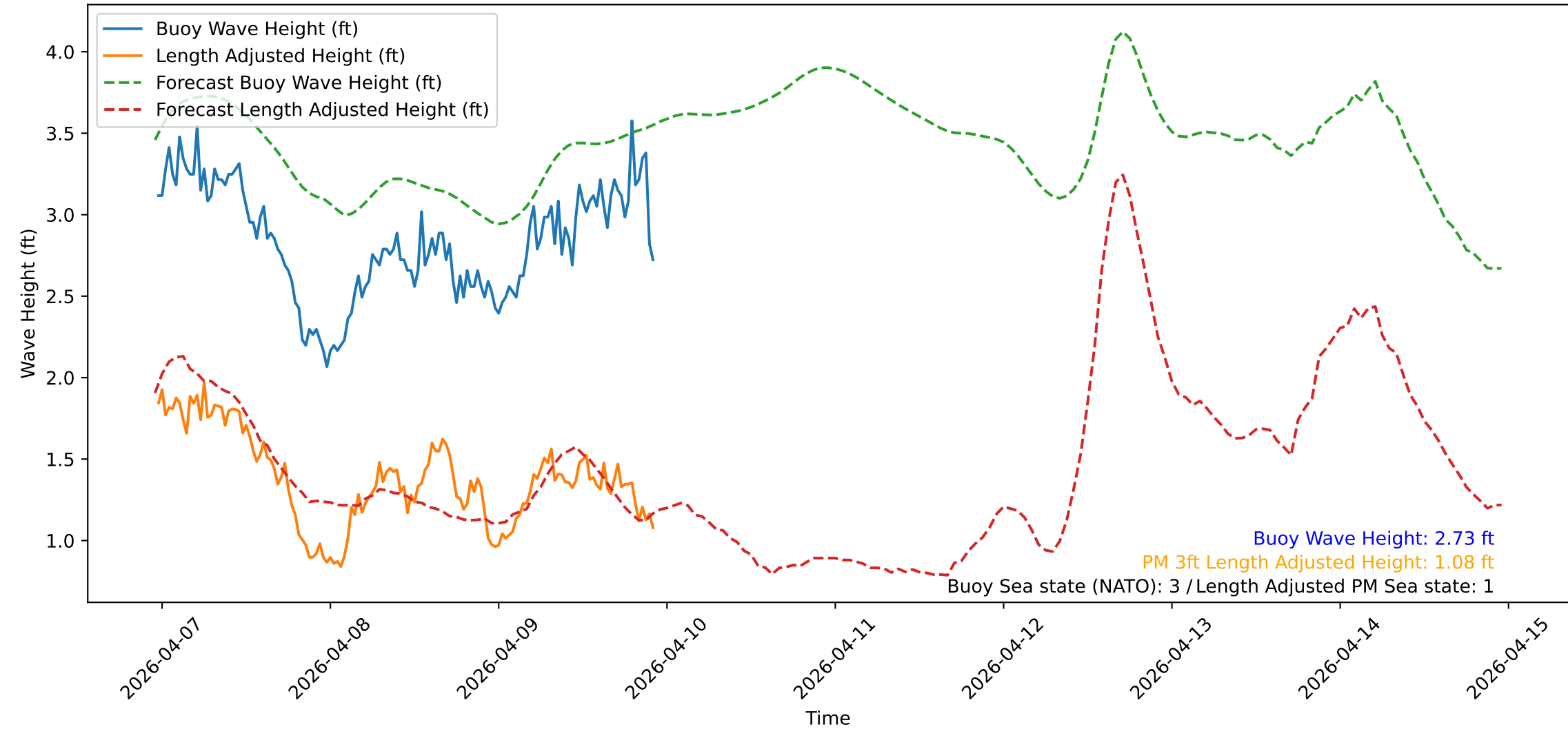
Wave Heights over Time for Red Beach at 2026-04-09 23:00:46
