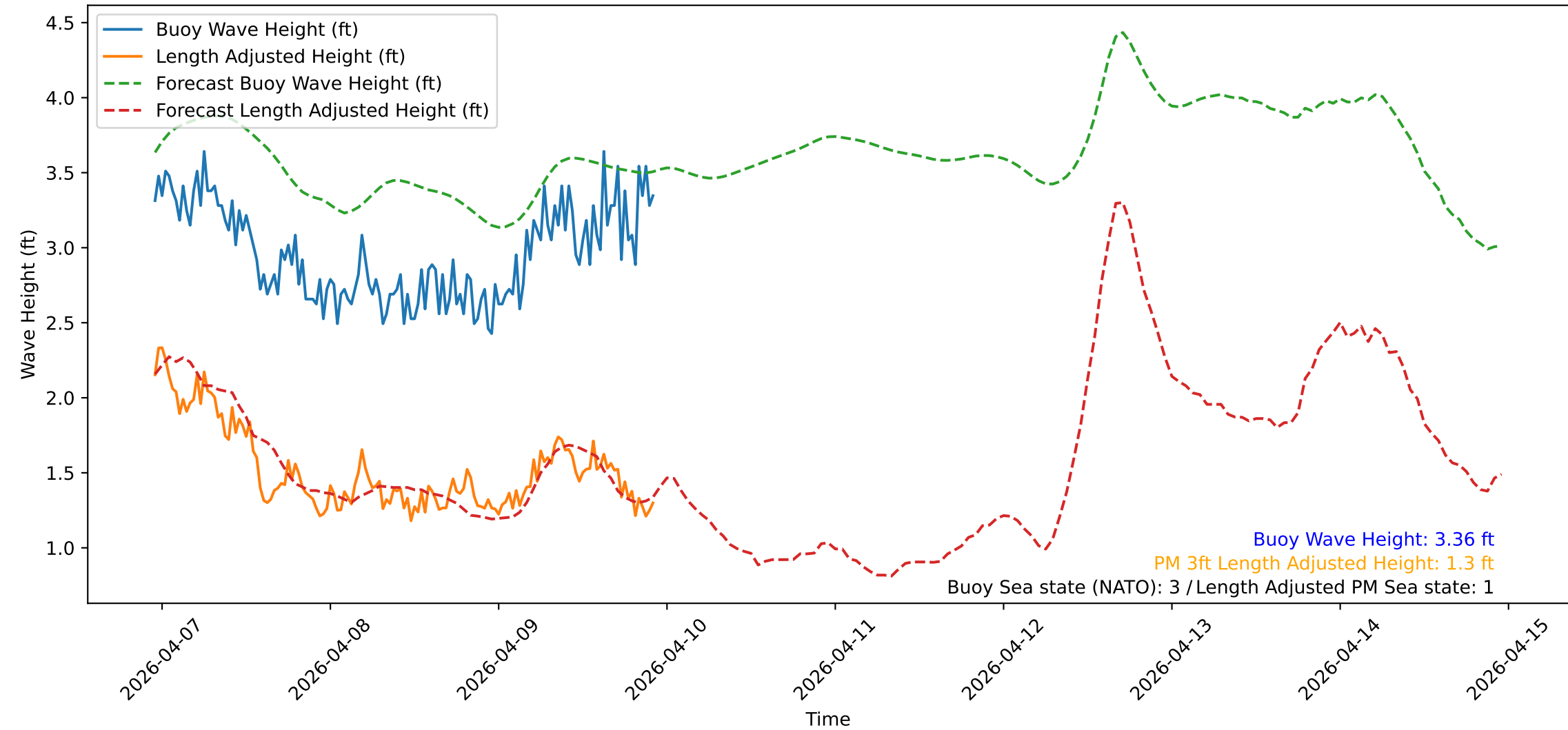
Wave Heights over Time for Oceanside Harbor at 2026-04-09 23:00:30
