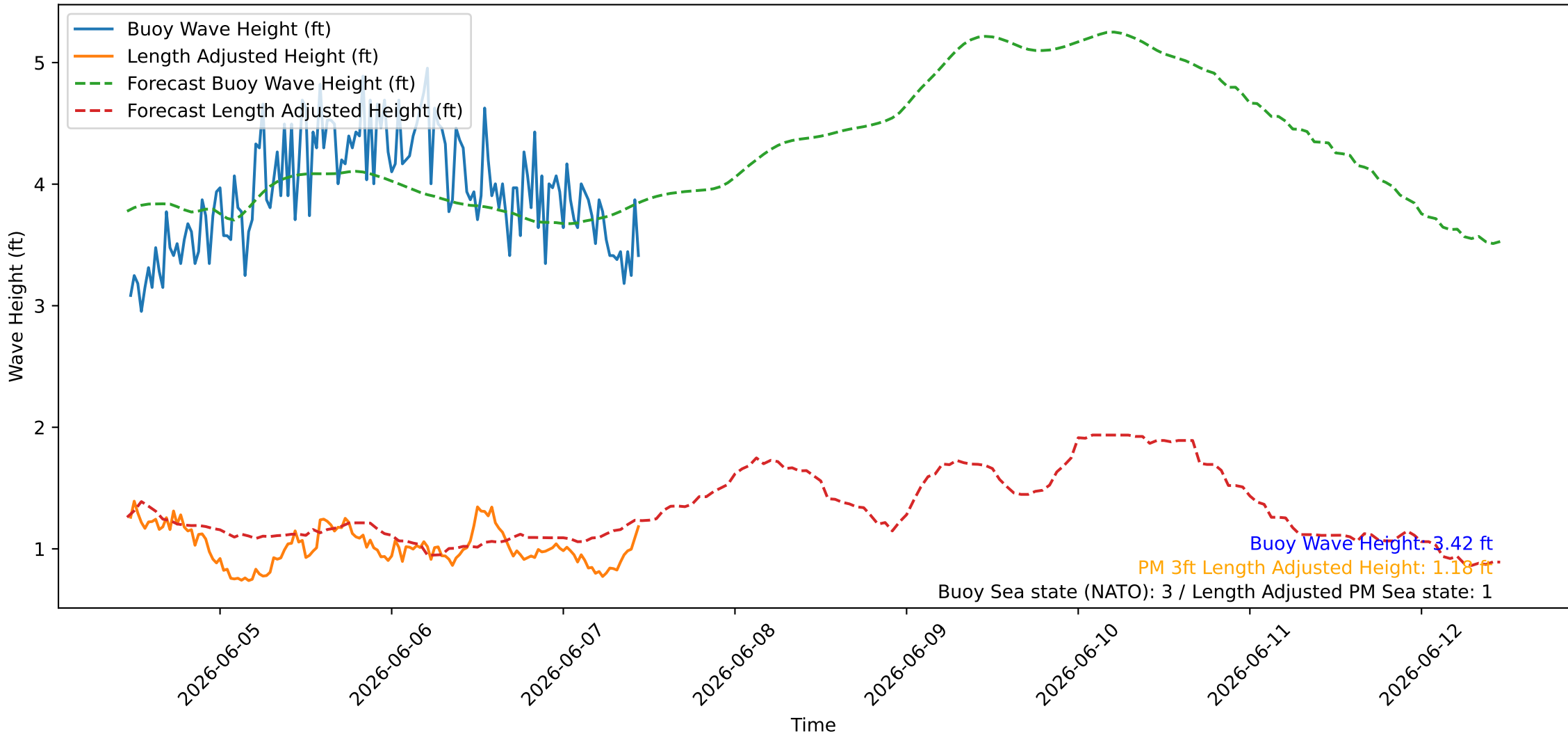
Wave Heights over Time for Red Beach at 2026-06-07 11:10:45
