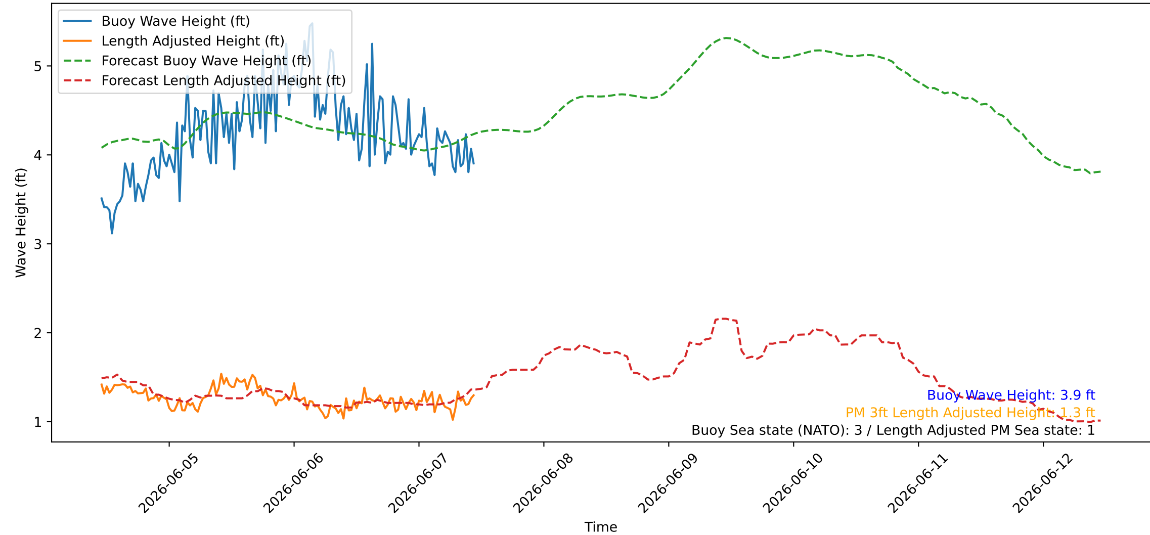
Wave Heights over Time for Oceanside Harbor at 2026-06-07 11:10:26
