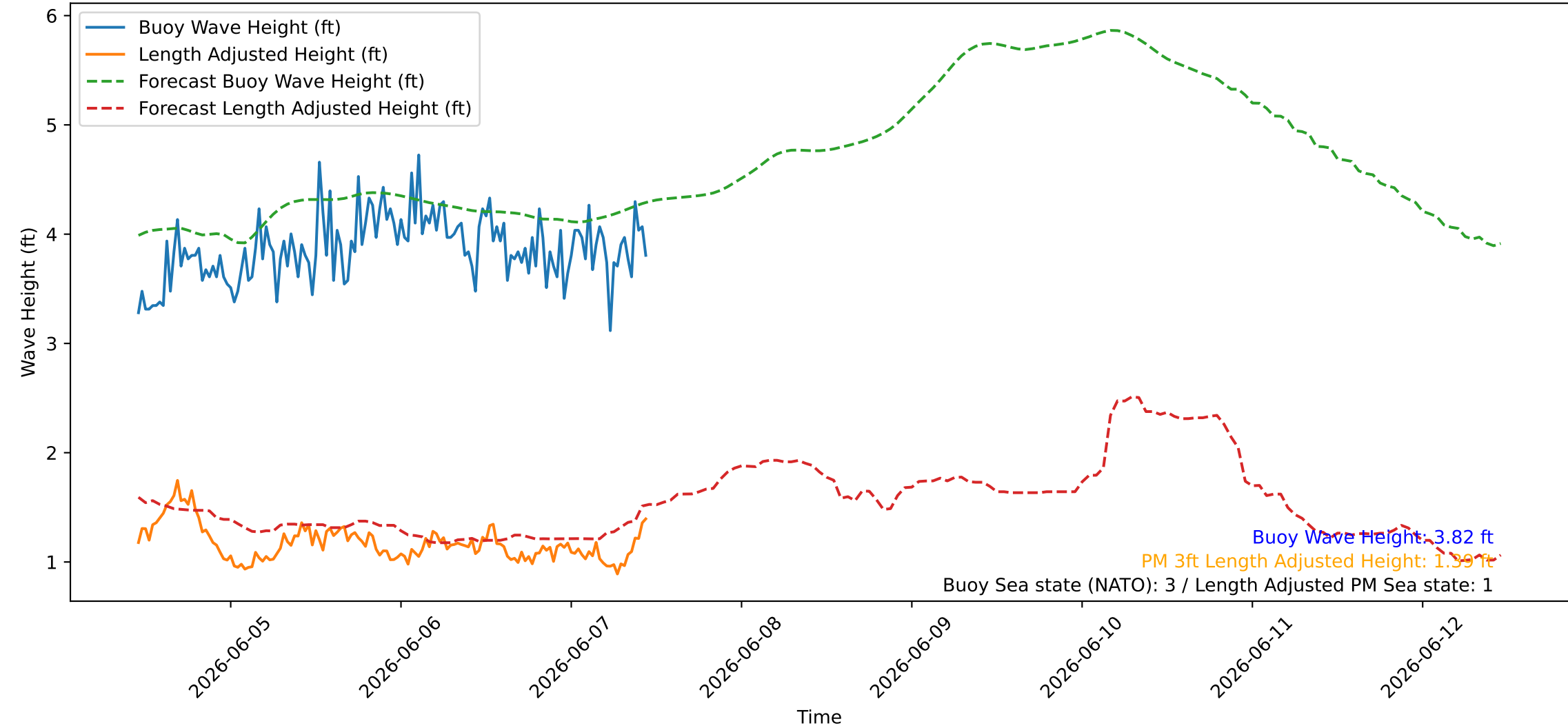
Wave Heights over Time for Green Beach at 2026-06-07 11:11:08
