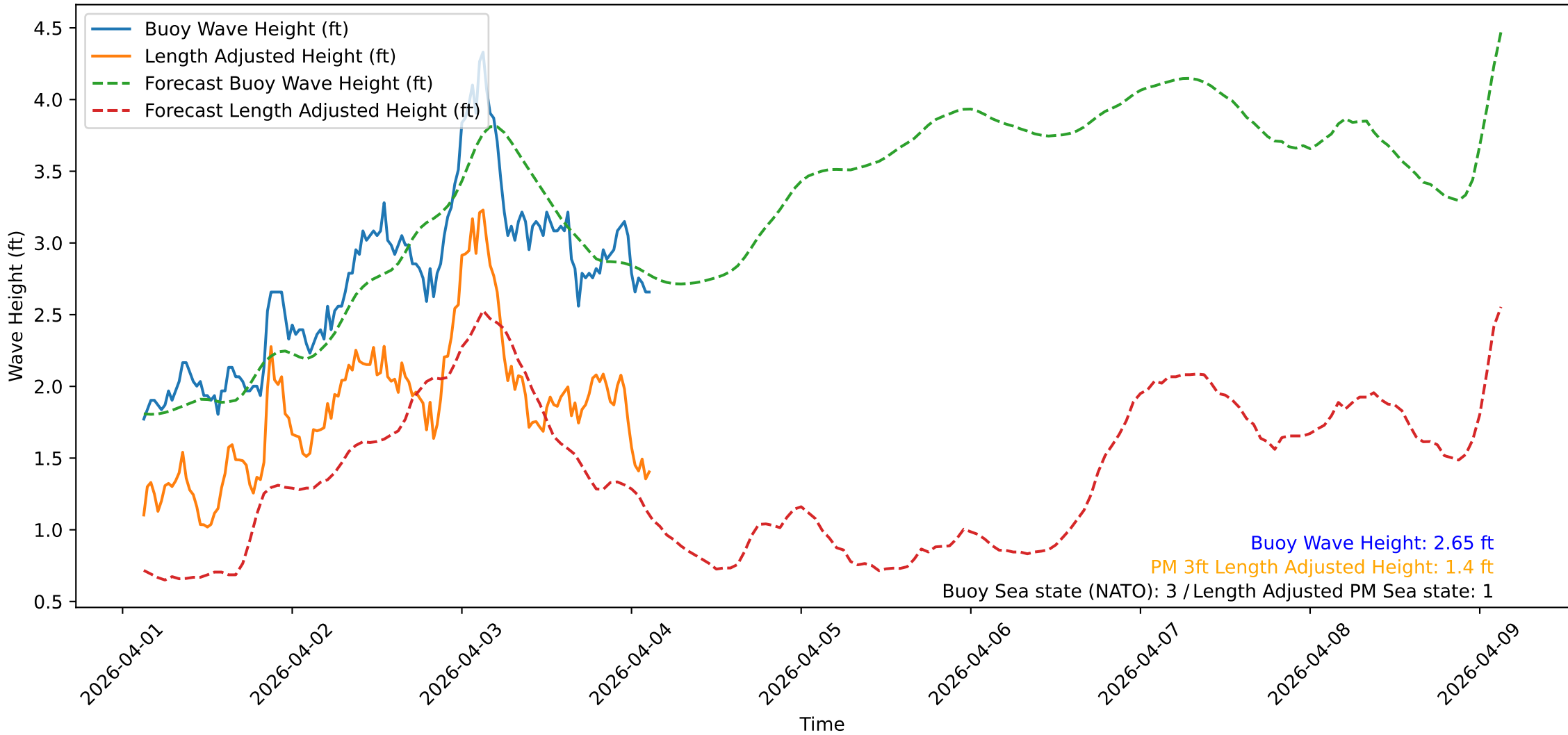
Wave Heights over Time for Green Beach at 2026-04-04 03:11:09
