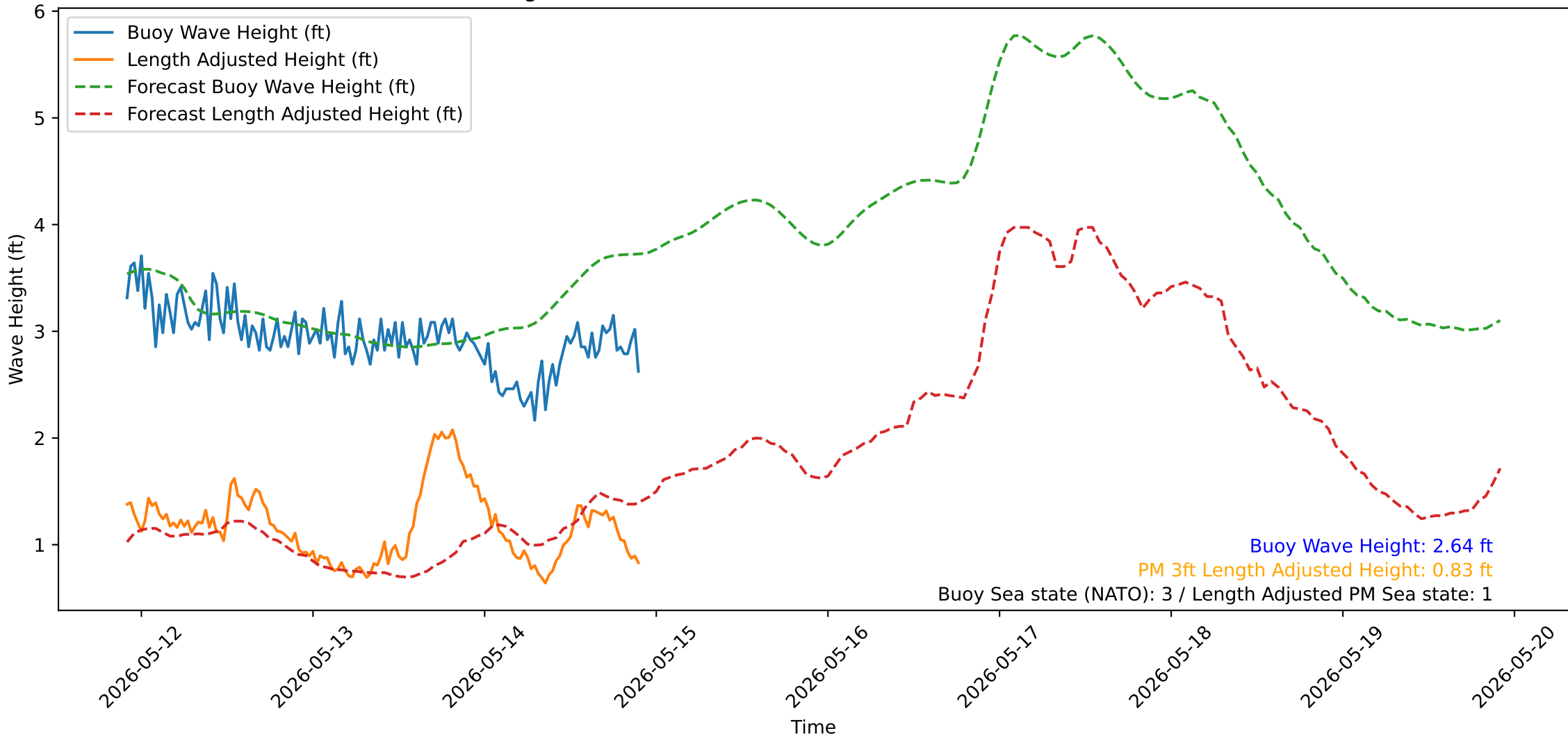
Wave Heights over Time for Oceanside Harbor at 2026-05-14 22:10:32
