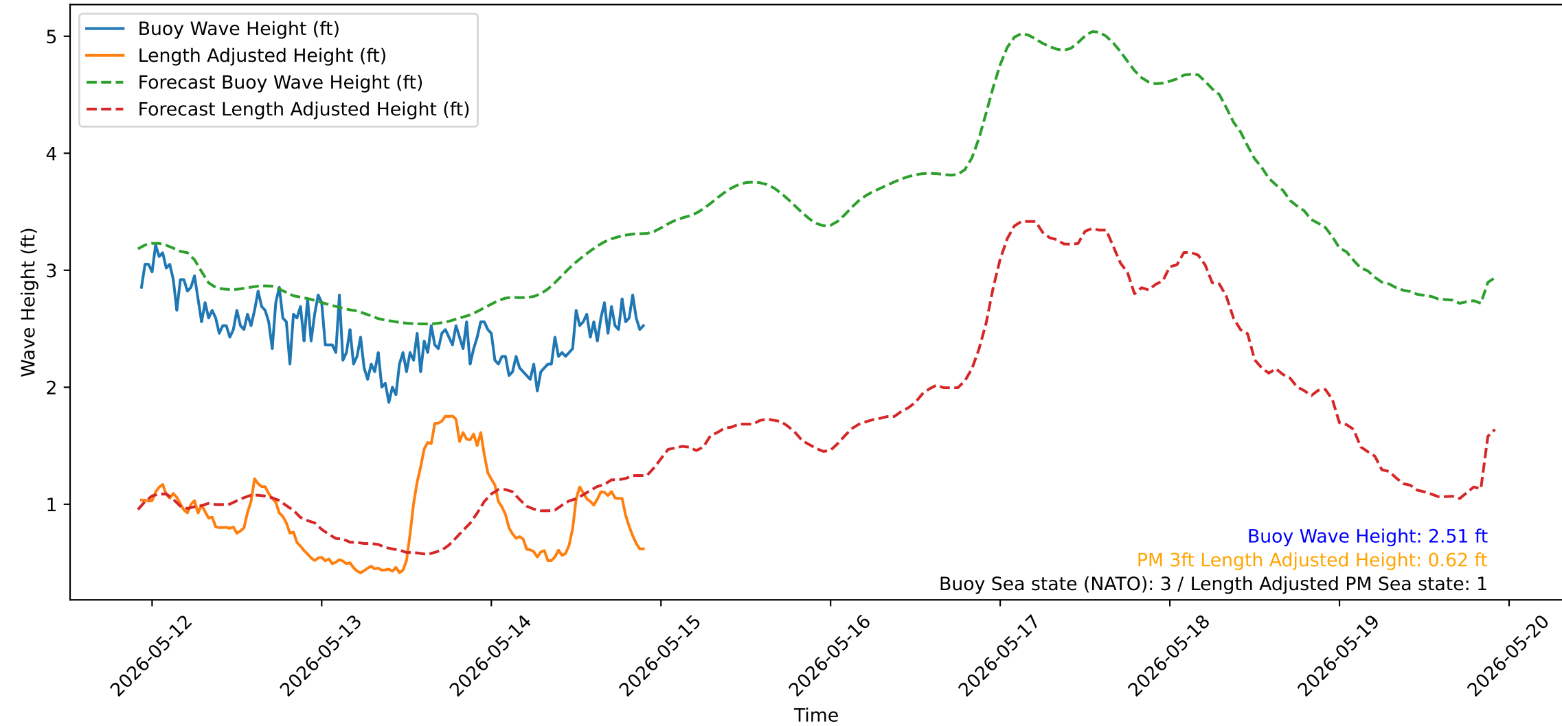
Wave Heights over Time for Red Beach at 2026-05-14 22:10:51
