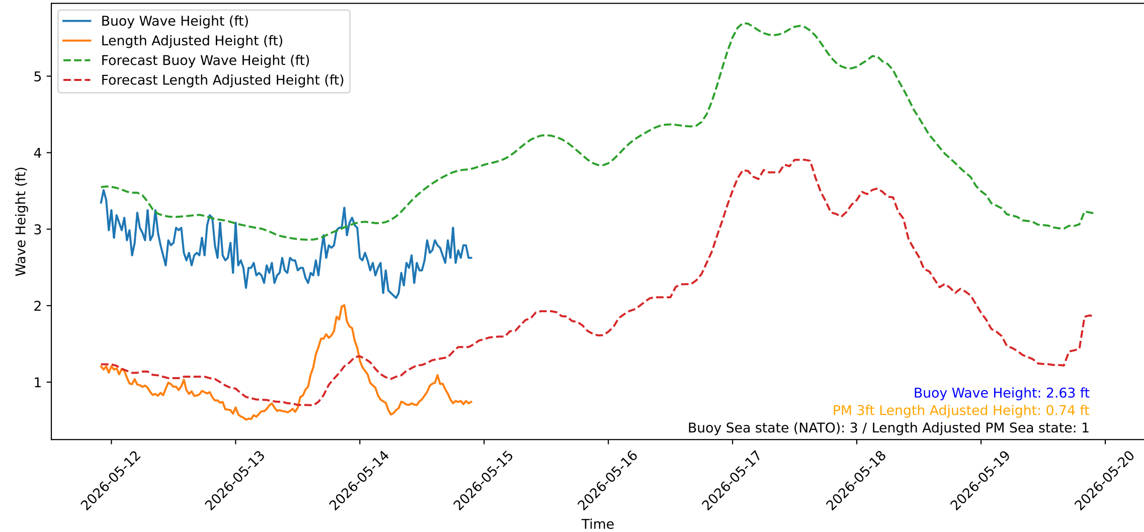
Wave Heights over Time for Green Beach at 2026-05-14 22:11:14
