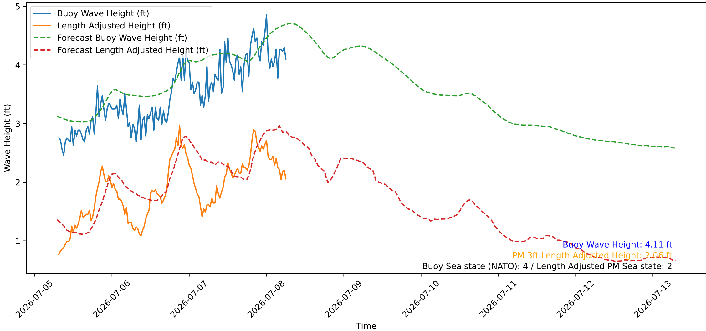
Wave Heights over Time for Red Beach at 2026-07-08 07:00:46
