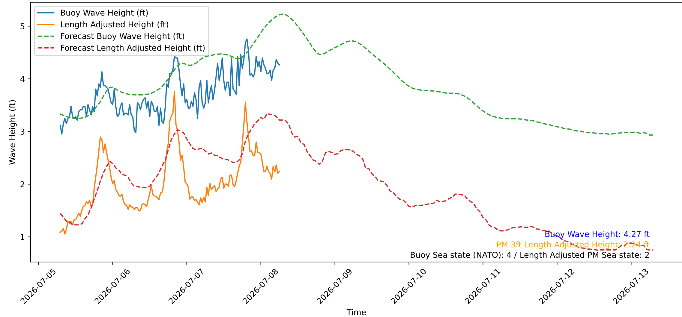
Wave Heights over Time for Green Beach at 2026-07-08 07:01:08
