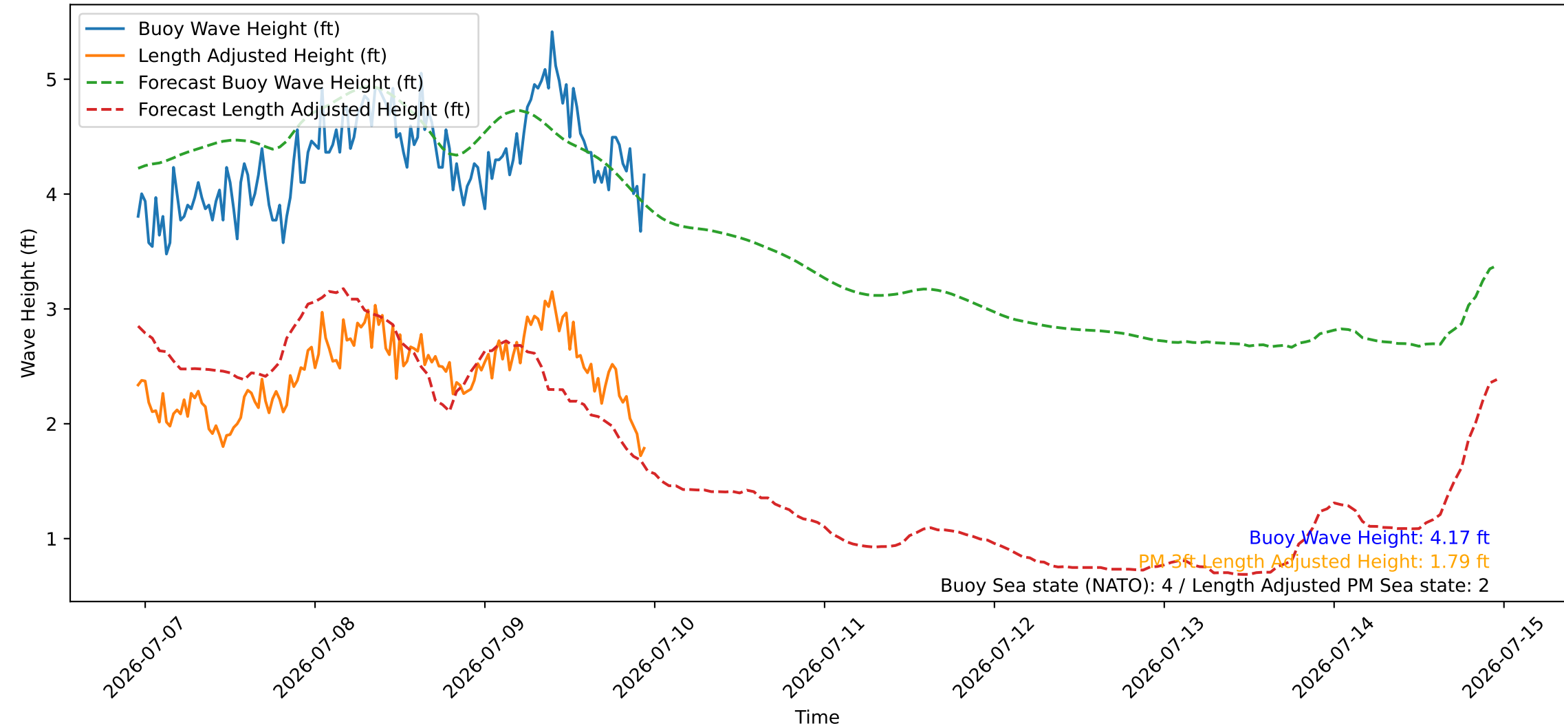
Wave Heights over Time for Oceanside Harbor at 2026-07-09 23:10:26
