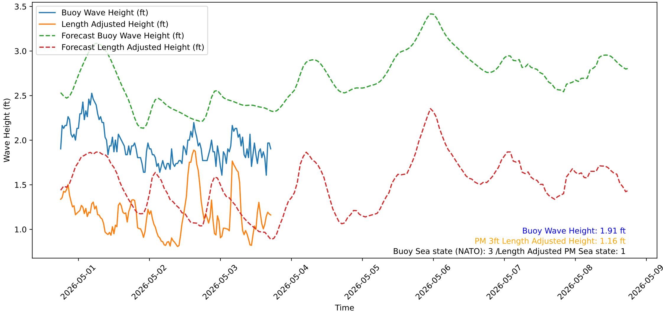
Wave Heights over Time for Red Beach at 2026-05-03 17:50:51
