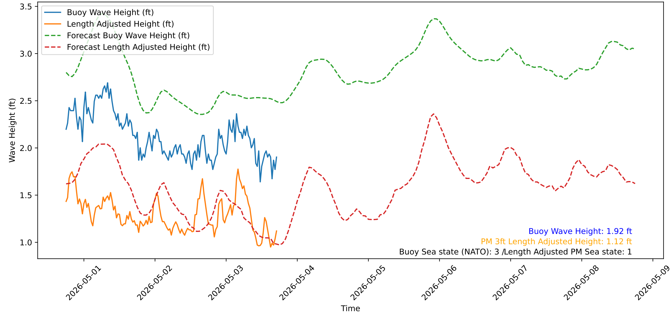
Wave Heights over Time for Oceanside Harbor at 2026-05-03 17:50:31
