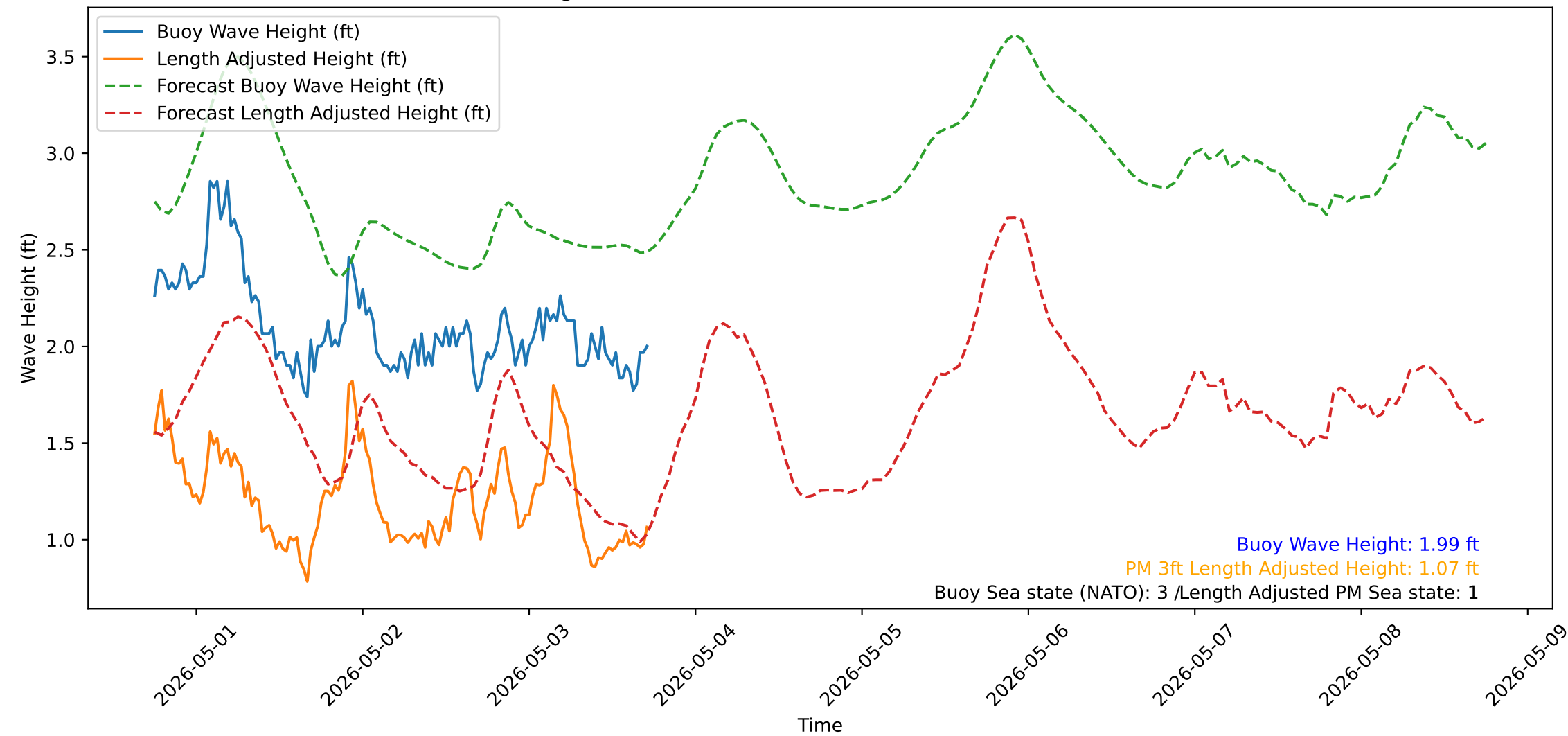
Wave Heights over Time for Green Beach at 2026-05-03 17:51:13
