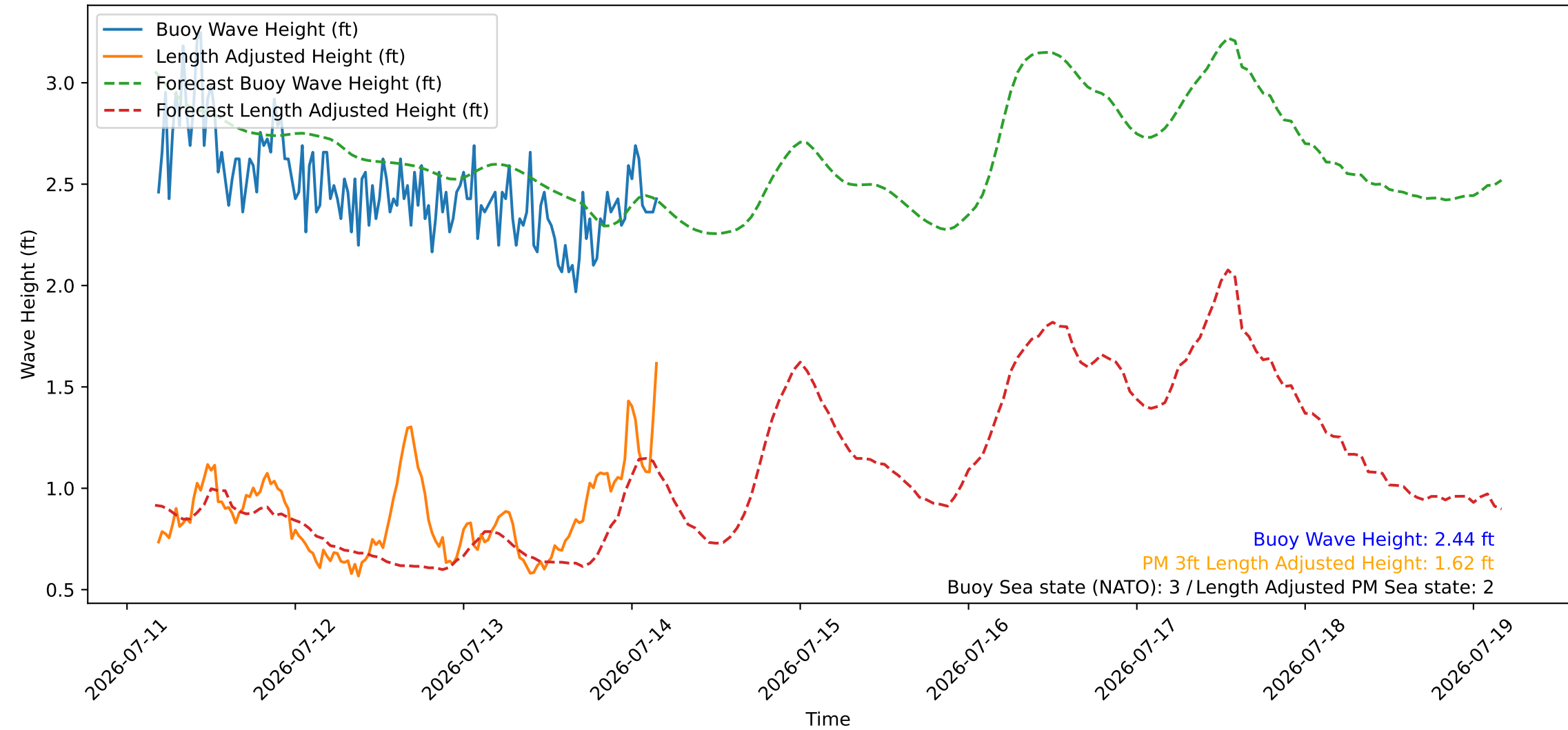
Wave Heights over Time for Red Beach at 2026-07-14 04:20:49
