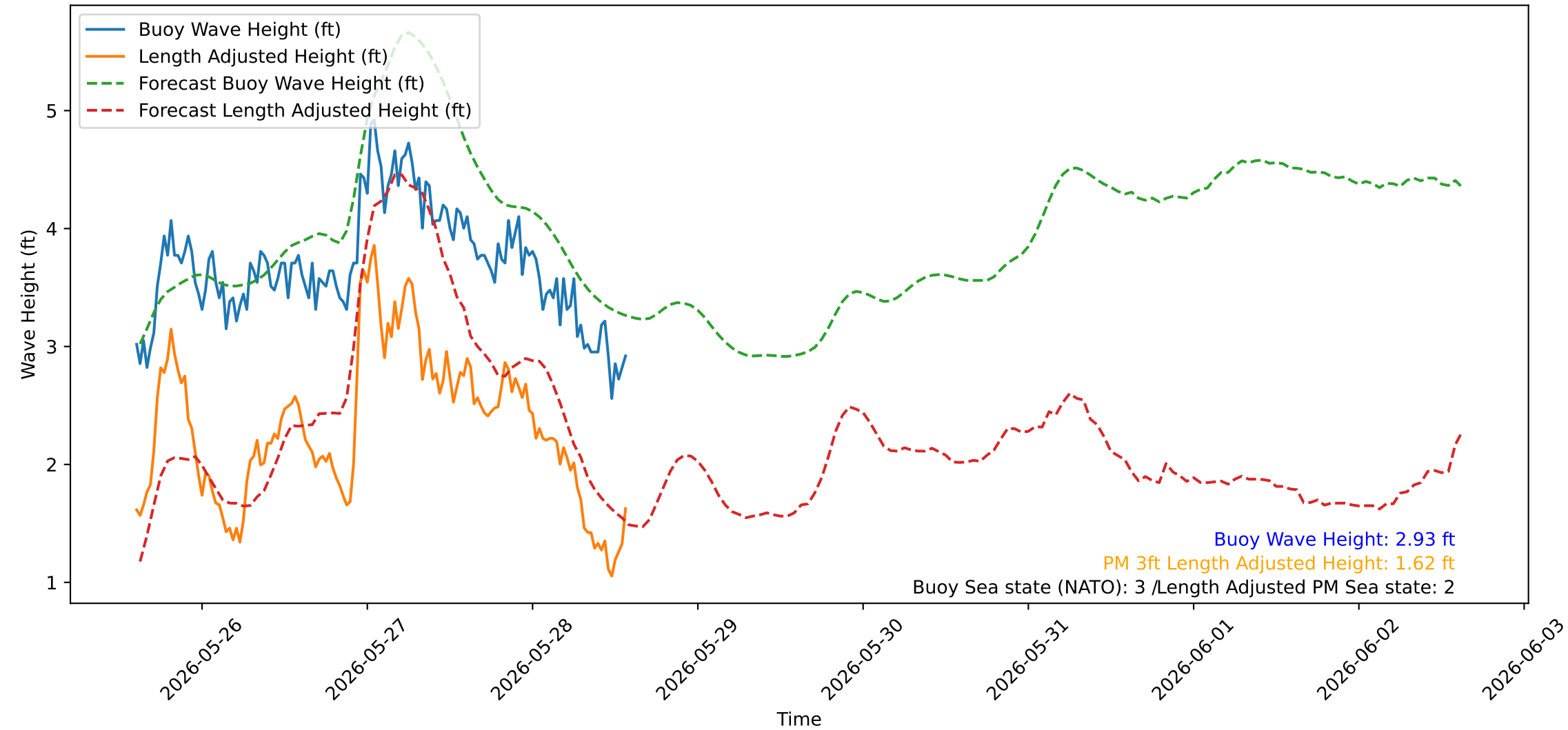
Wave Heights over Time for Green Beach at 2026-05-28 14:31:01
