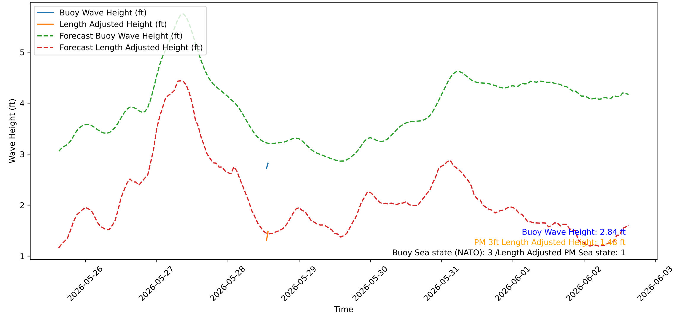
Wave Heights over Time for Oceanside Harbor at 2026-05-28 14:30:19
