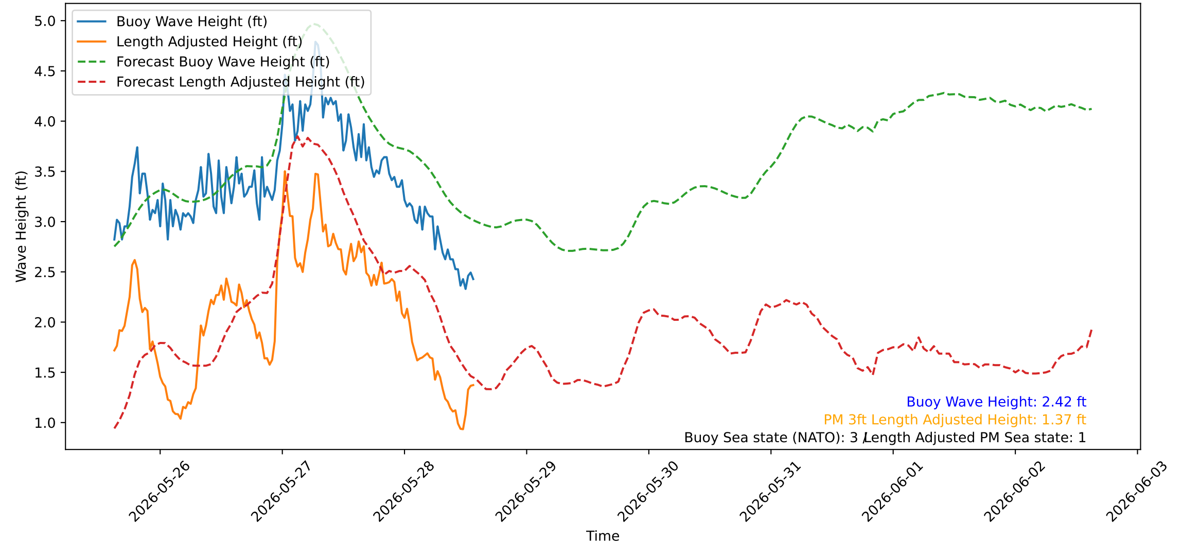
Wave Heights over Time for Red Beach at 2026-05-28 14:30:38
