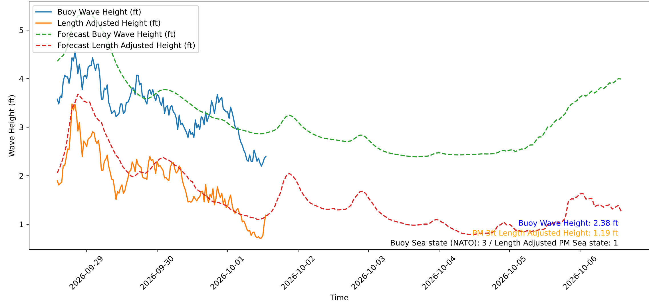
Wave Heights over Time for Green Beach at 2026-10-01 13:51:14
