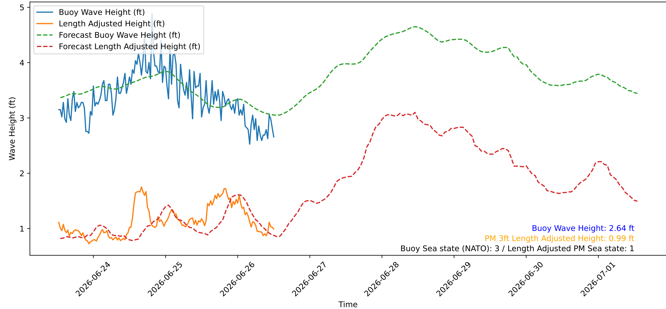
Wave Heights over Time for Oceanside Harbor at 2026-06-26 12:30:26
