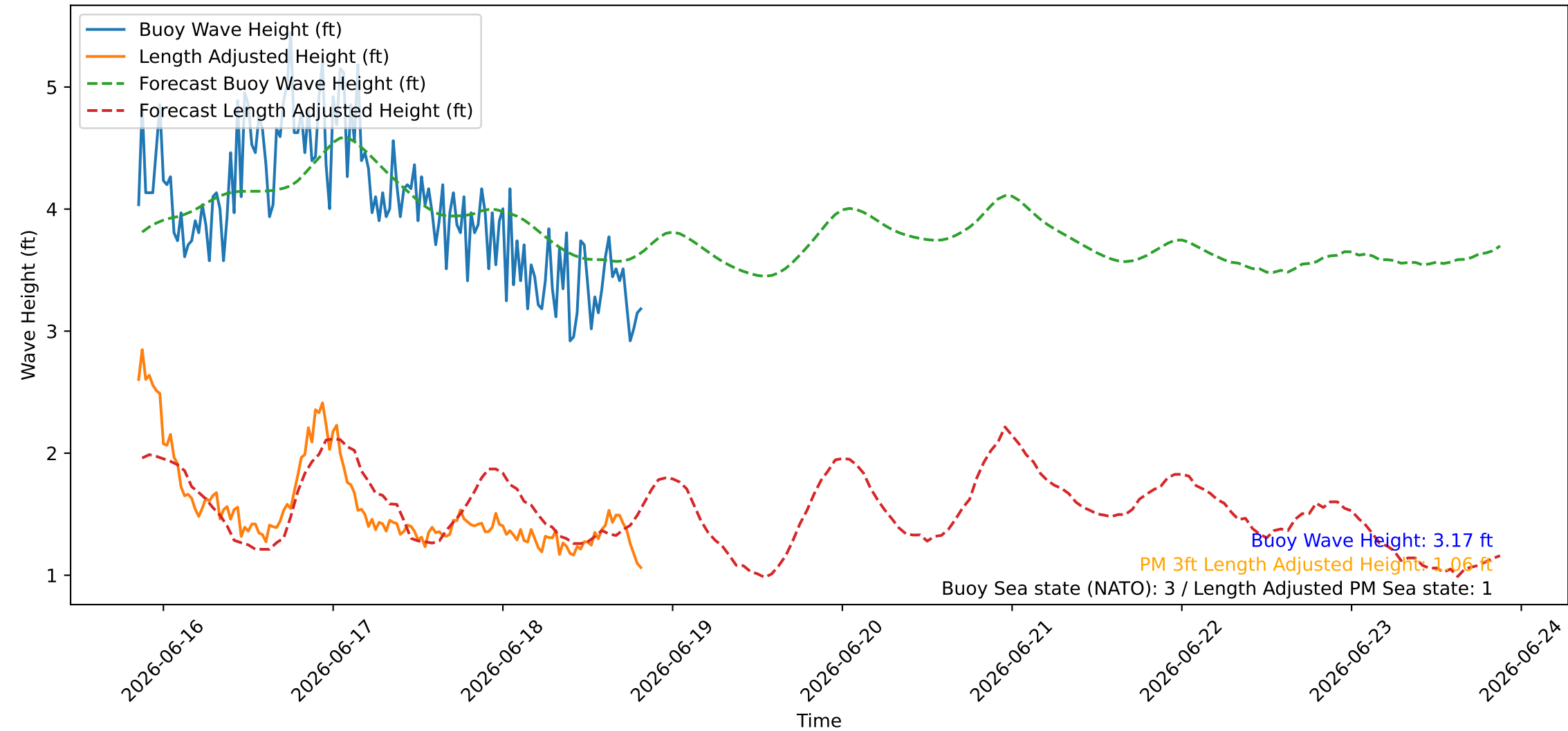
Wave Heights over Time for Oceanside Harbor at 2026-06-18 20:30:26
