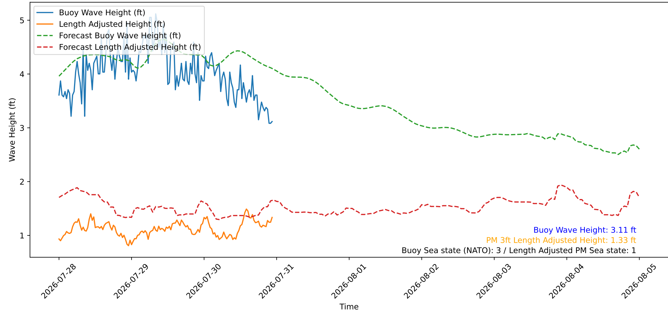
Wave Heights over Time for Red Beach at 2026-07-30 23:30:46
