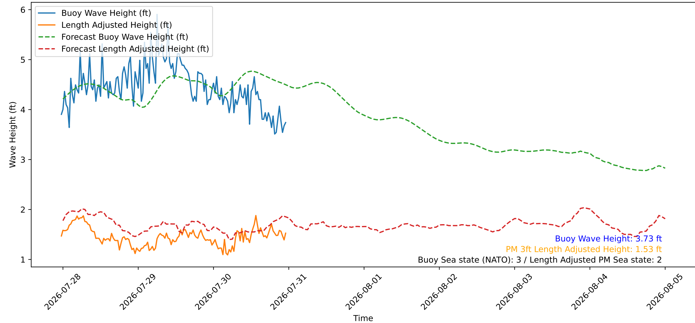
Wave Heights over Time for Oceanside Harbor at 2026-07-30 23:30:26
