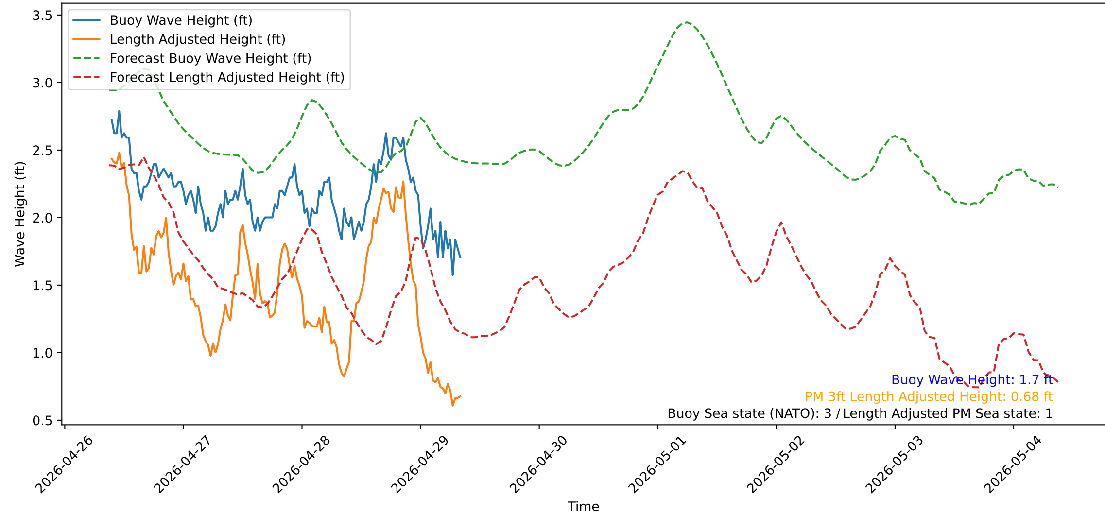
Wave Heights over Time for Red Beach at 2026-04-29 09:00:50
