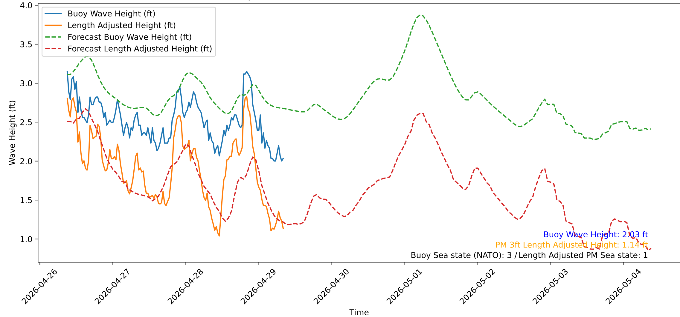
Wave Heights over Time for Green Beach at 2026-04-29 09:01:12
