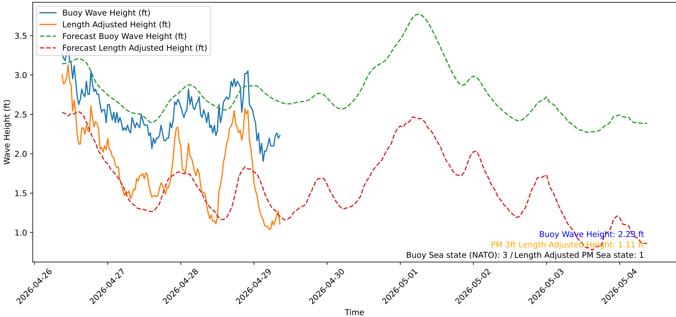
Wave Heights over Time for Oceanside Harbor at 2026-04-29 09:00:31
