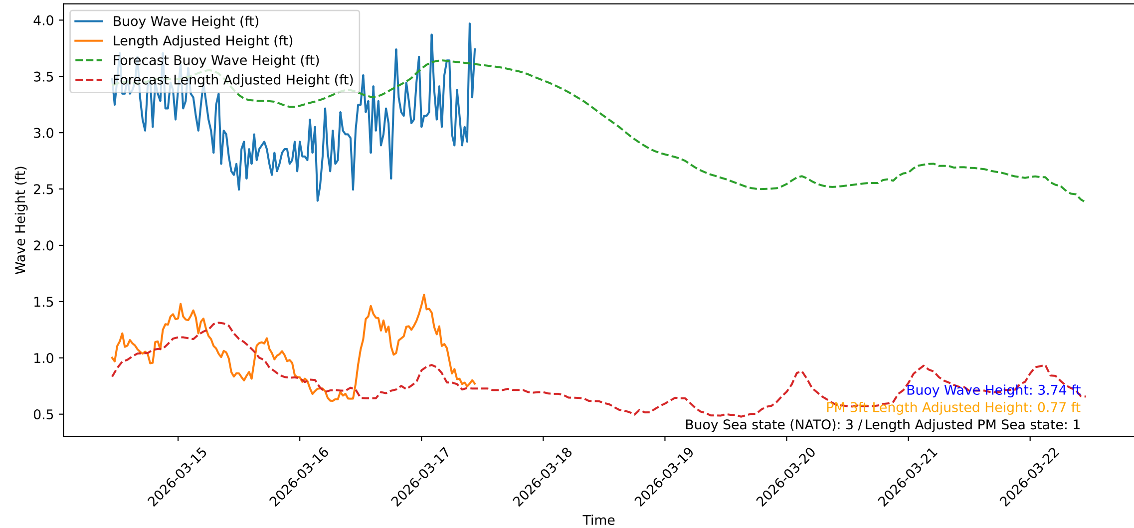
Wave Heights over Time for Oceanside Harbor at 2026-03-17 11:00:43
