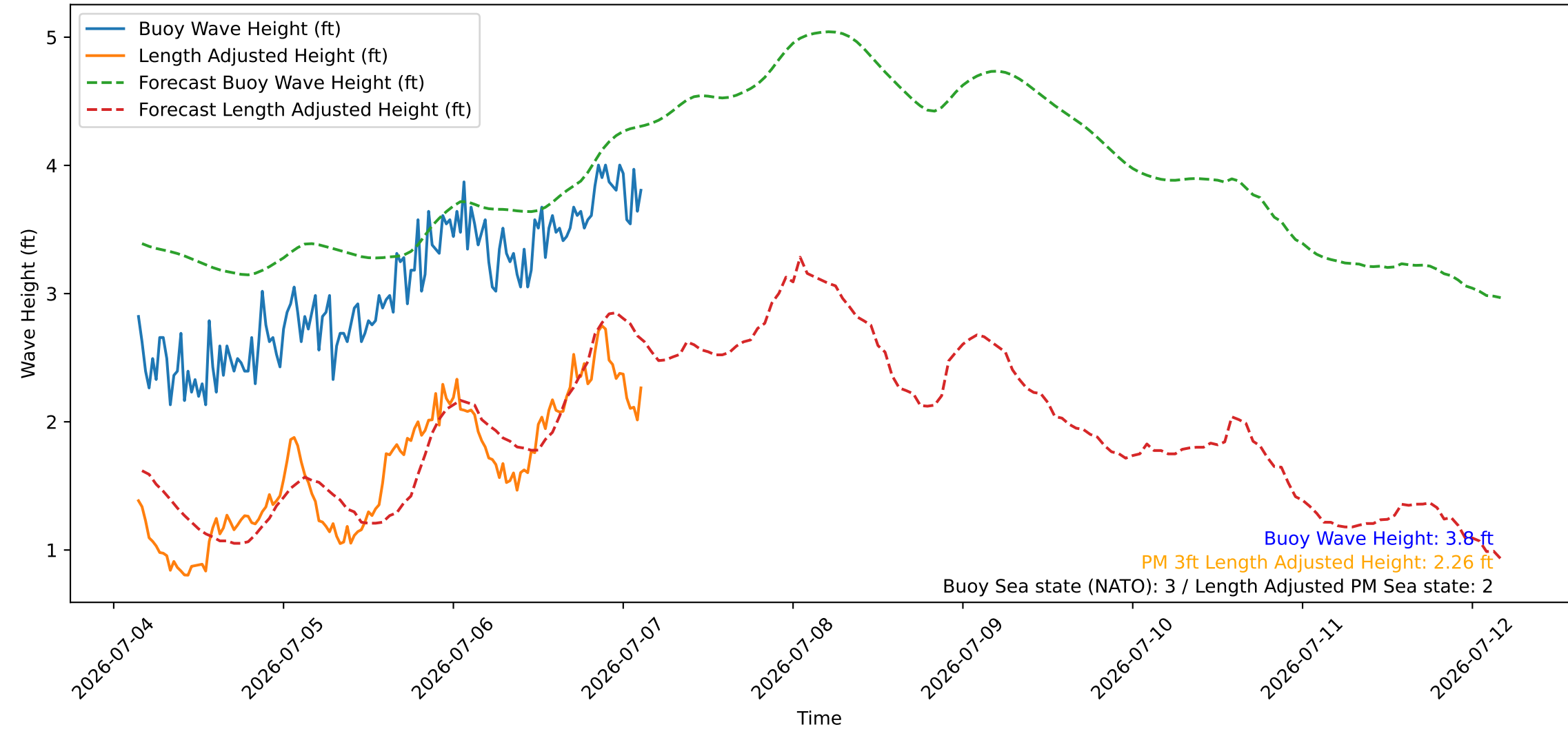
Wave Heights over Time for Oceanside Harbor at 2026-07-07 03:30:26
