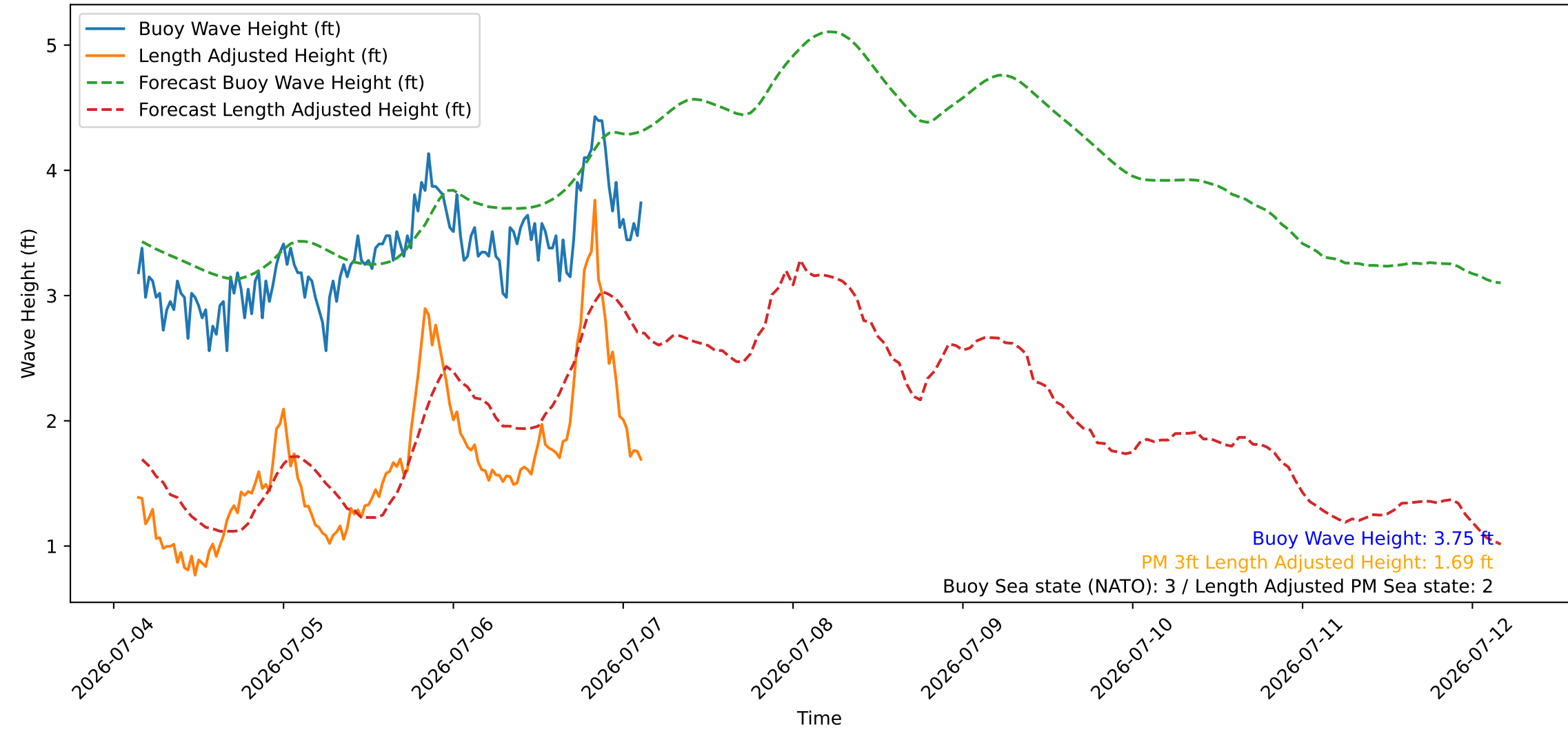
Wave Heights over Time for Green Beach at 2026-07-07 03:31:07
