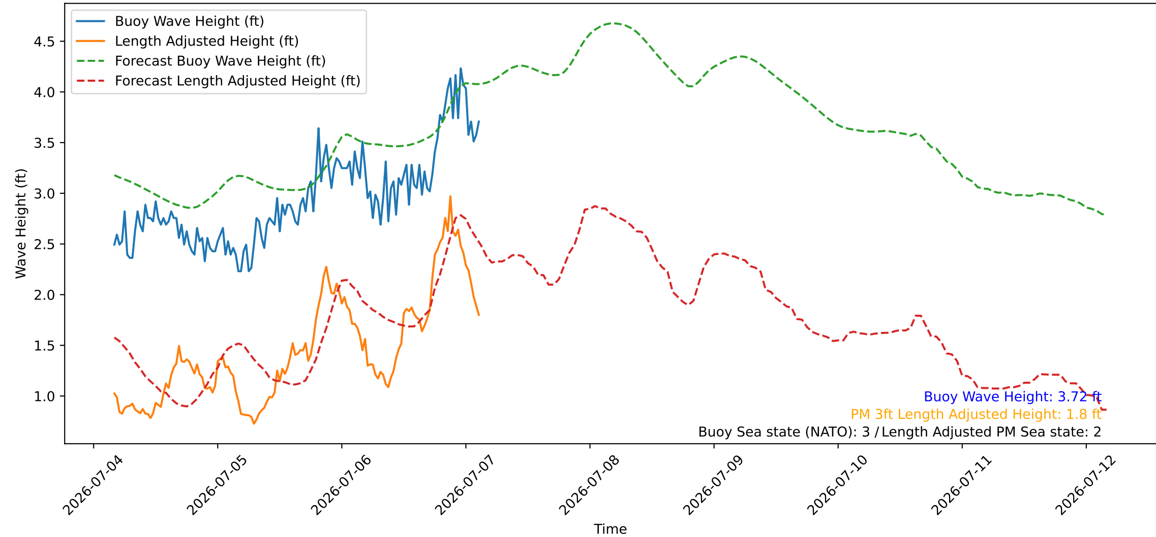
Wave Heights over Time for Red Beach at 2026-07-07 03:30:45
