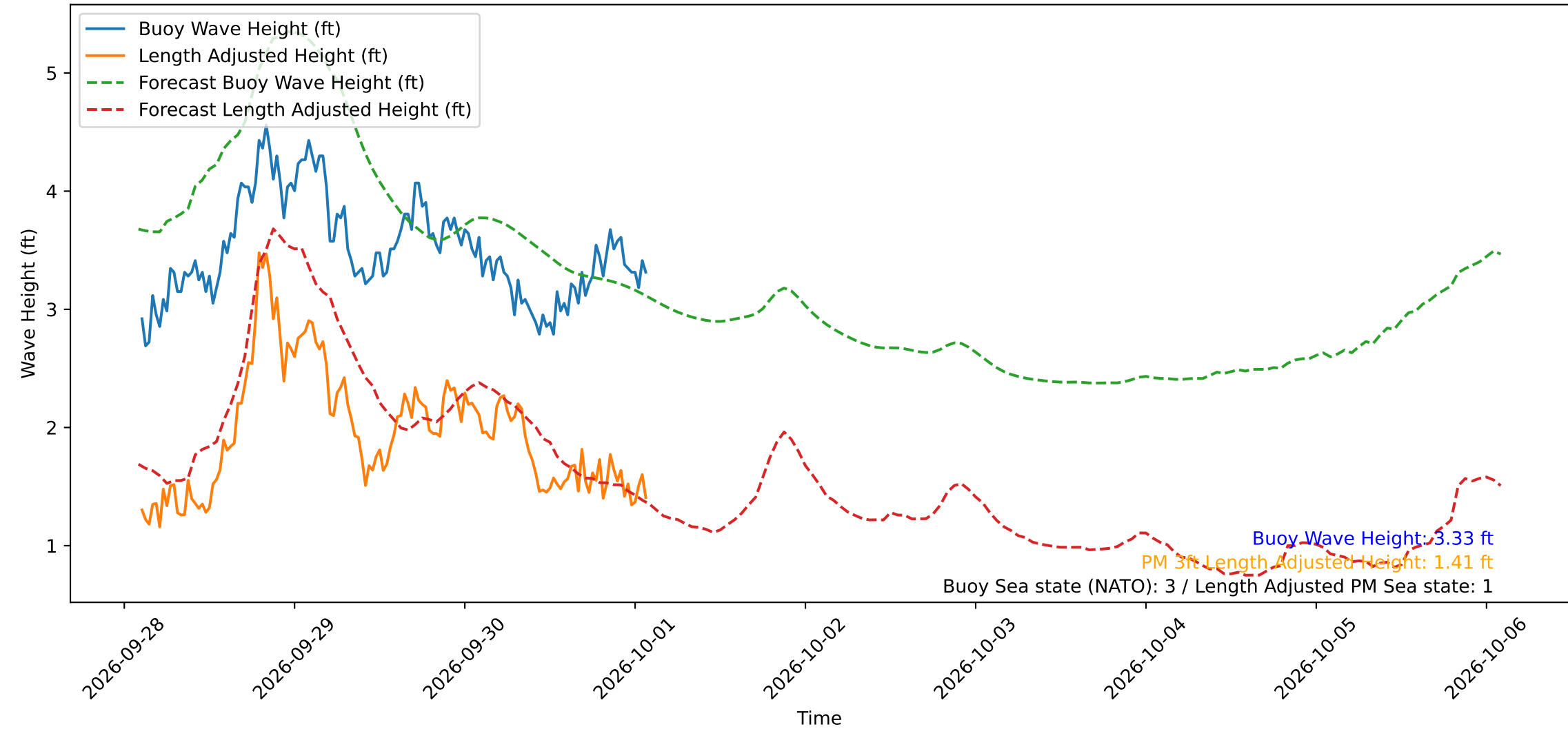
Wave Heights over Time for Green Beach at 2026-10-01 02:21:15
