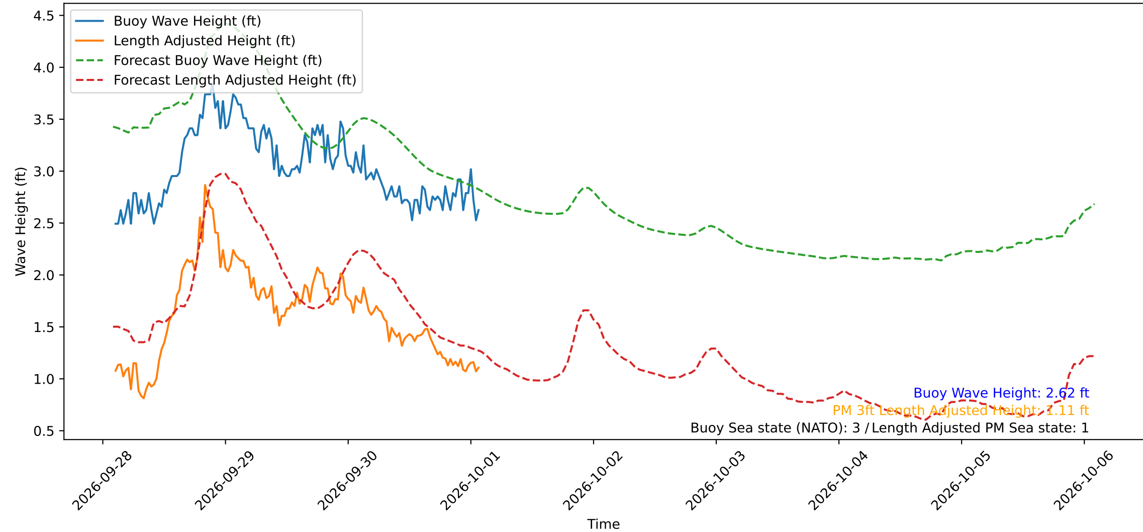
Wave Heights over Time for Red Beach at 2026-10-01 02:20:51
