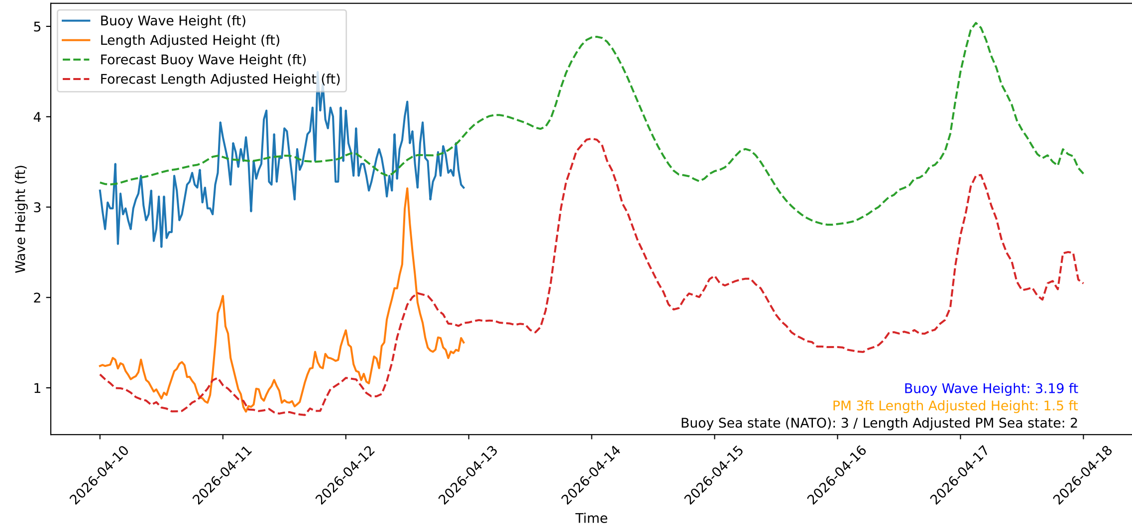
Wave Heights over Time for Green Beach at 2026-04-12 23:51:13
