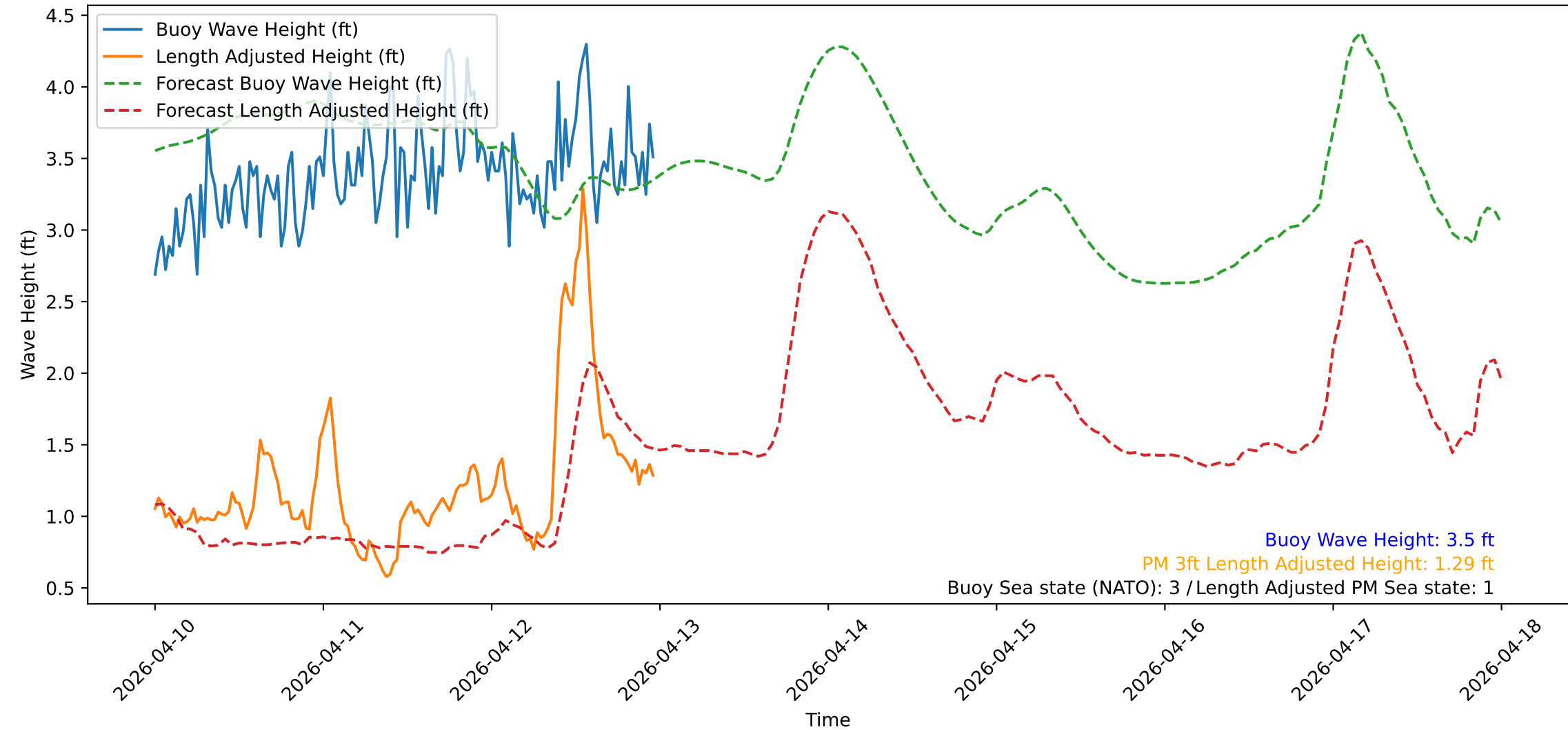
Wave Heights over Time for Red Beach at 2026-04-12 23:50:51
