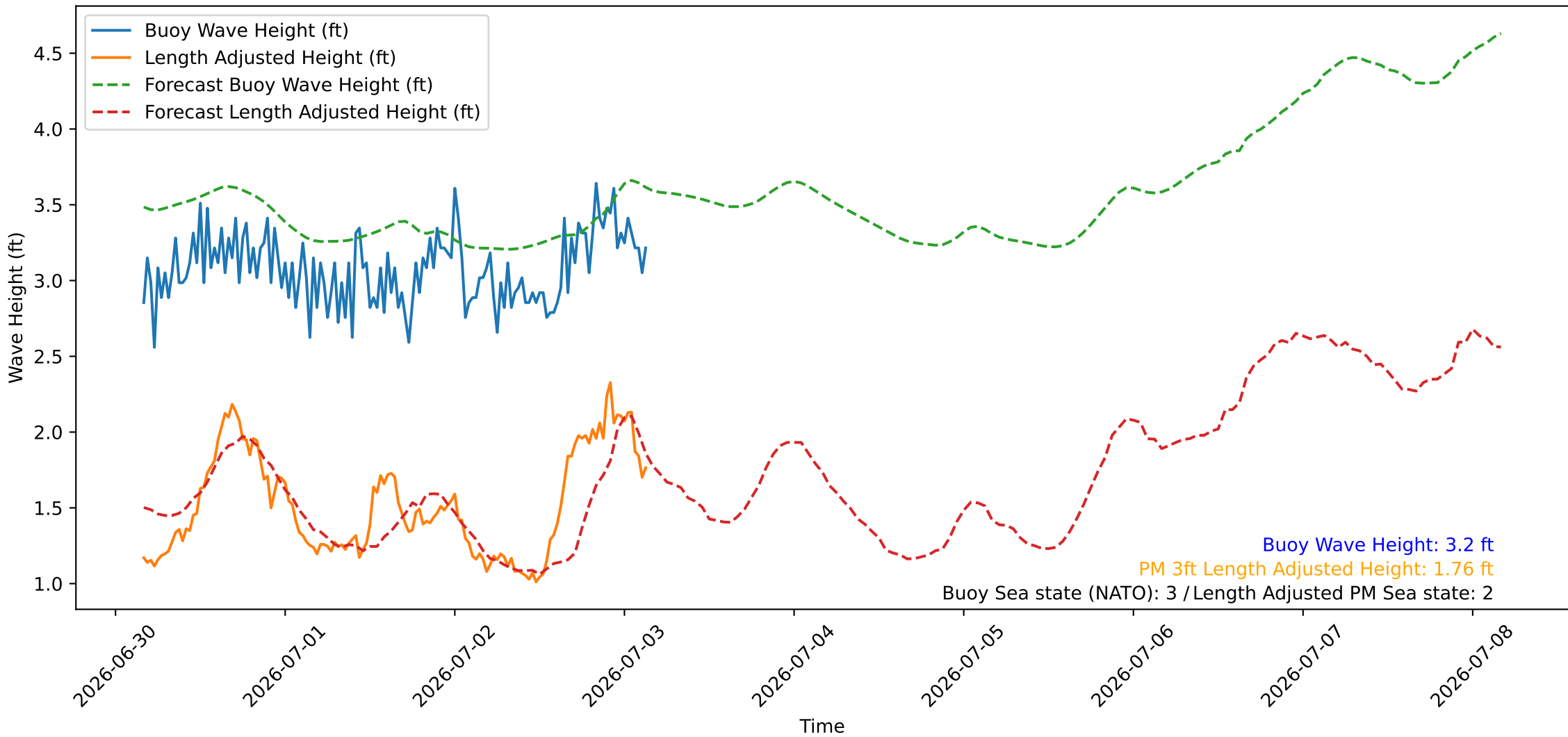
Wave Heights over Time for Oceanside Harbor at 2026-07-03 03:50:25
