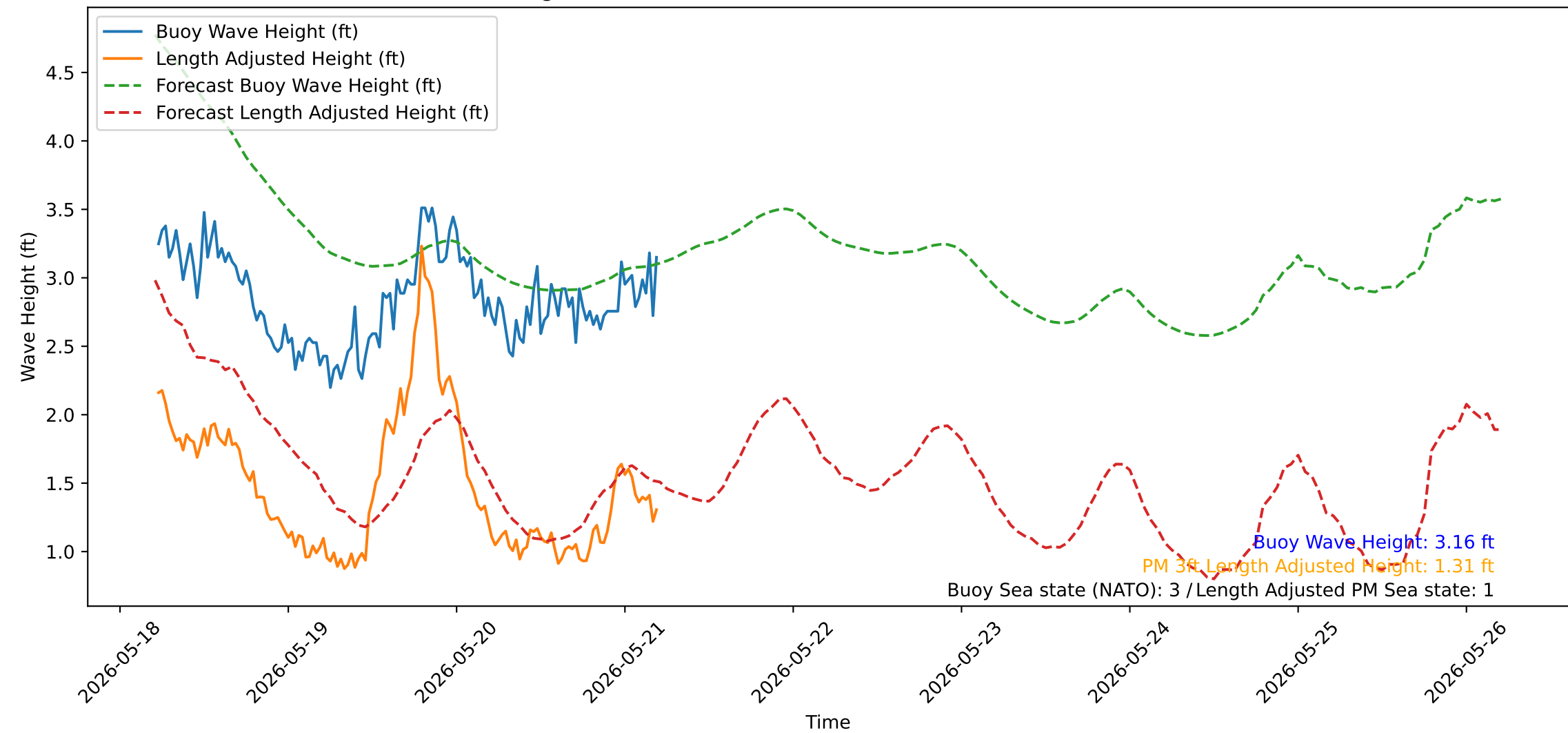
Wave Heights over Time for Oceanside Harbor at 2026-05-21 05:20:32
