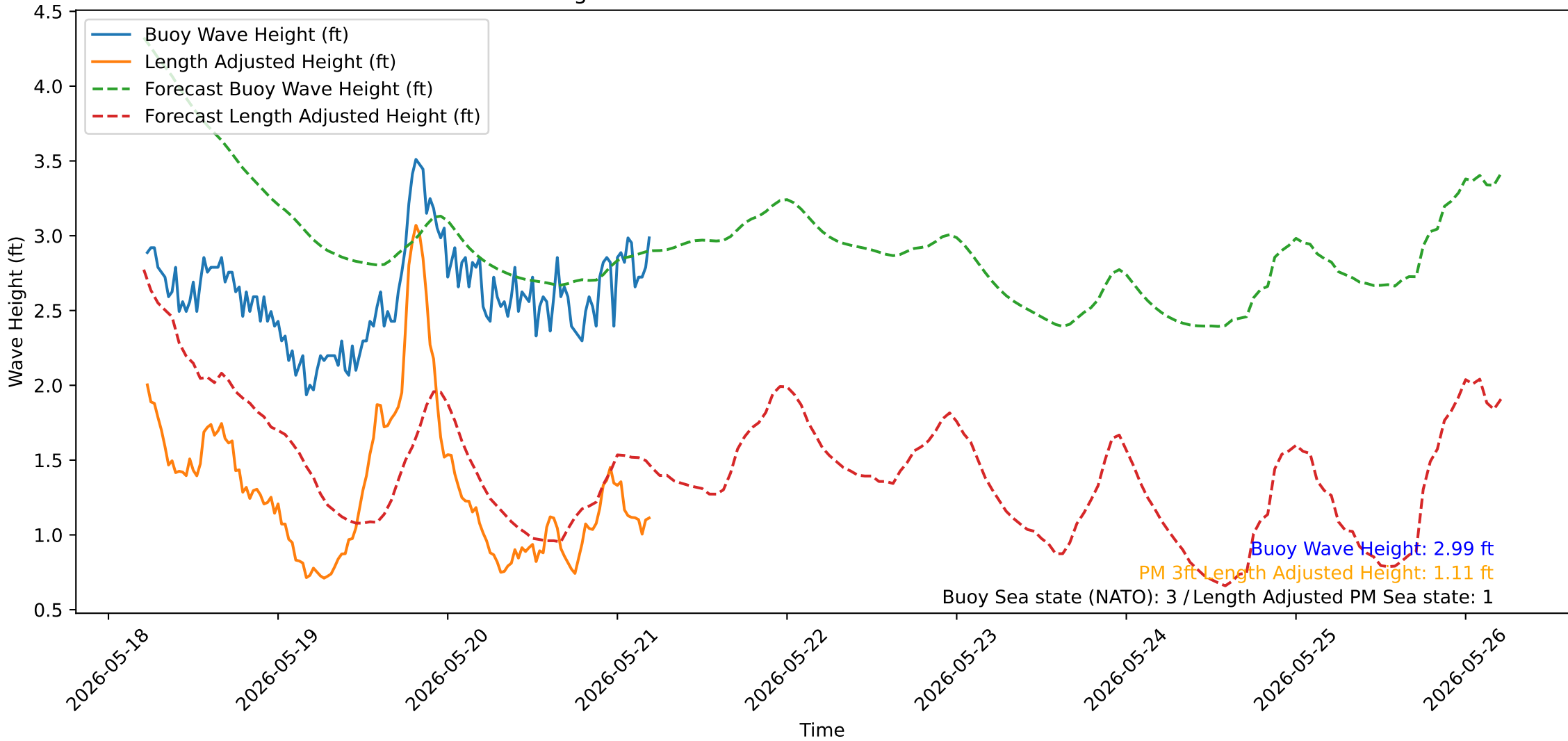
Wave Heights over Time for Red Beach at 2026-05-21 05:20:52
