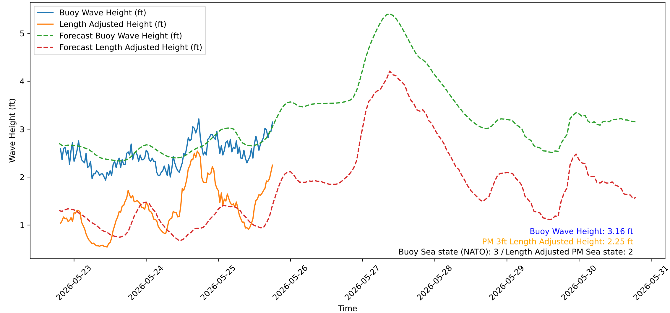
Wave Heights over Time for Red Beach at 2026-05-25 19:00:48
