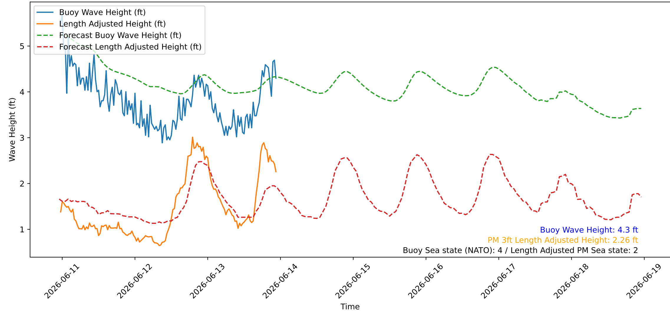
Wave Heights over Time for Green Beach at 2026-06-13 23:21:09
