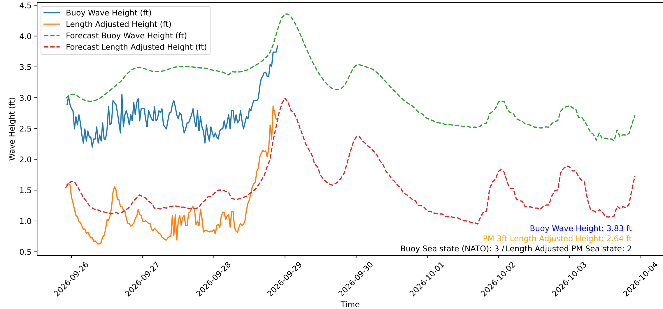
Wave Heights over Time for Red Beach at 2026-09-28 22:10:50
