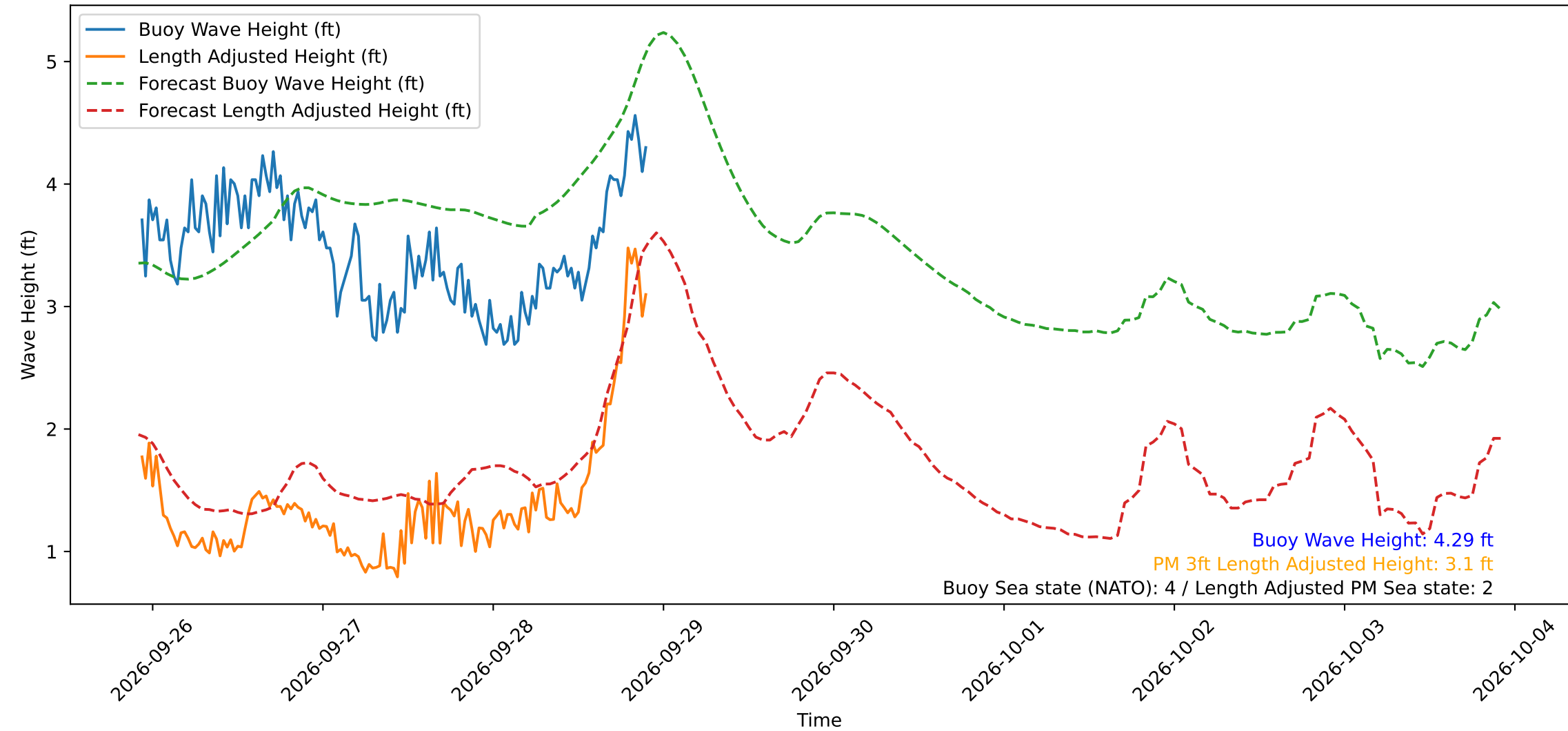
Wave Heights over Time for Green Beach at 2026-09-28 22:11:12
