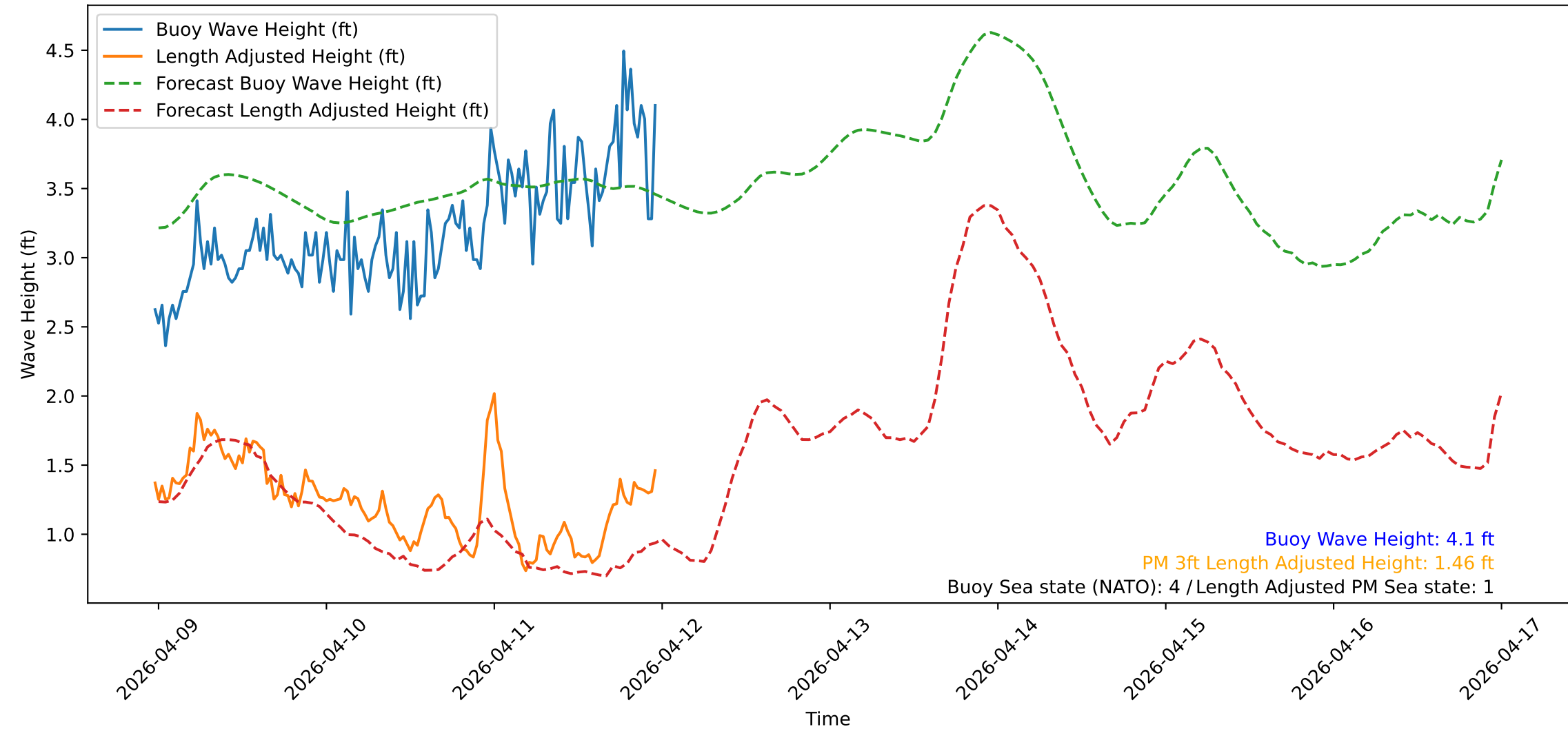
Wave Heights over Time for Green Beach at 2026-04-11 23:41:13
