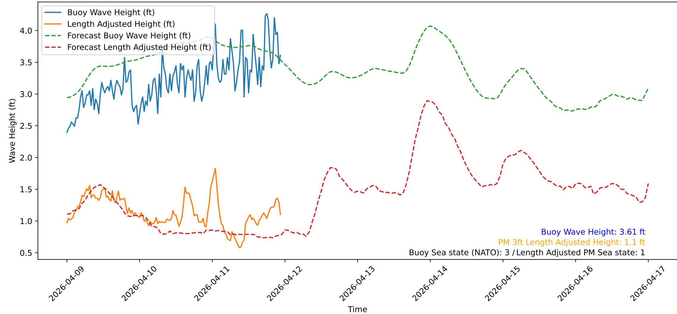
Wave Heights over Time for Red Beach at 2026-04-11 23:40:50
