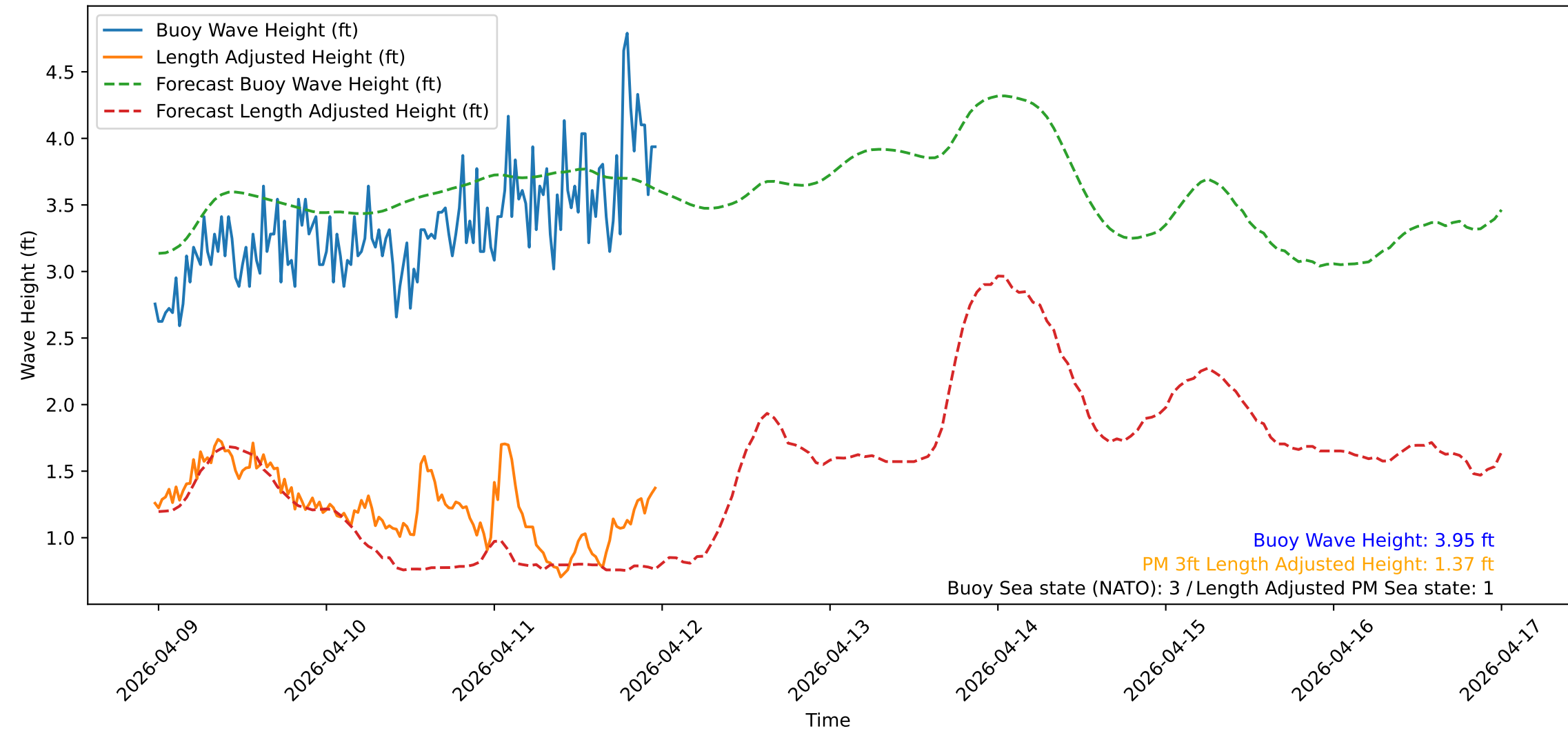
Wave Heights over Time for Oceanside Harbor at 2026-04-11 23:40:31
