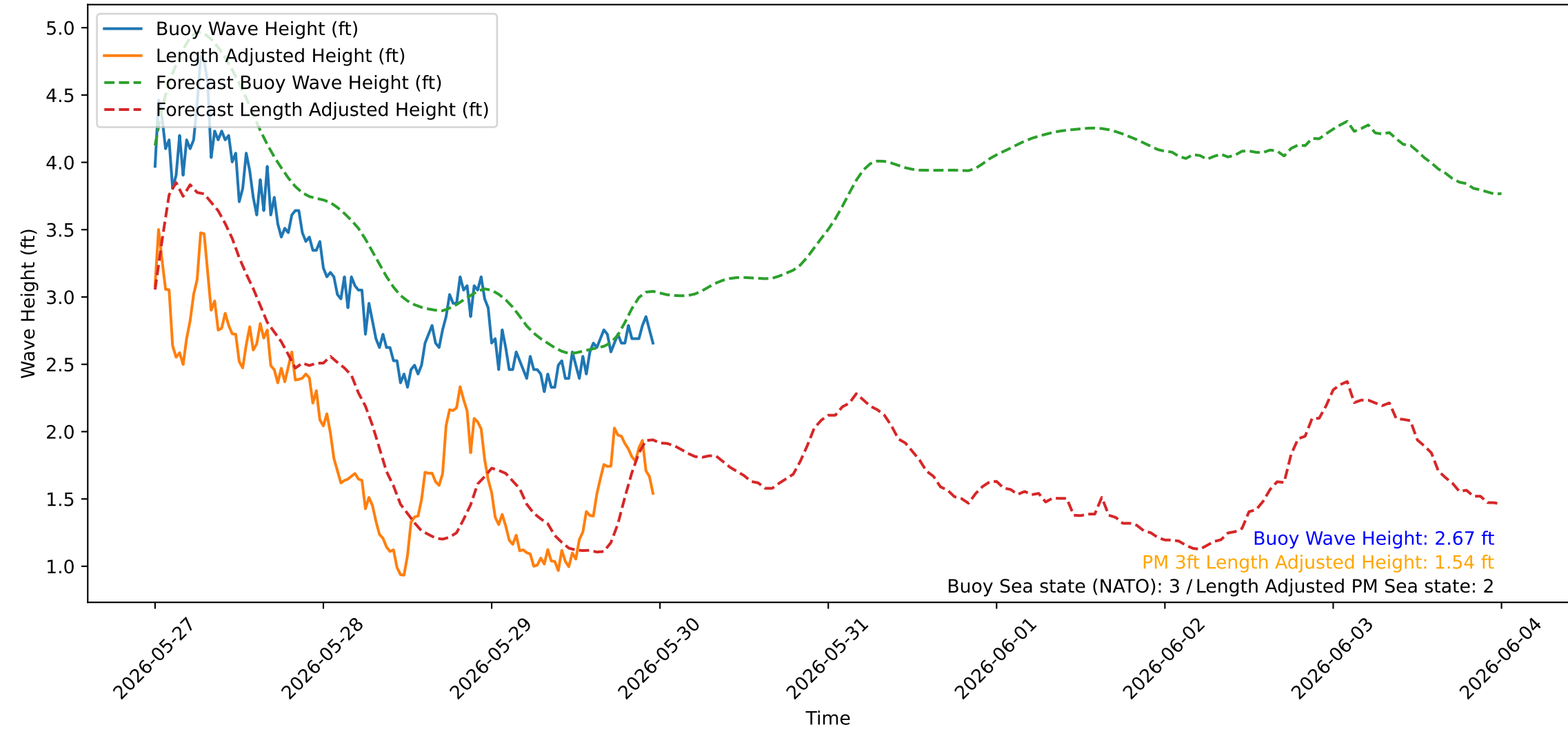
Wave Heights over Time for Red Beach at 2026-05-29 23:40:42
