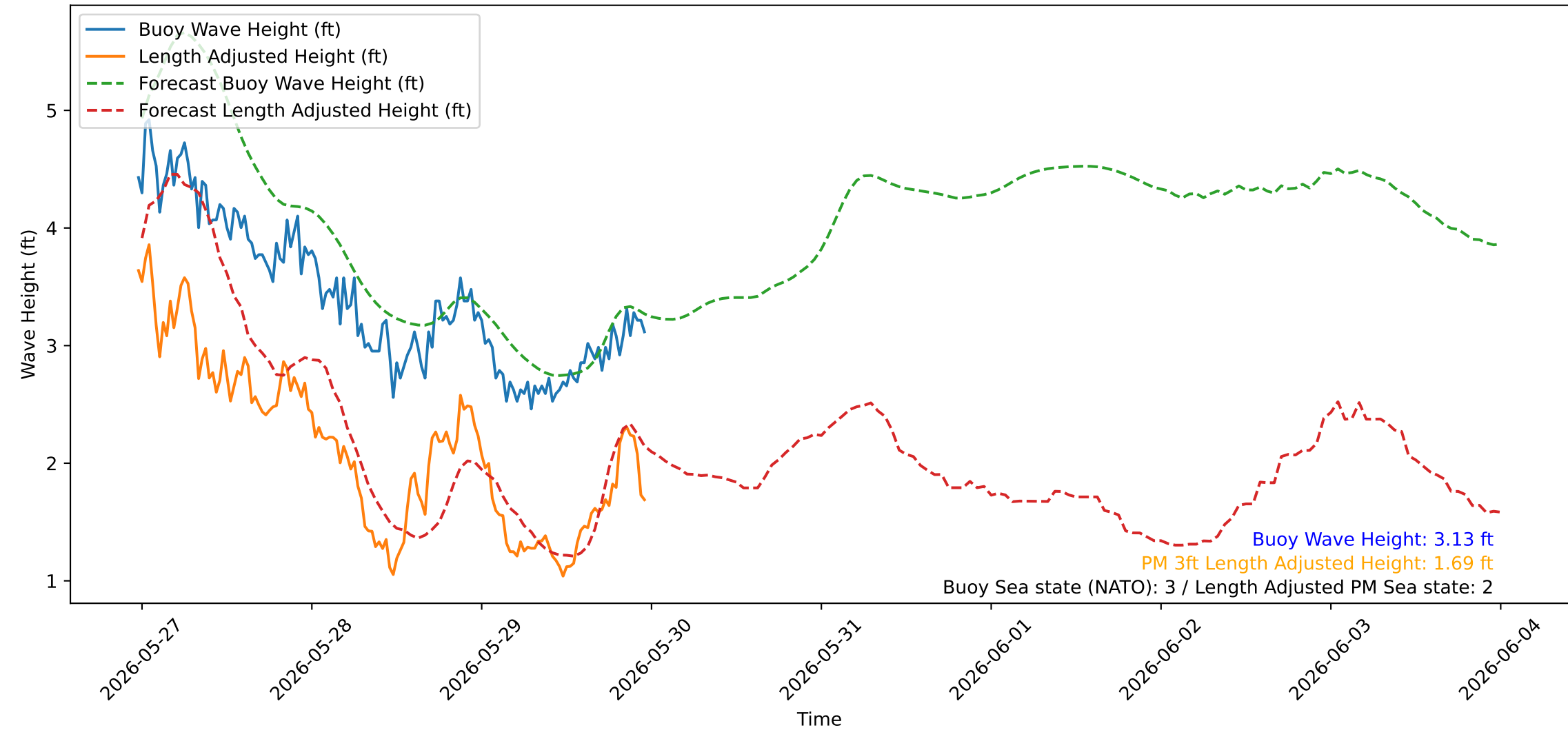
Wave Heights over Time for Green Beach at 2026-05-29 23:41:05
