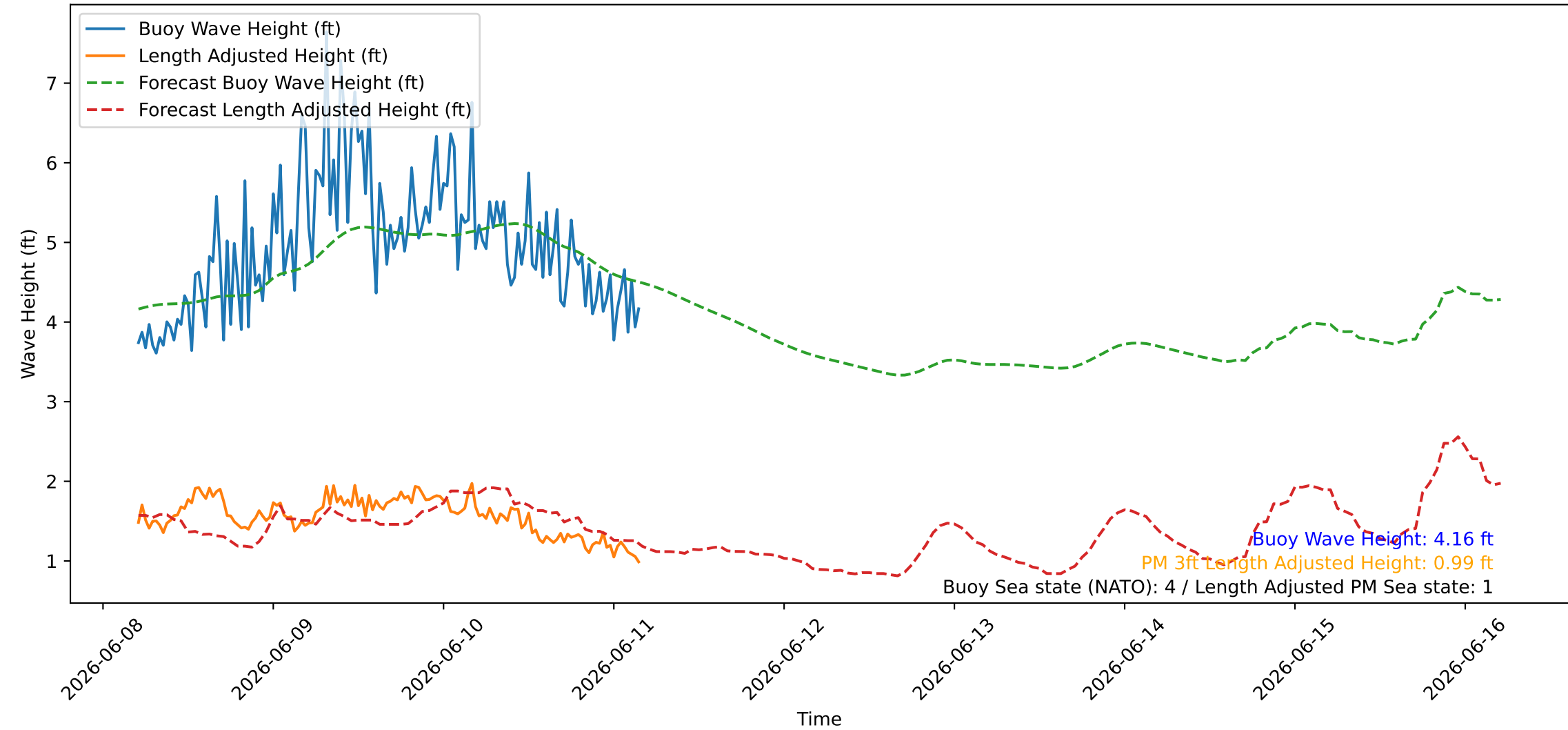
Wave Heights over Time for Red Beach at 2026-06-11 04:30:46
