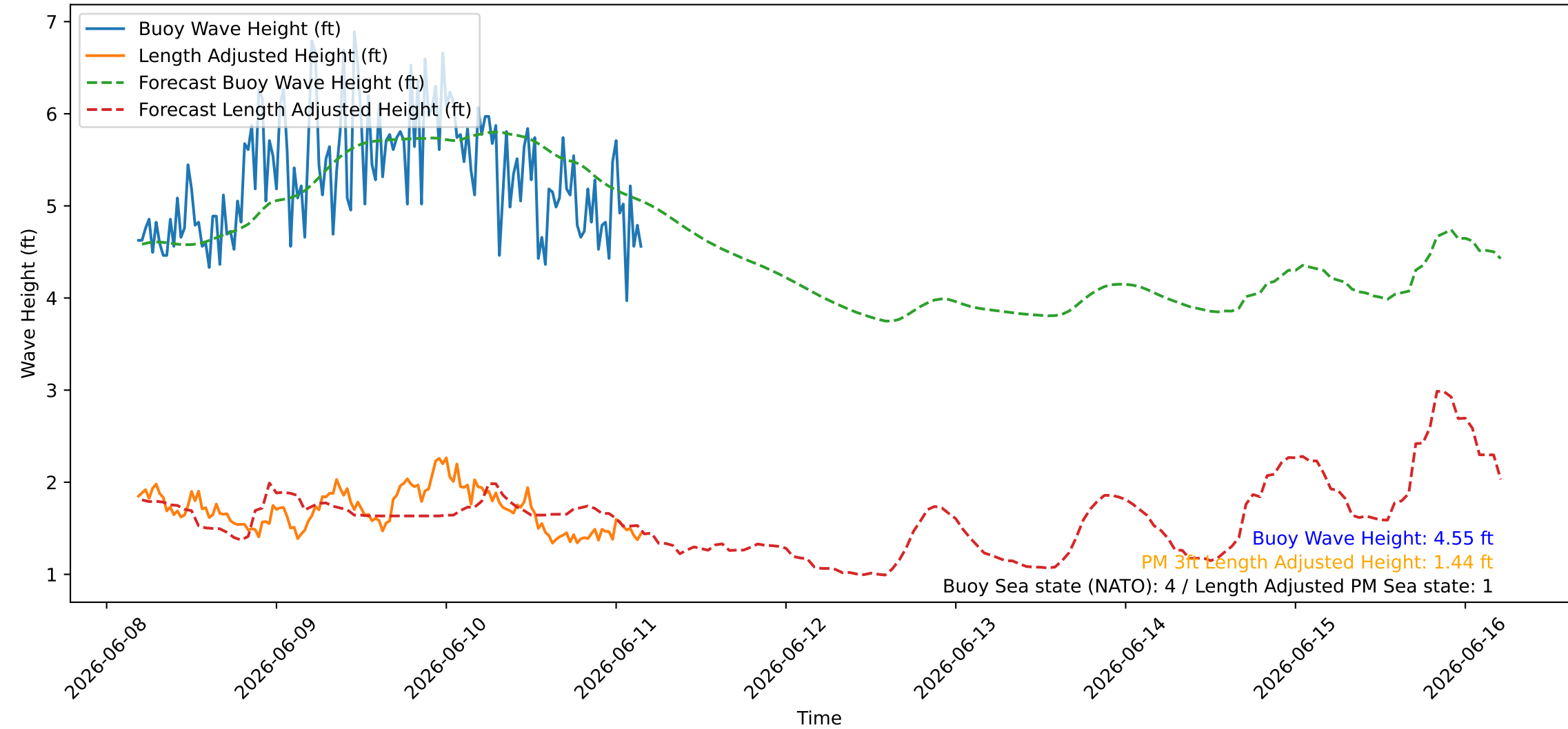
Wave Heights over Time for Green Beach at 2026-06-11 04:31:10
