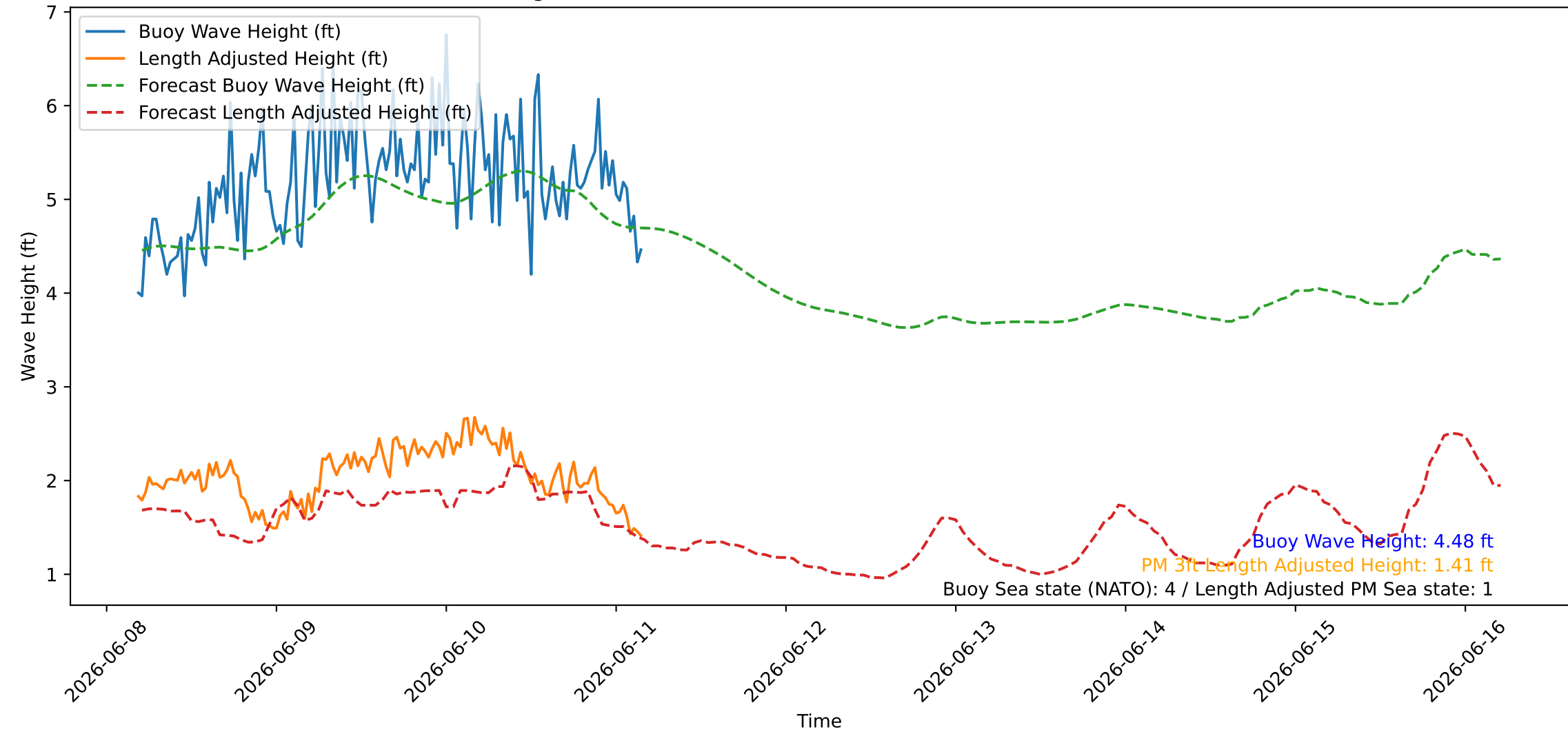
Wave Heights over Time for Oceanside Harbor at 2026-06-11 04:30:26
