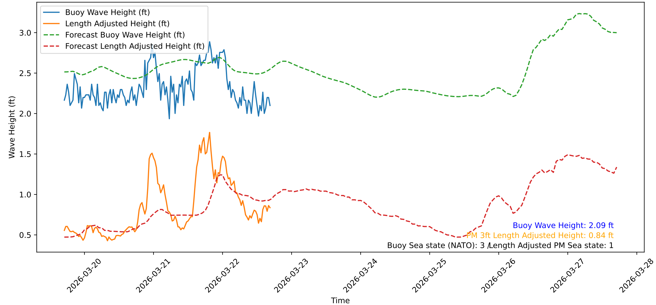
Wave Heights over Time for Green Beach at 2026-03-22 17:11:08
