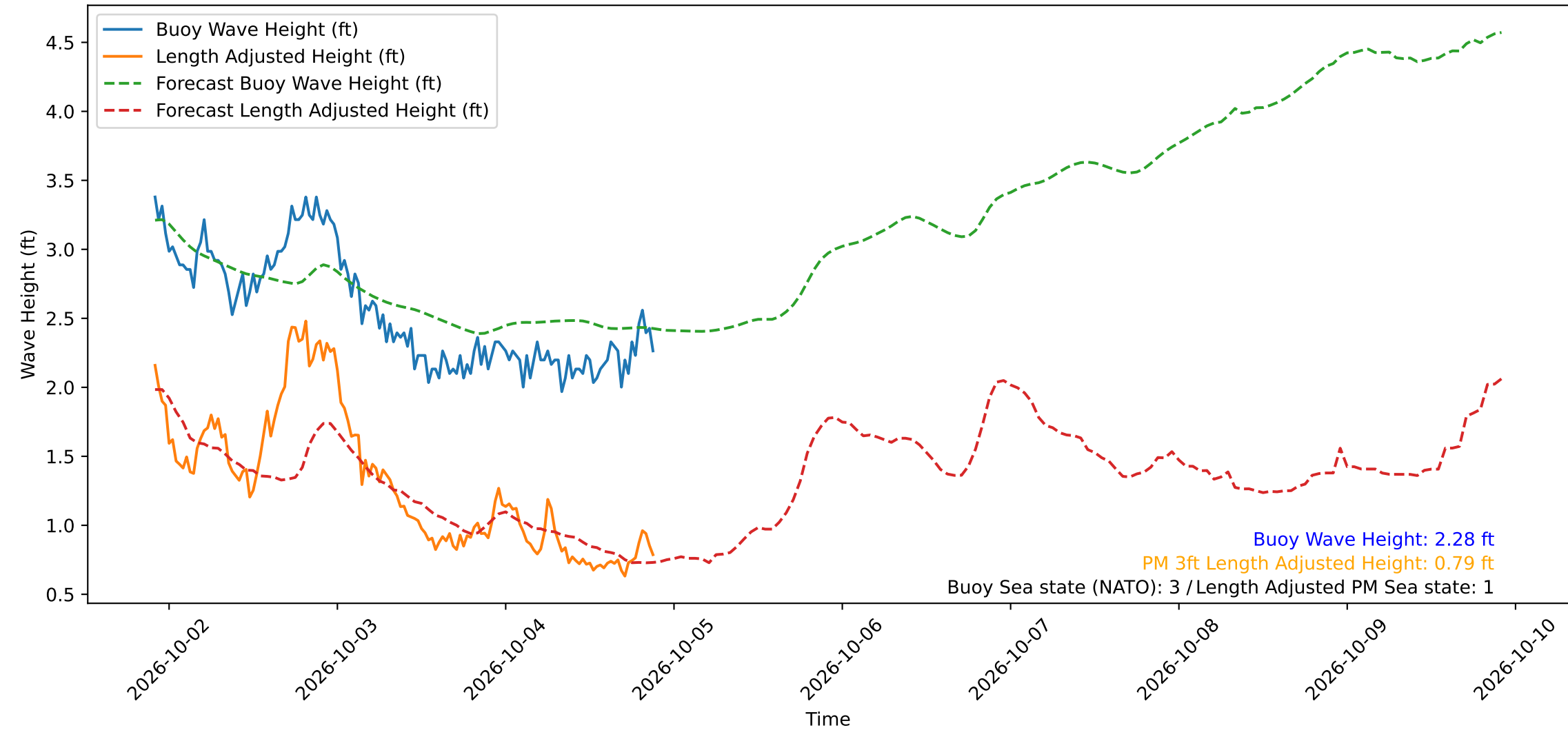
Wave Heights over Time for Green Beach at 2026-10-04 21:51:15
