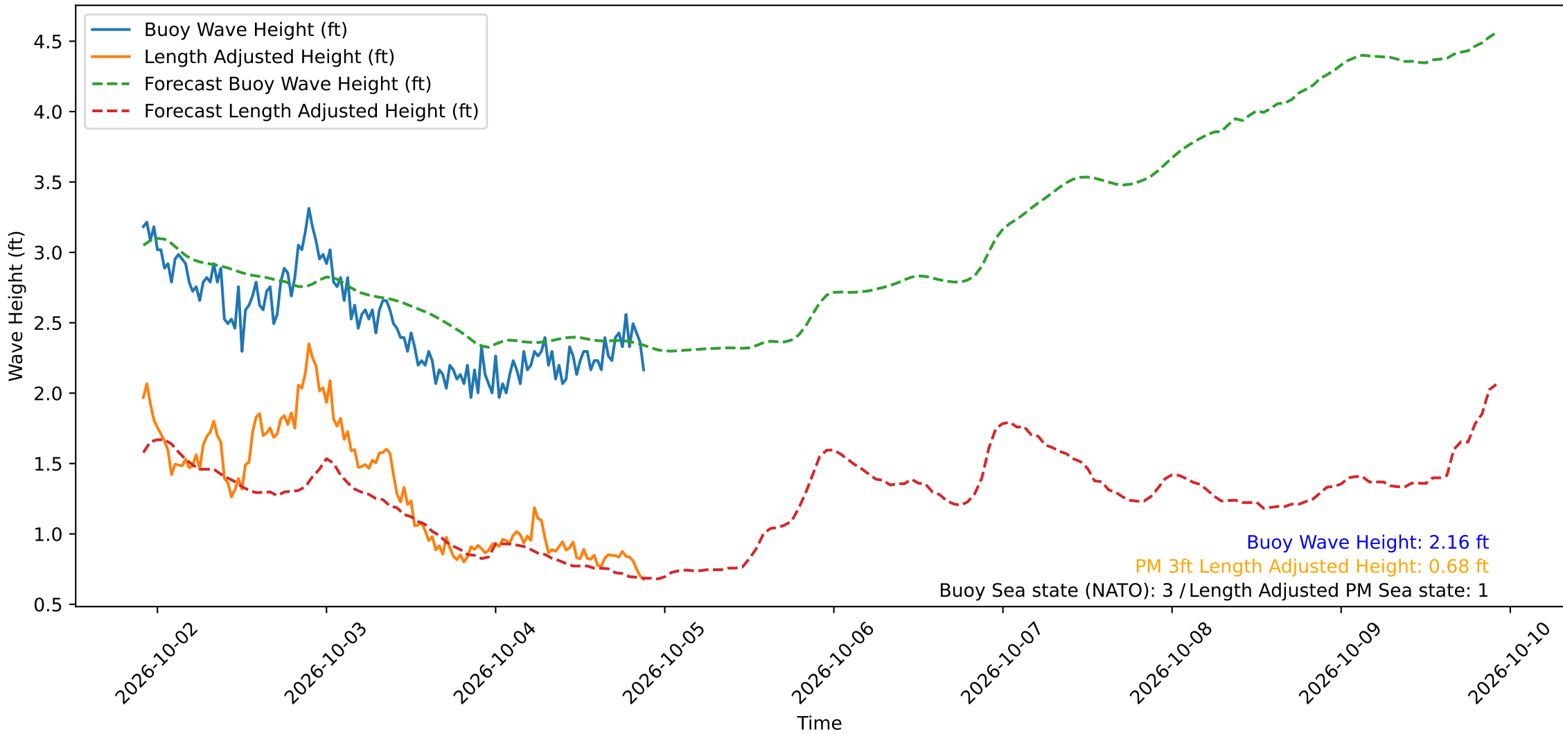
Wave Heights over Time for Oceanside Harbor at 2026-10-04 21:50:30
