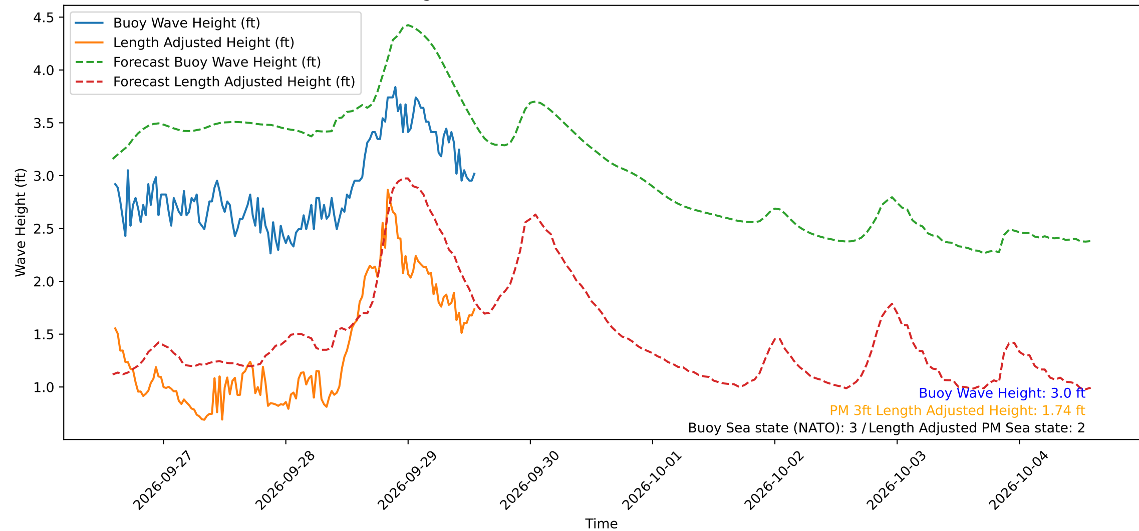
Wave Heights over Time for Red Beach at 2026-09-29 14:00:50
