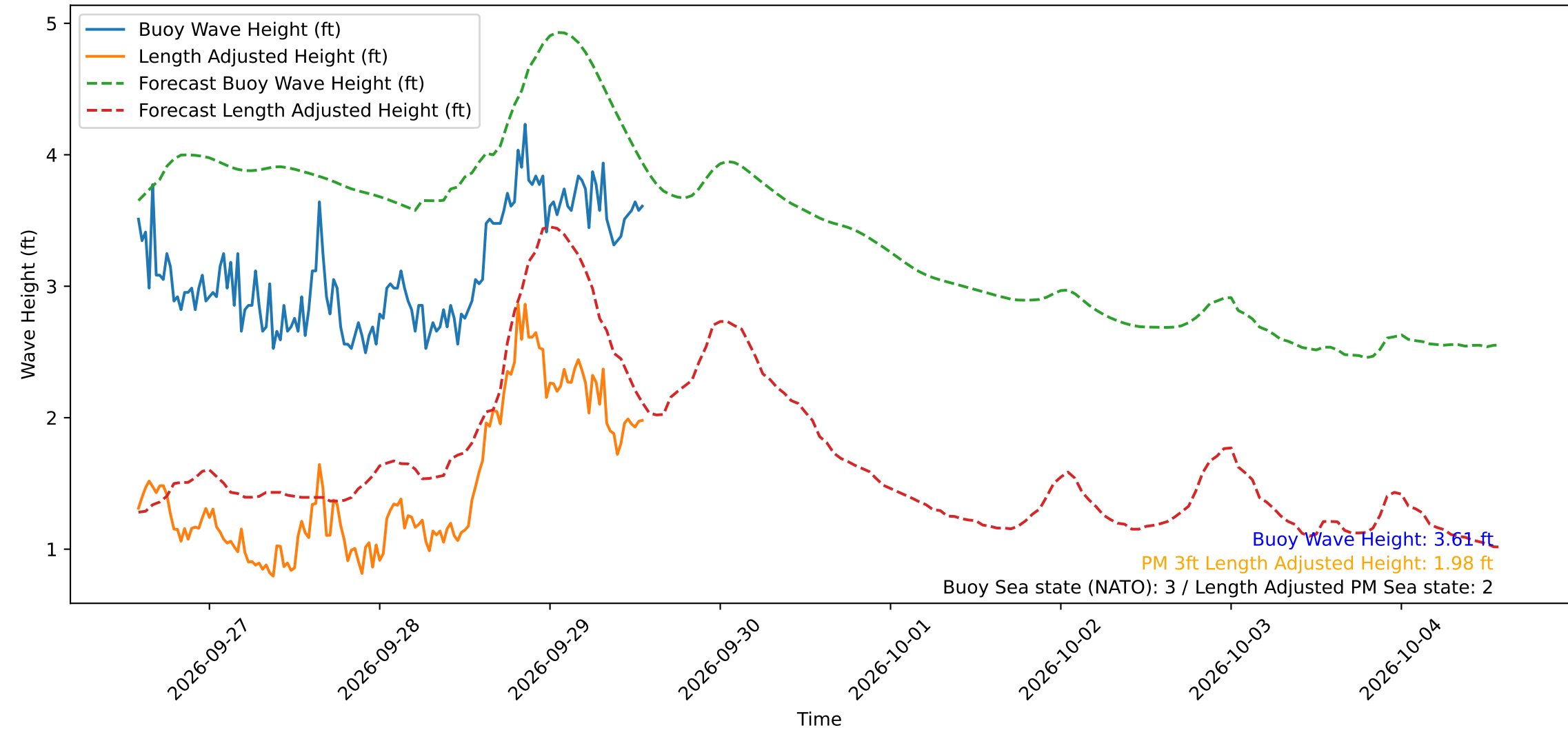
Wave Heights over Time for Oceanside Harbor at 2026-09-29 14:00:30
