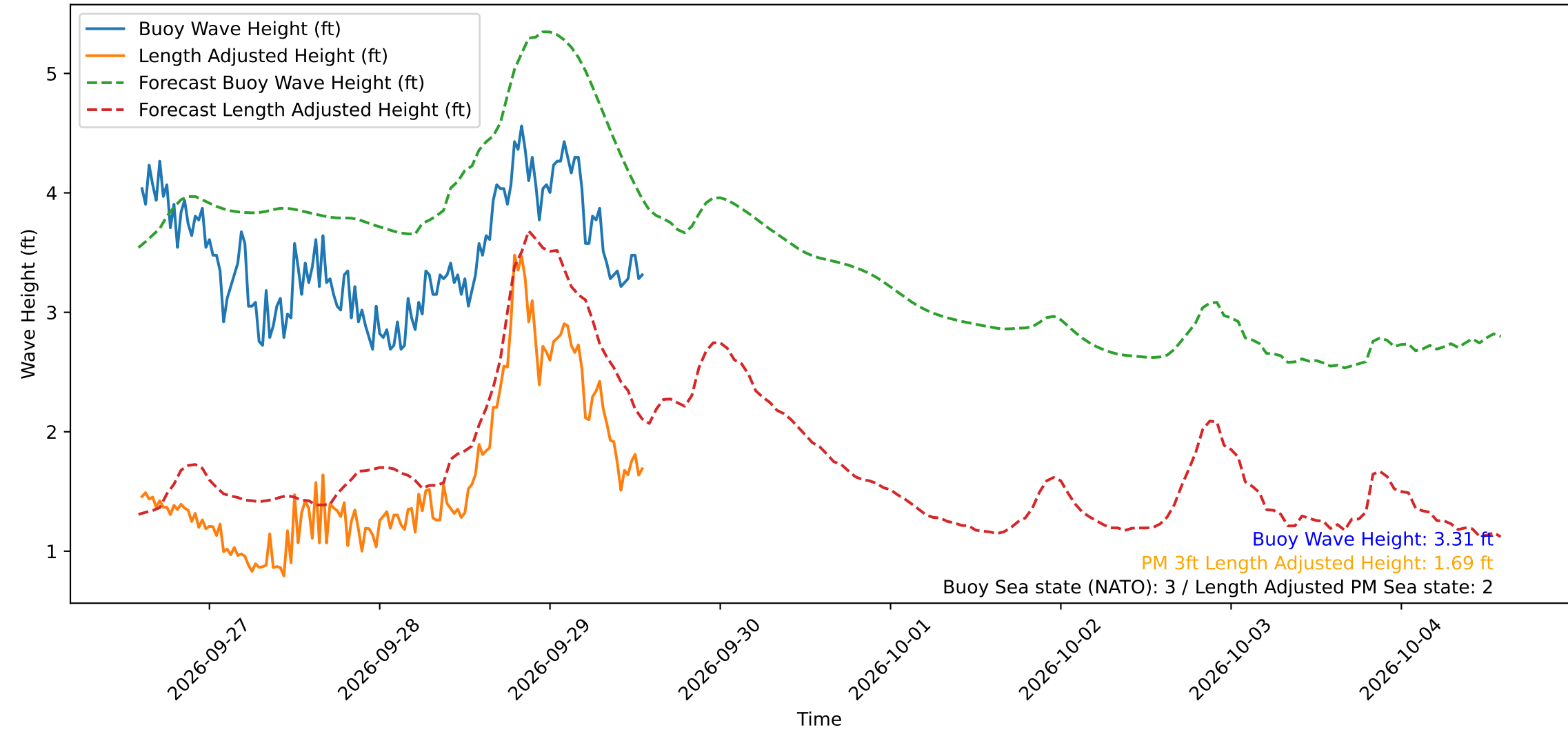
Wave Heights over Time for Green Beach at 2026-09-29 14:01:13
