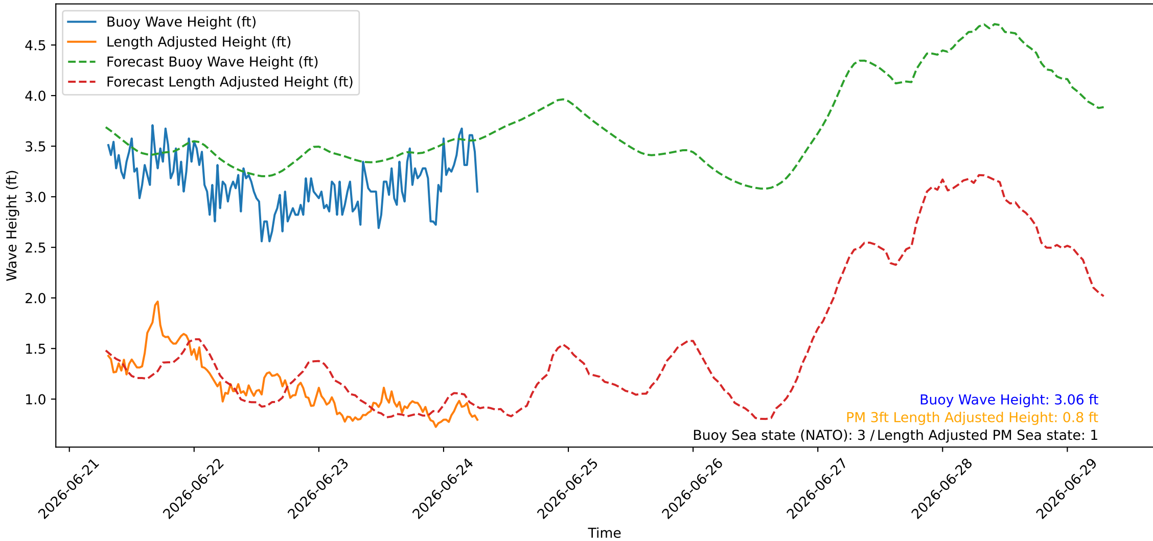
Wave Heights over Time for Oceanside Harbor at 2026-06-24 07:20:26
