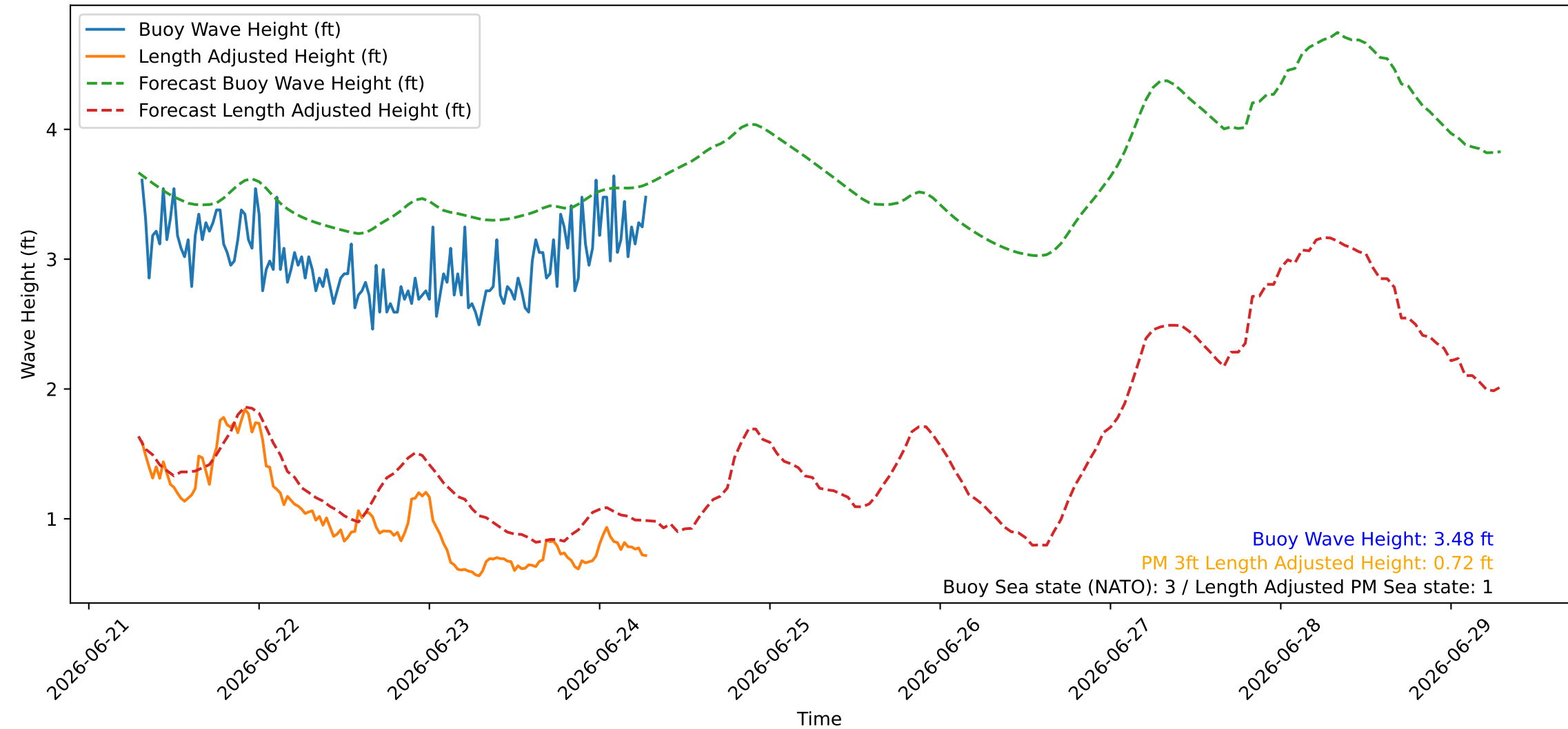
Wave Heights over Time for Green Beach at 2026-06-24 07:21:09
