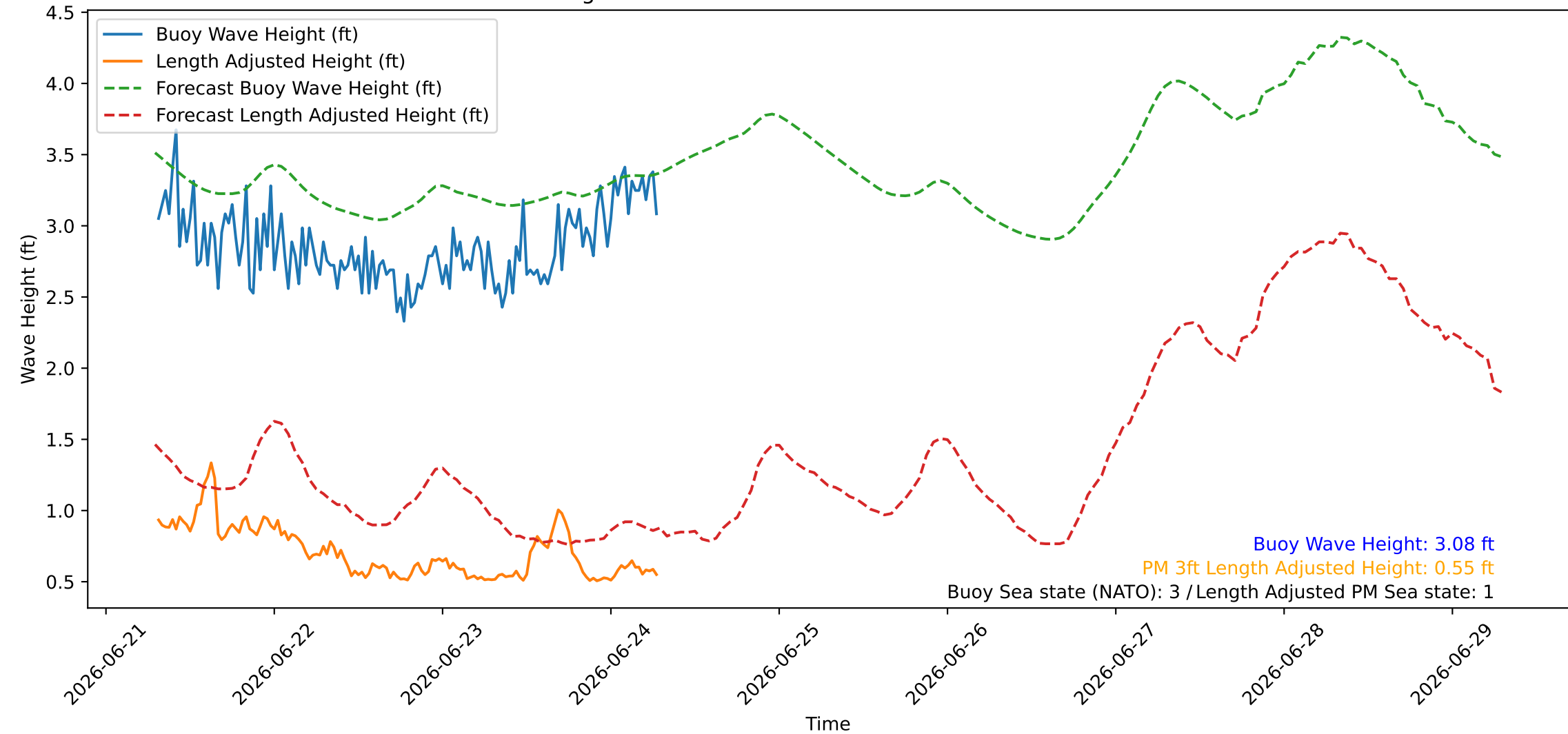
Wave Heights over Time for Red Beach at 2026-06-24 07:20:46
