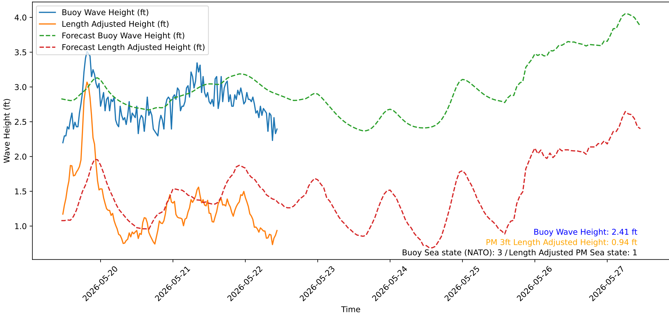
Wave Heights over Time for Red Beach at 2026-05-22 11:20:52
